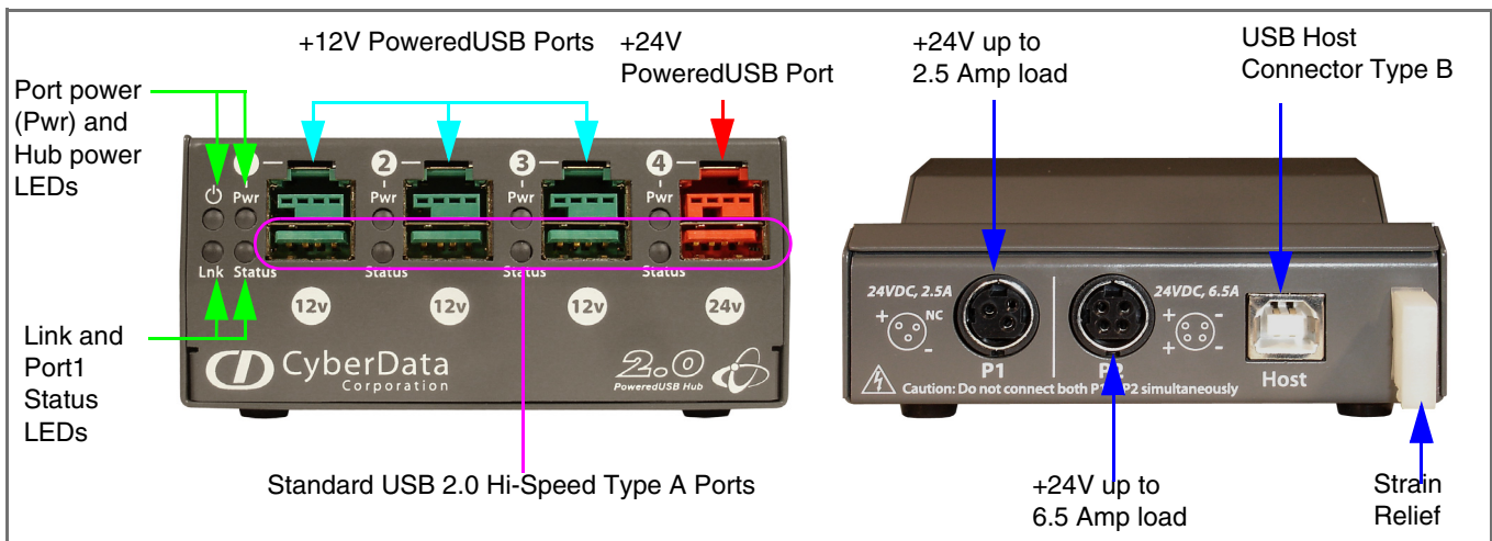
Figure 2: Component identification: external front and back views
