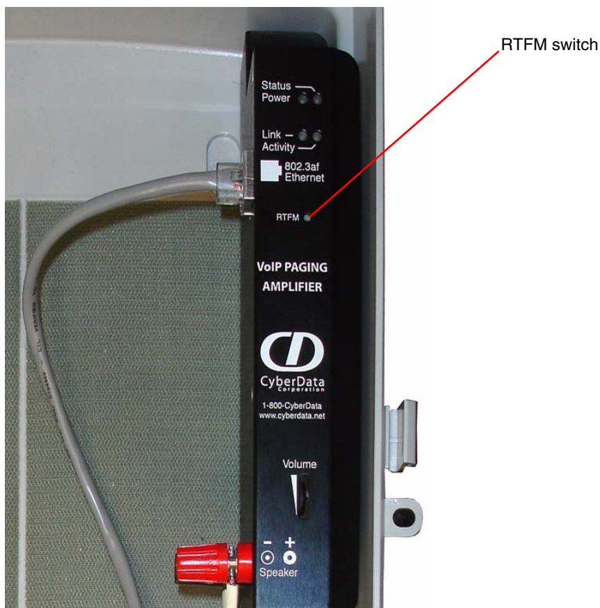
Figure 2-7. RTFM Switch
