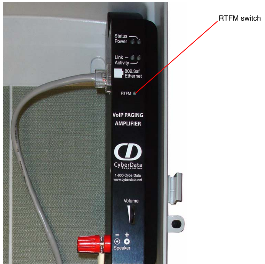
Figure 2-7. RTFM Switch
