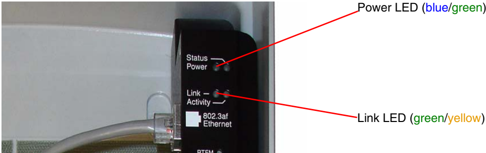
Figure 2-5. Loudspeaker Amplifier LEDs—Power and Link
