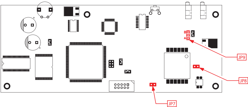
Figure 2-2. Jumper Locations
