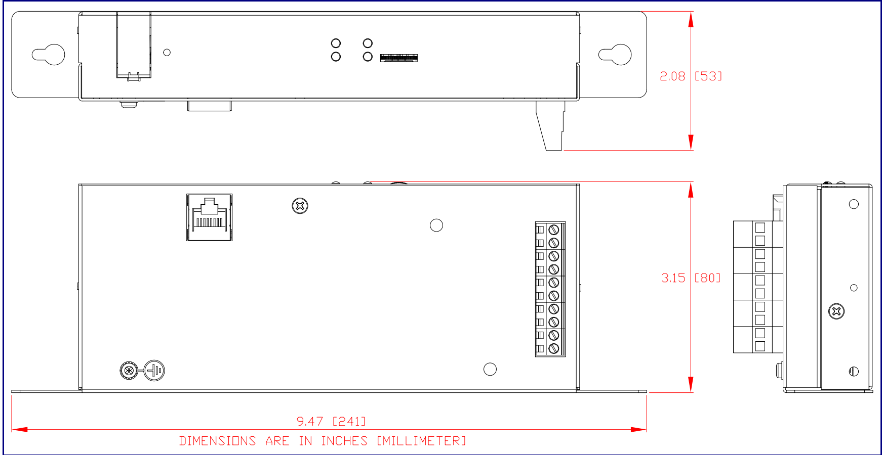
Figure 1-3. Dimensions
