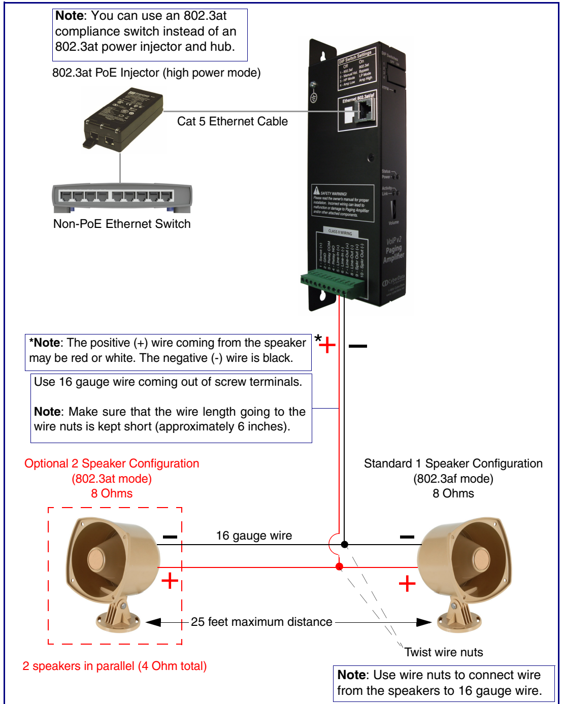
Figure 2-6. Using the Amplified Outputs—High Power Mode
