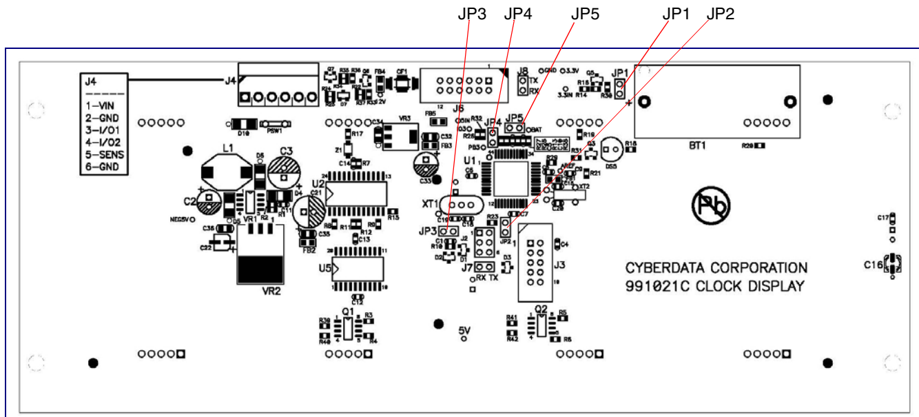
Figure 2-9. Jumper Locations
