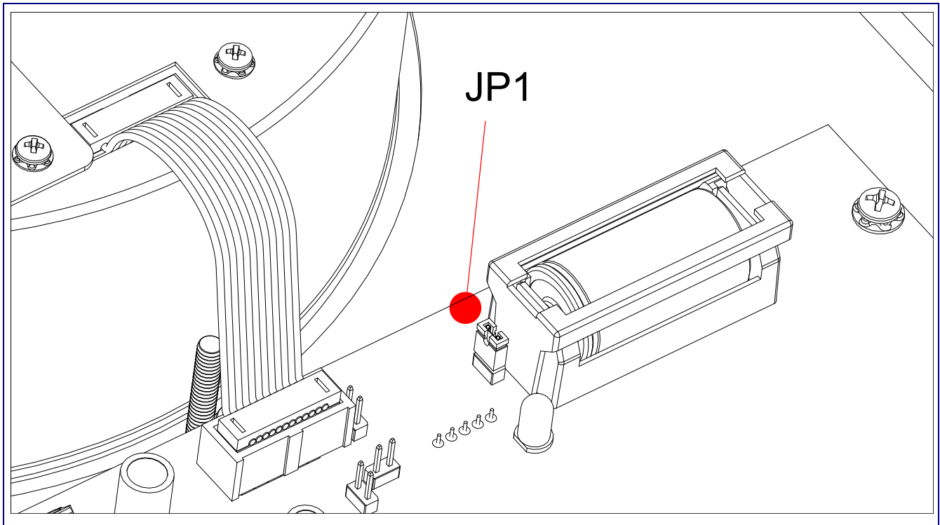
Figure 2-11. Jumper JP1
