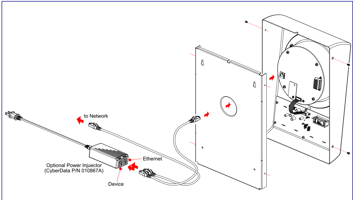
Figure 2-8. Connecting Power—Optional Power Injector
