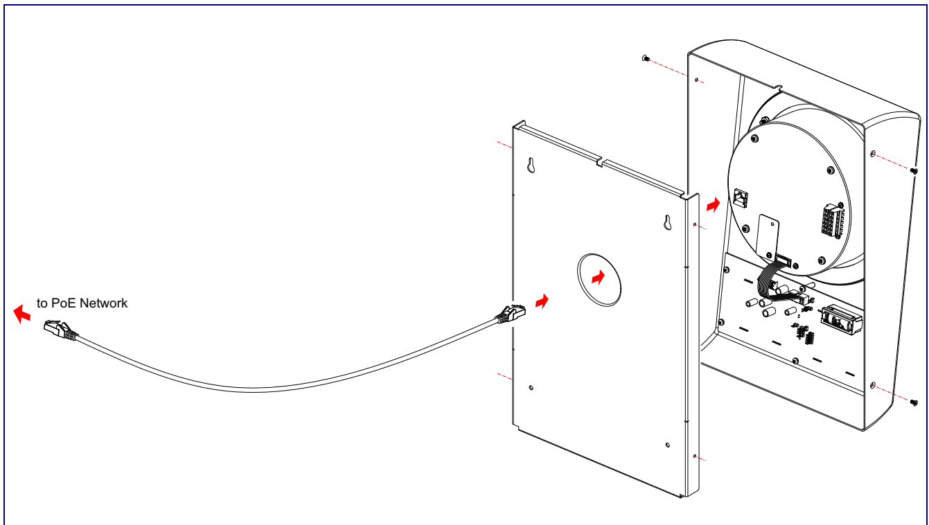
Figure 2-7. Connecting Power—PoE
