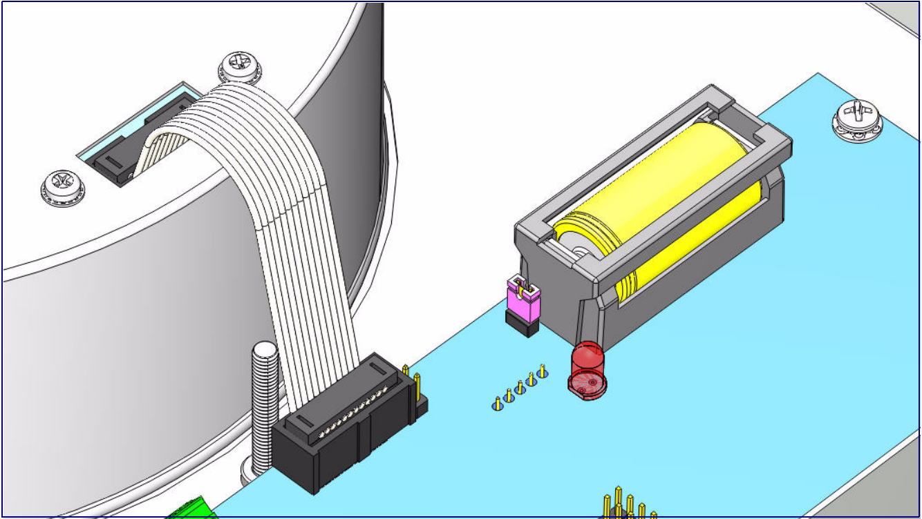
Figure 2-12. Clock Kit Battery Location
