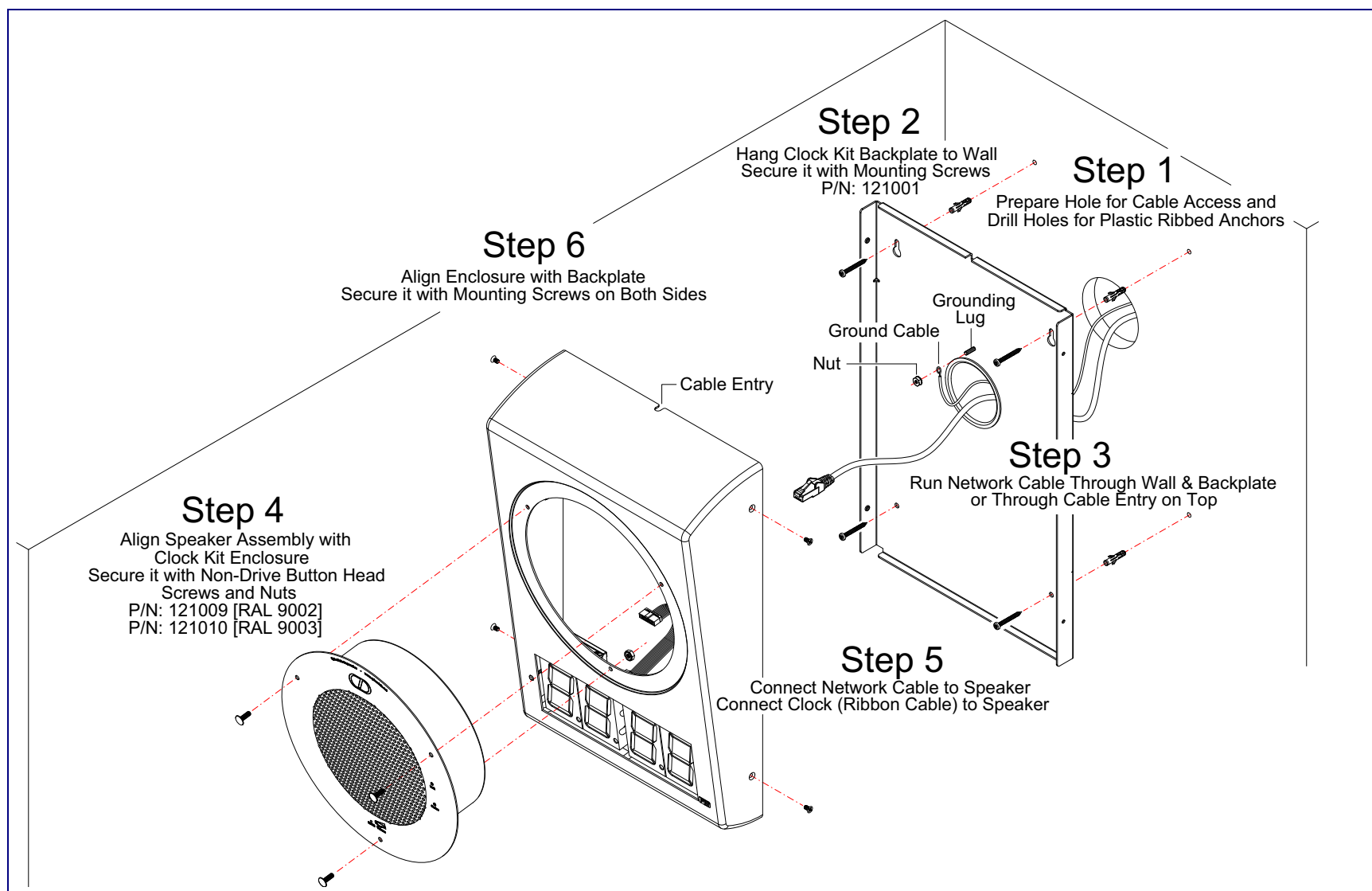
Figure 2-14. Clock Kit Wall Mount Adapter Installation
