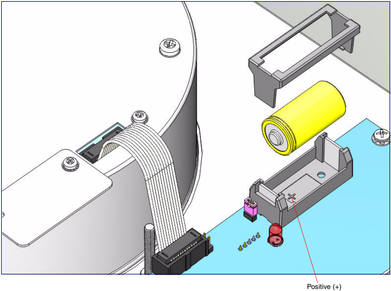
Figure 2-13. Clock Kit Battery Replacement
