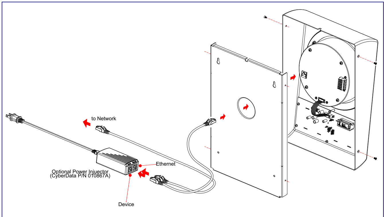
Figure 2-10. Connecting Power
