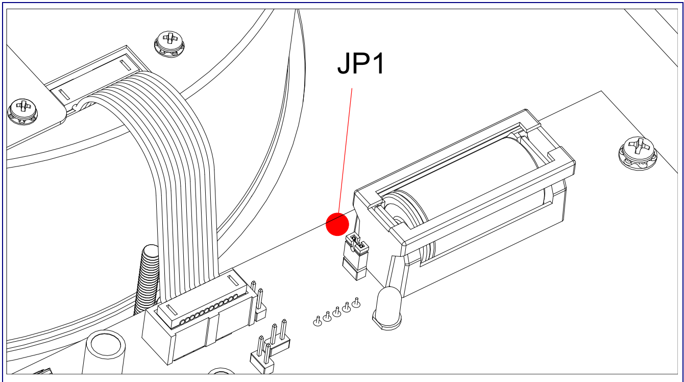
Figure 2-5. Jumper JP1
