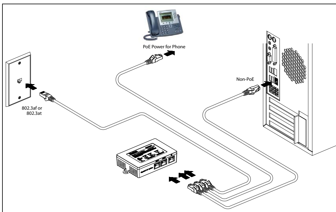
Figure C-1. Typical Installation
