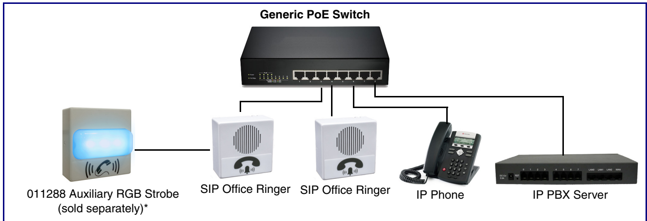
Figure 1-2. Typical Installation
