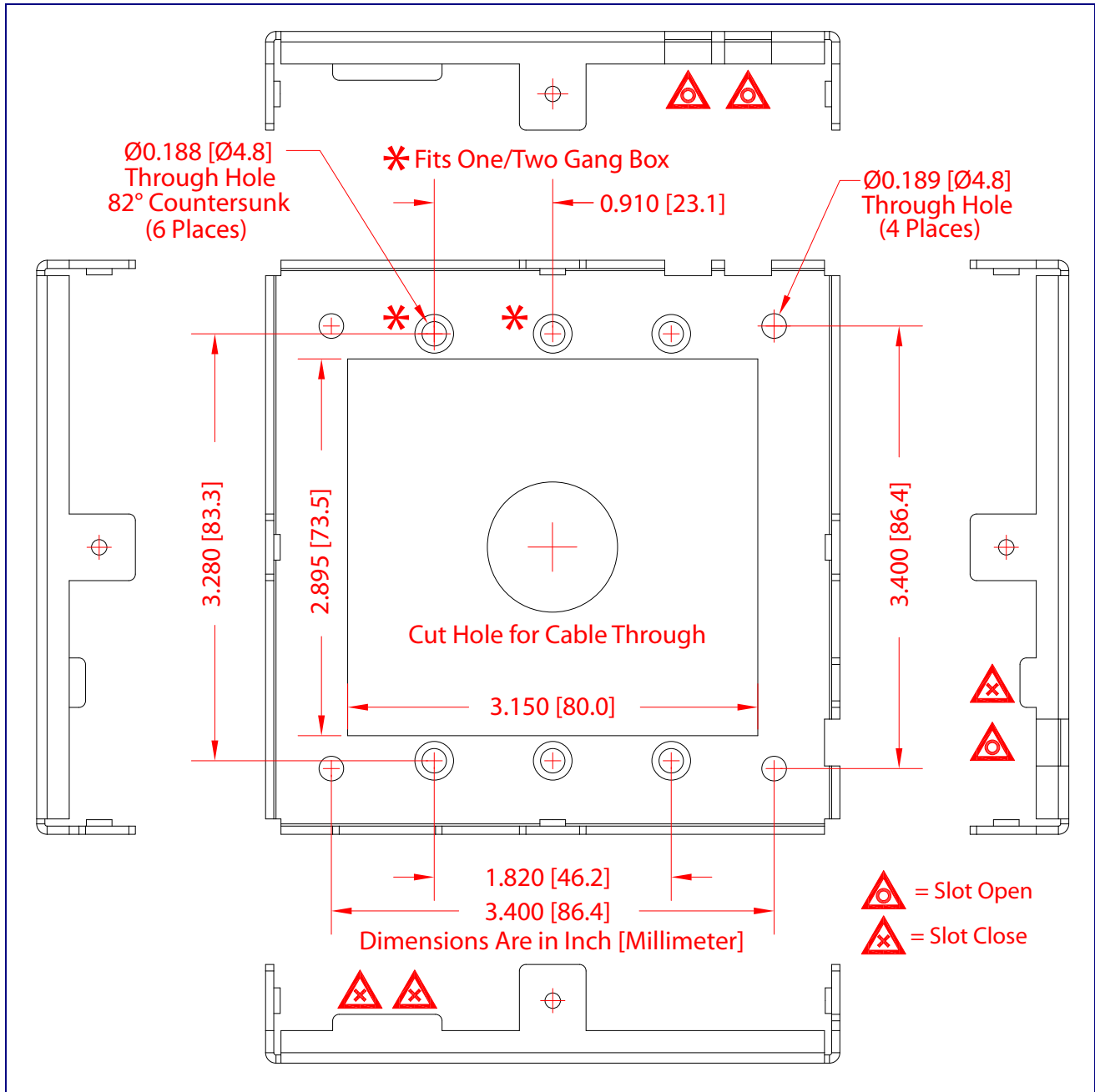
Figure A-3. Dimensions for Backplate and Cable Through-Holes
