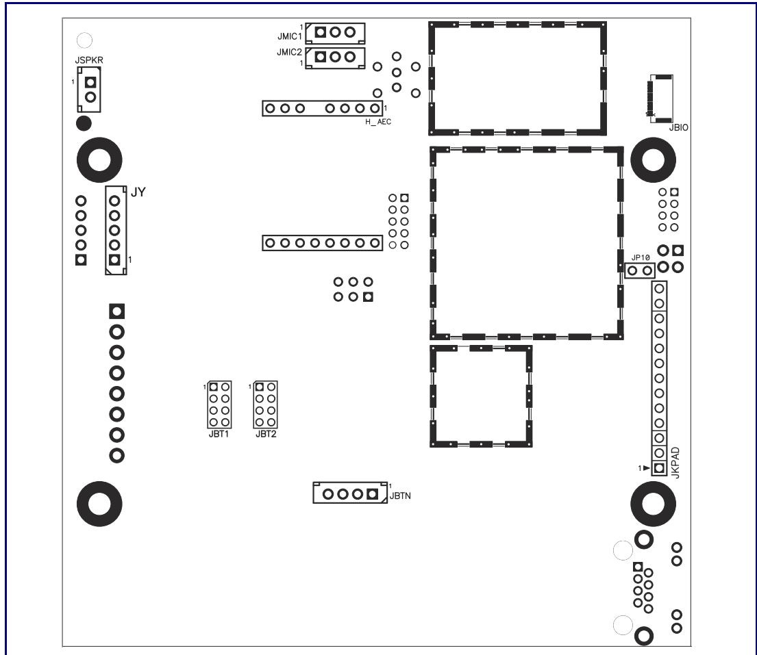
Figure 2-16. Connector Locations
