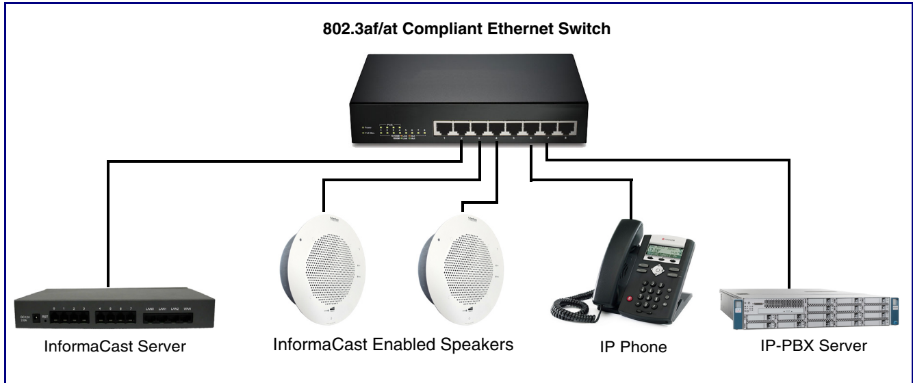
Figure 1-2. Typical Installation
