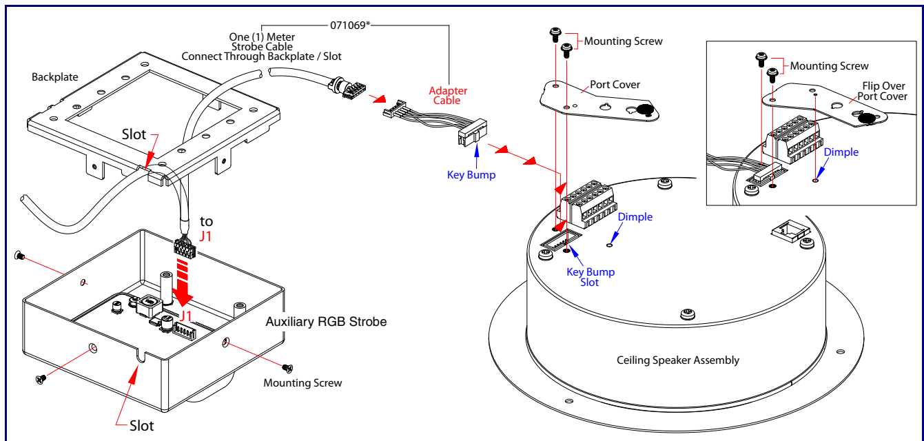
Figure 2-4. Connecting the Auxiliary RGB Strobe Kit to the InformaCast Enabled Speaker
