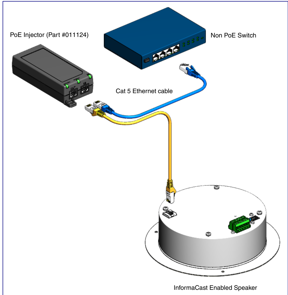
Figure 2-2. InformaCast Enabled Speaker (with PoE Injector) to a Non PoE Switch
