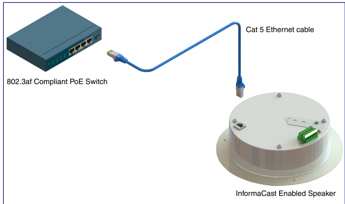
Figure 2-1. InformaCast Enabled Speaker to a 802.3af Compliant PoE Switch
