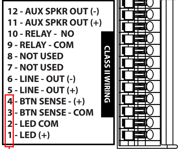
Figure 1-3. Optional Connections
