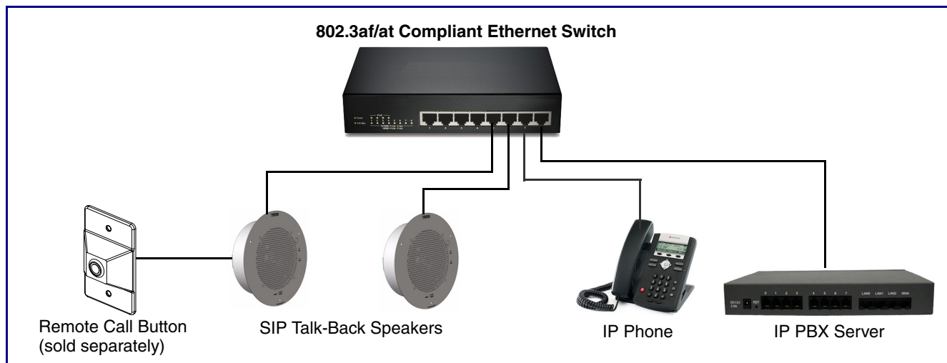
Figure 1-2. Typical Installation
