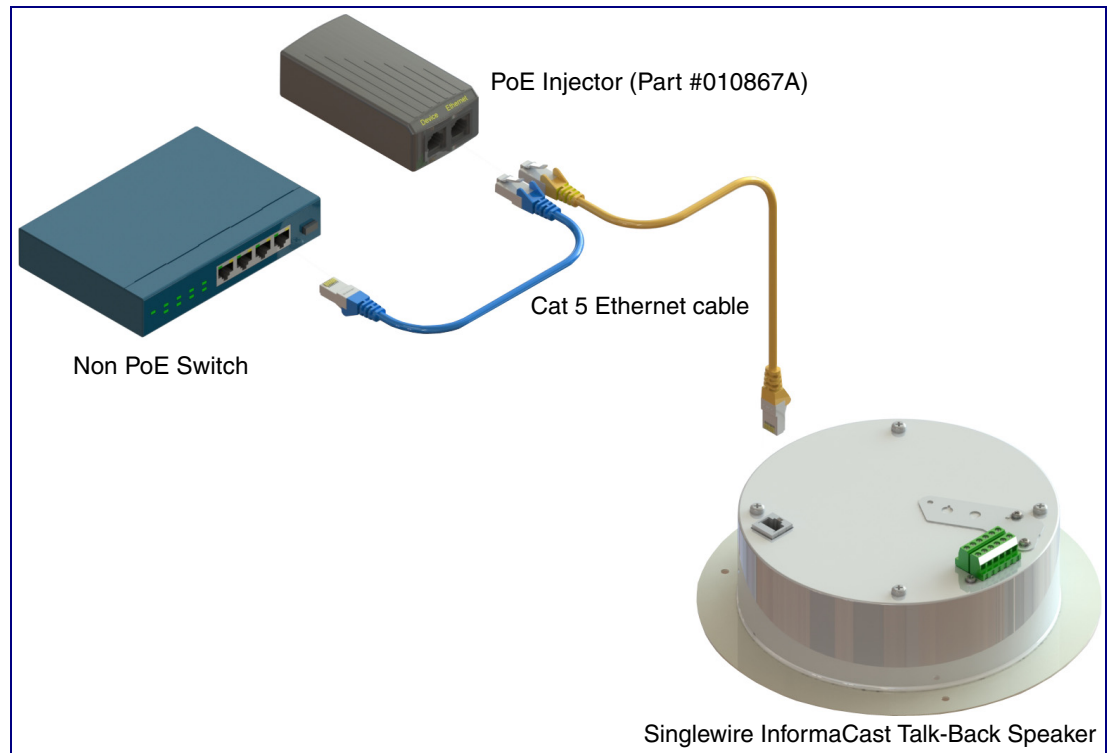
Figure 2-3. Singlewire InformaCast Speaker (with PoE Injector) to a Non PoE Switch
