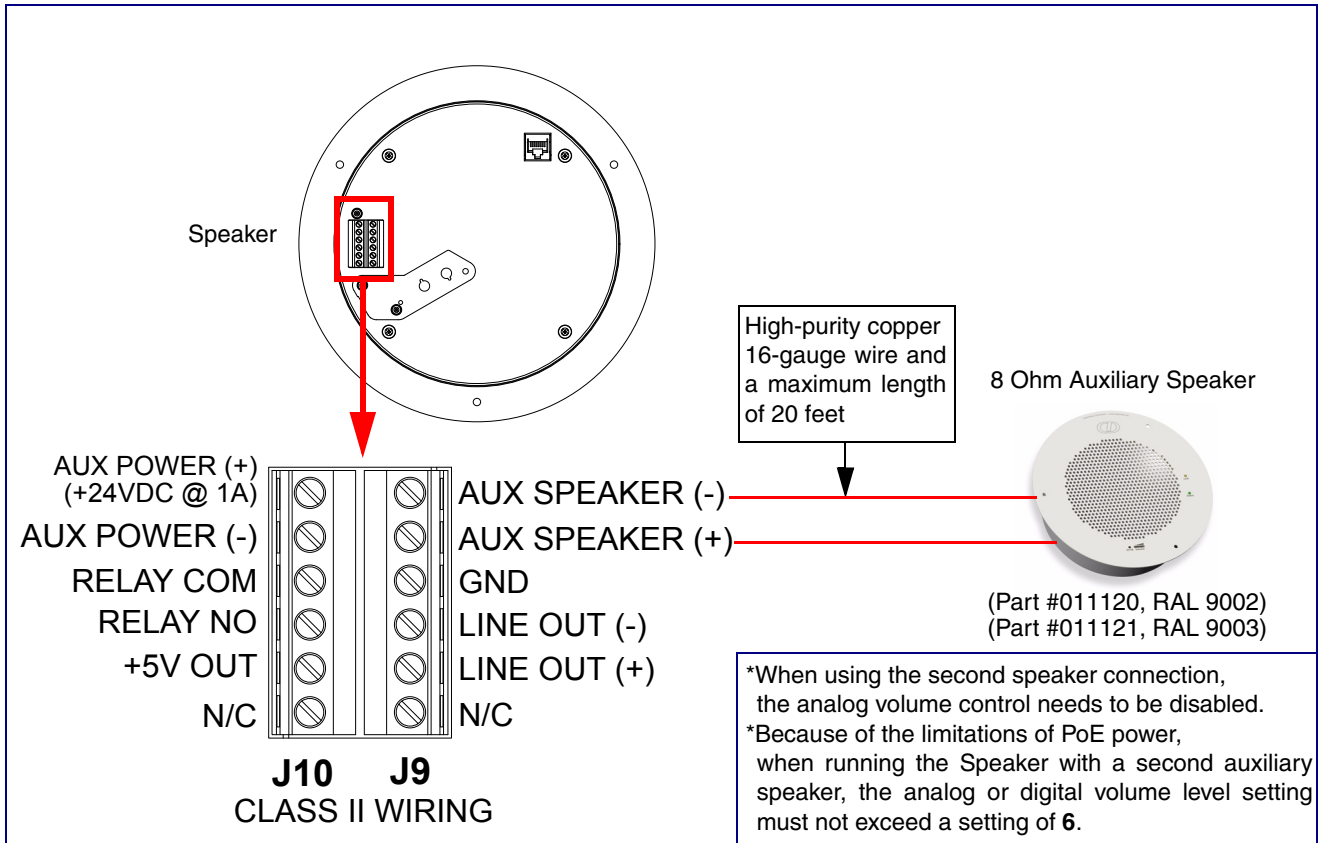
Figure 2-7. Singlewire InformaCast Speaker with Auxiliary Speaker Connection
