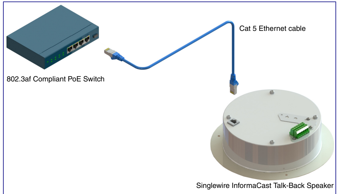
Figure 2-2. Singlewire InformaCast Speaker to a 802.3af Compliant PoE Switch
