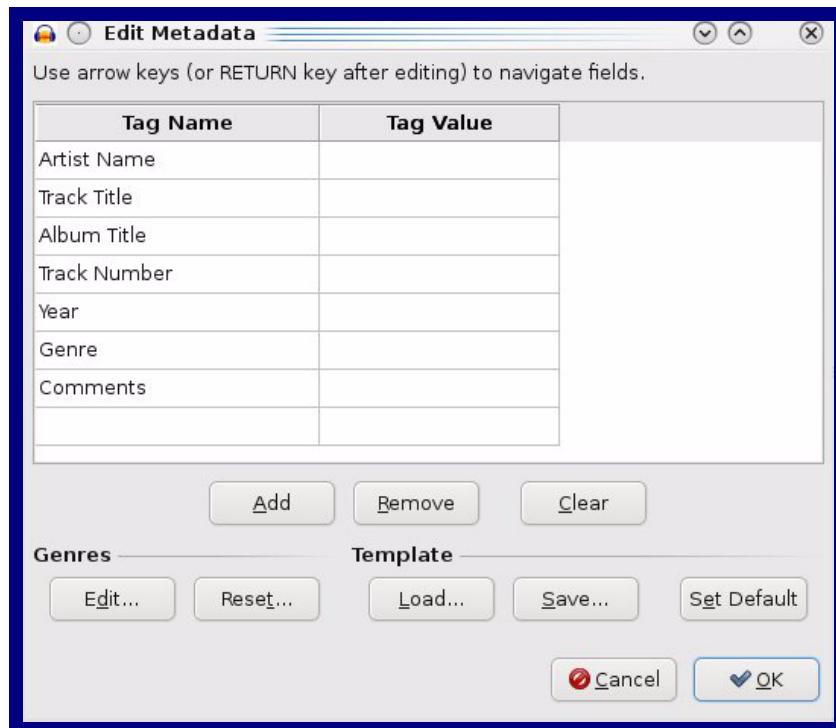
Figure 2-42. Audacity 2
