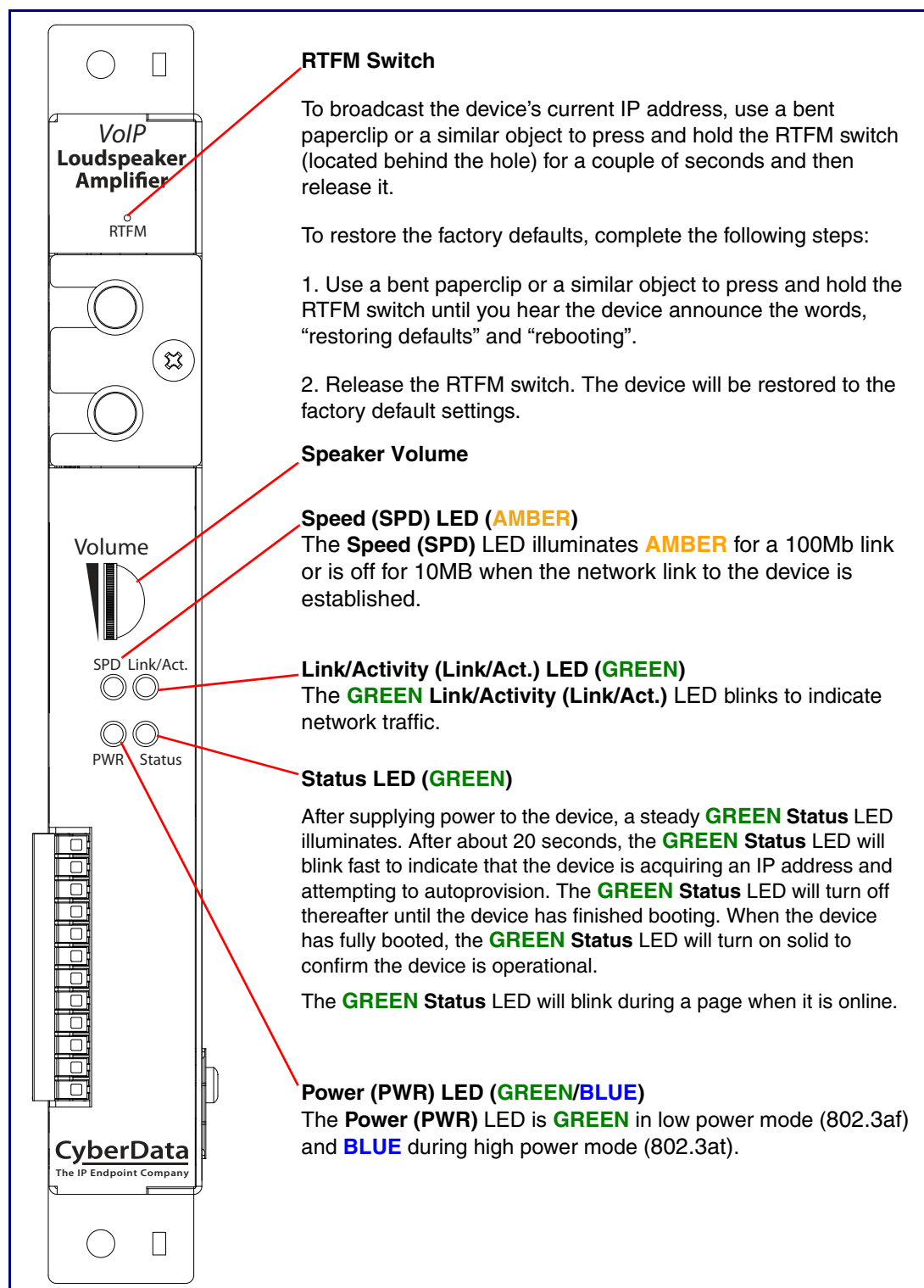
Figure 2-5. InformaCast Enabled Paging Amplifier Components
