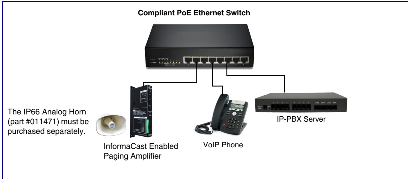
Figure 1-2. Typical Installation
