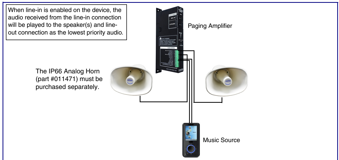
Figure 2-10. Line-In Connection
