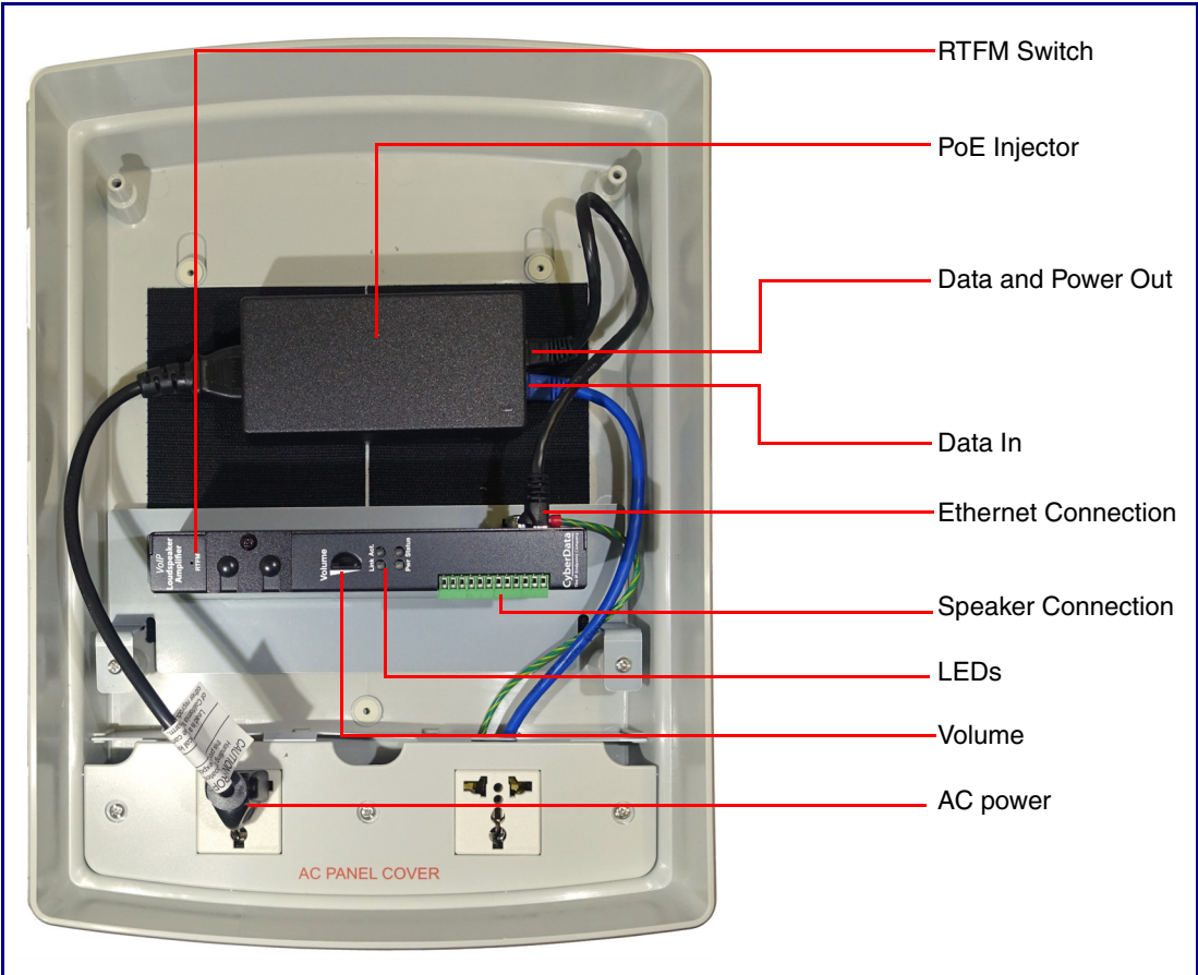
Figure 2-2. Loudspeaker Amplifier Components—AC powered
