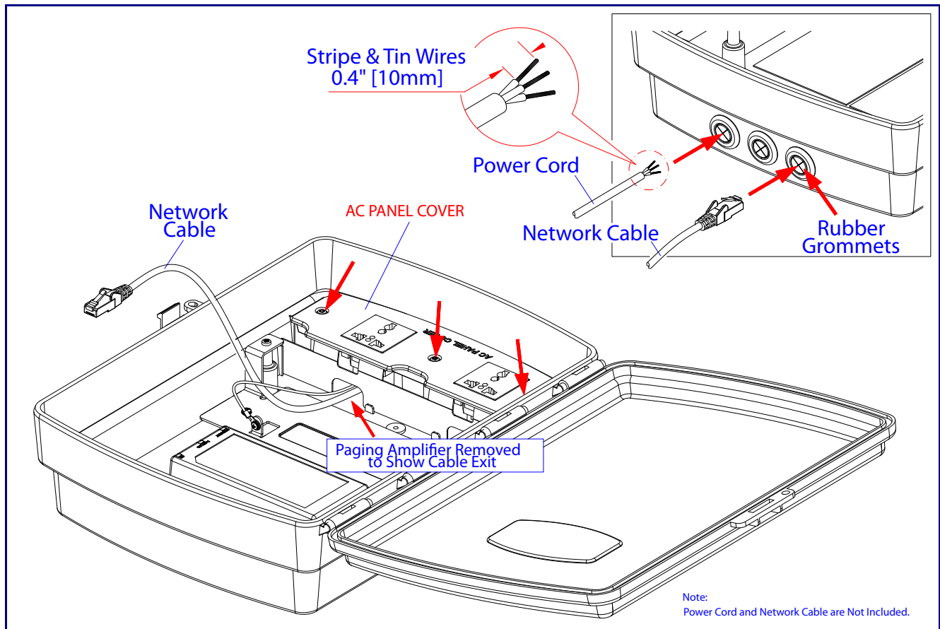
Figure 2-10. Connecting the Strobe
