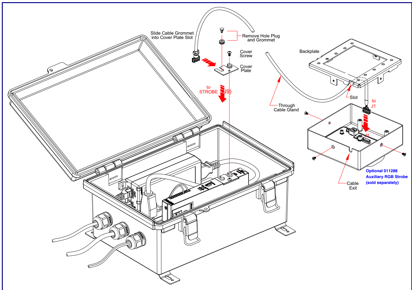
Figure 2-22. Connecting the Optional 011288 Auxiliary RGB Strobe
