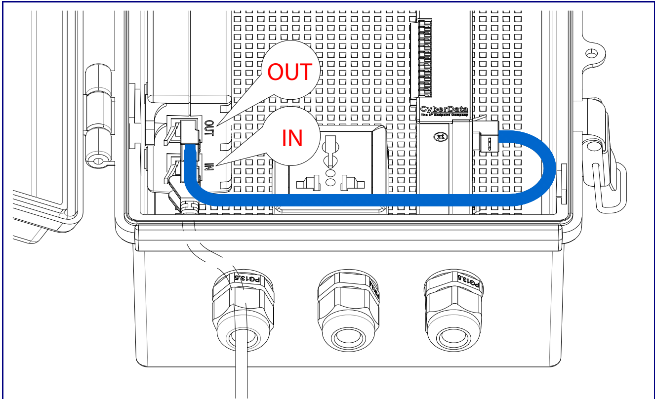
Figure 2-14. Connecting the SIP Loudspeaker Amplifier (AC-Powered) to the Power Injector
