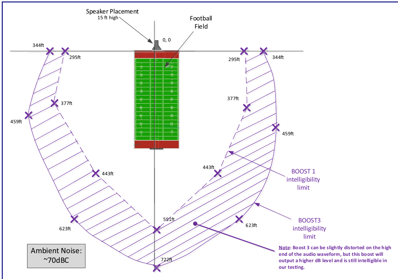
Figure 2-25. Intelligibility Outdoor Field Test
