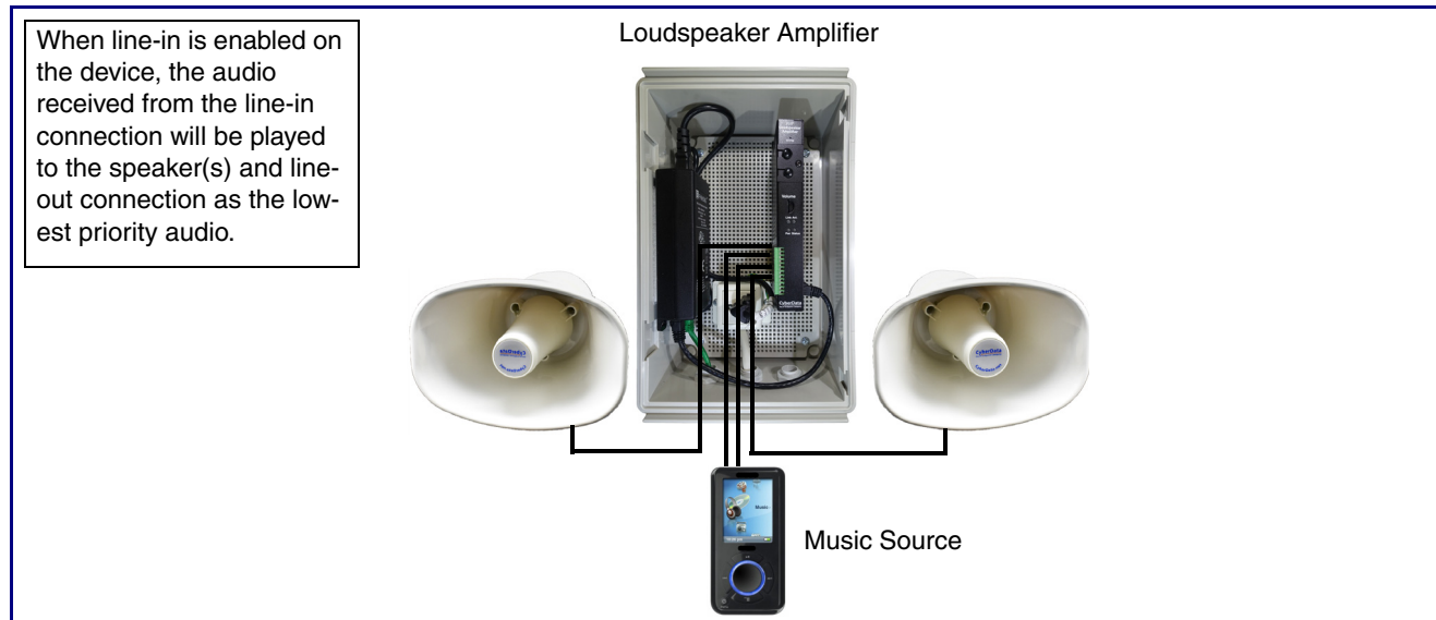
Figure 2-18. Line-In Connection
