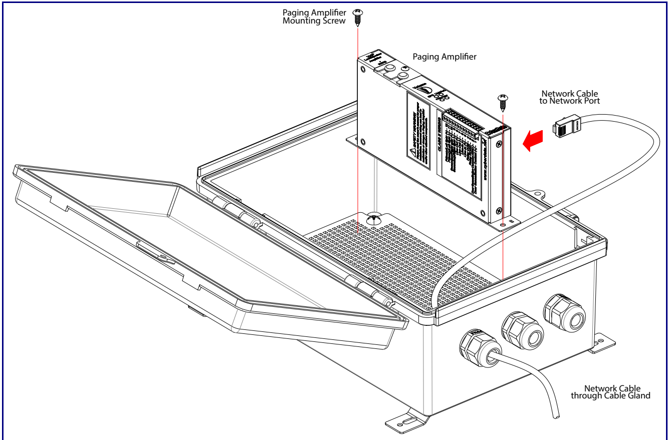
Figure 2-8. Installing the SIP Loudspeaker Amplifier (AC-Powered)
