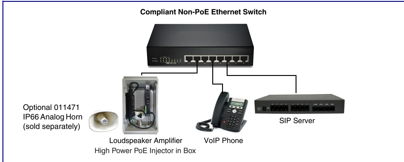
Figure 1-2. Typical Installation
