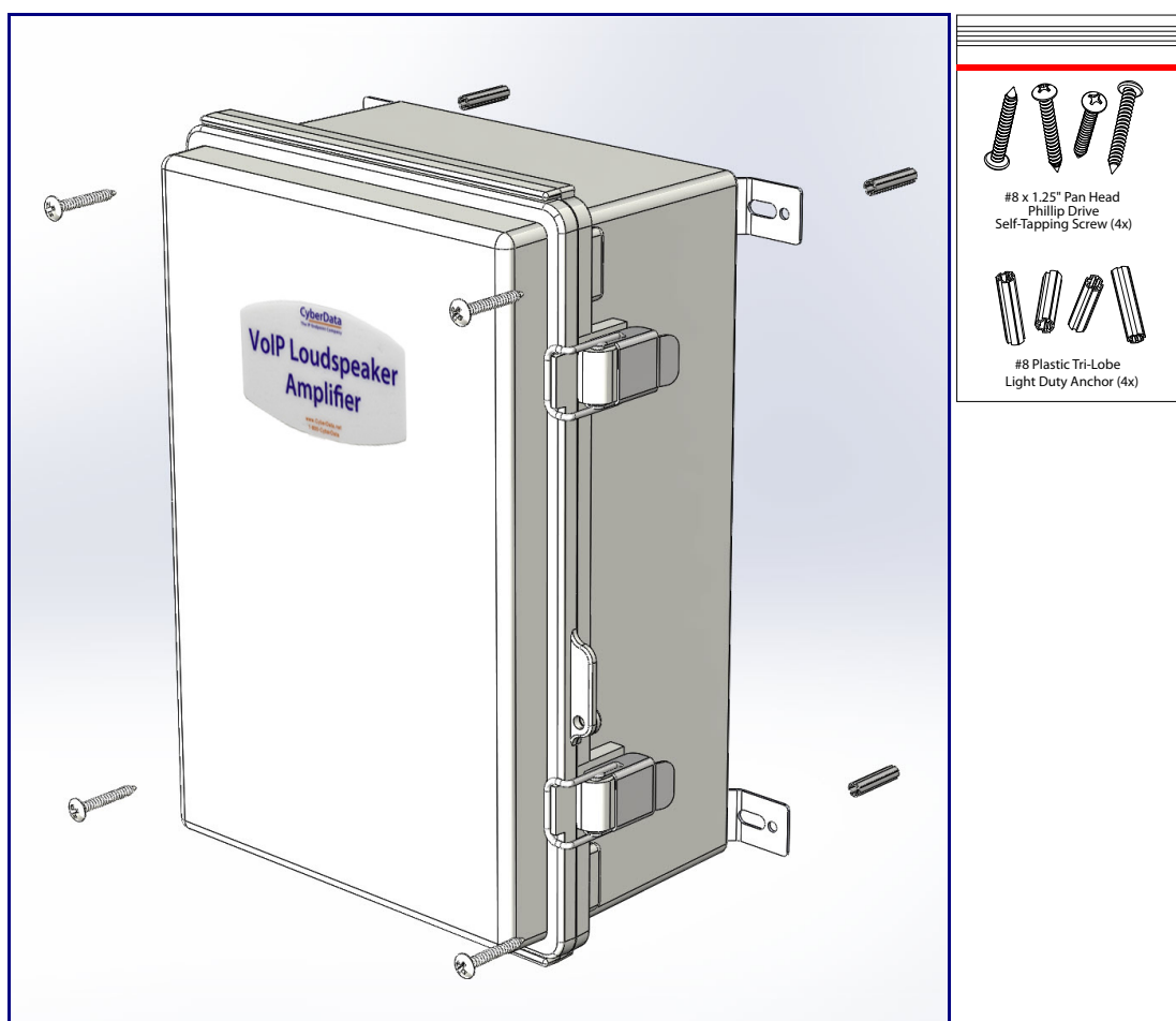
Figure A-1. Mounting the Enclosure
