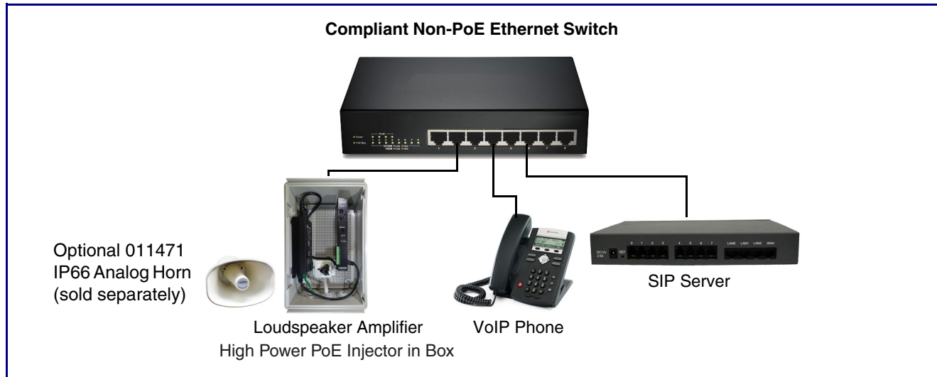
Figure 1-2. Typical Installation
