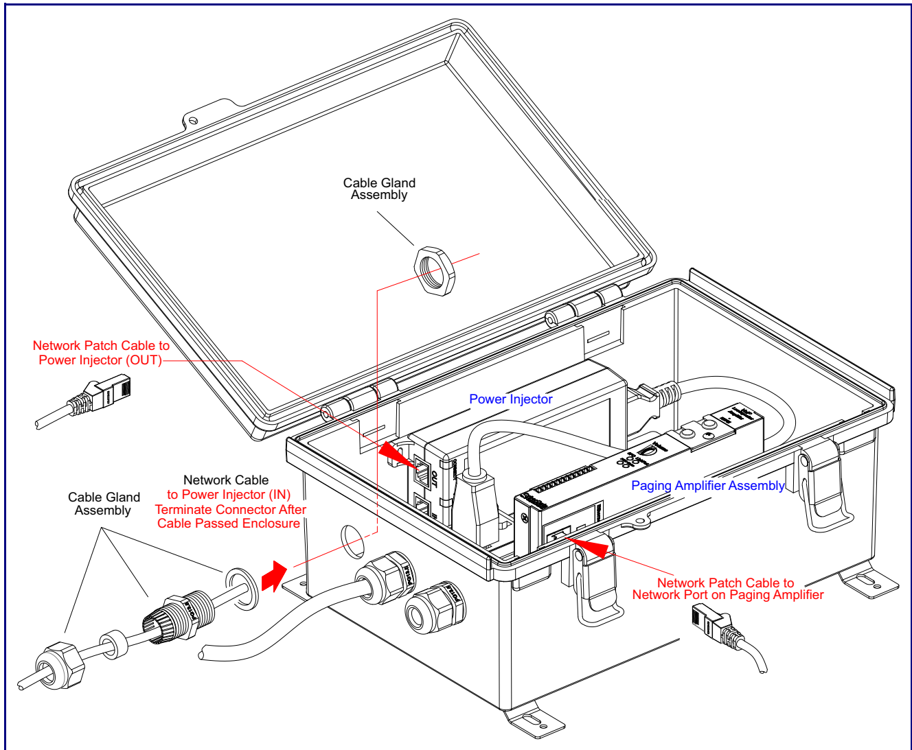
Figure 2-13. Connecting the Network Cable Connector
