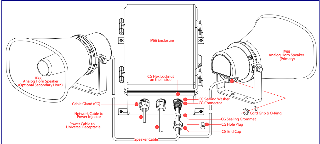
Figure 2-26. IP66 Weatherproofing
