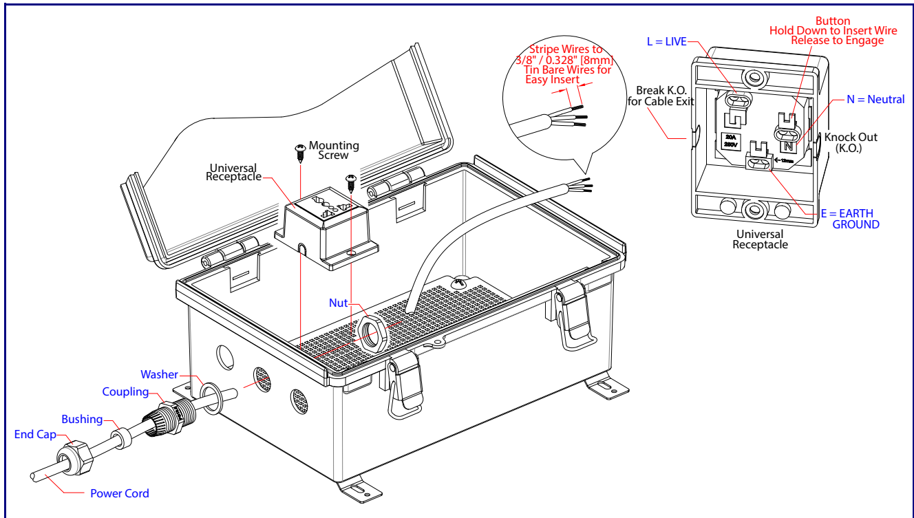
Figure 2-9. Installing the Universal Receptacle
