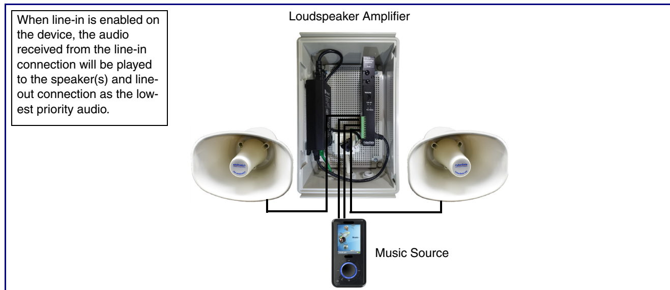
Figure 2-18. Line-In Connection
