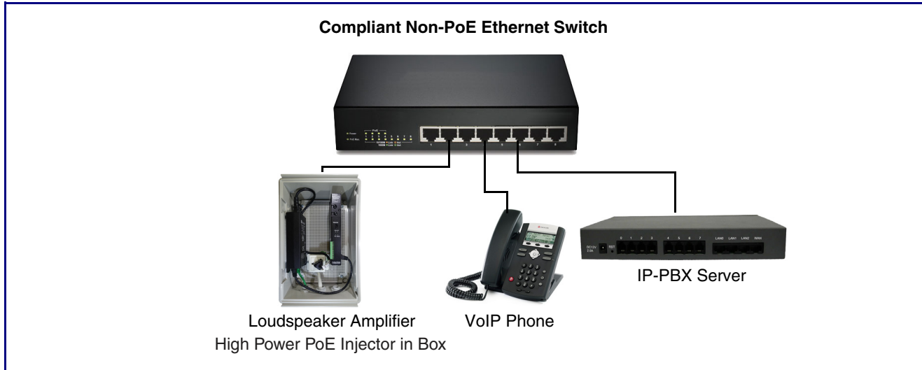
Figure 1-2. Typical Installation
