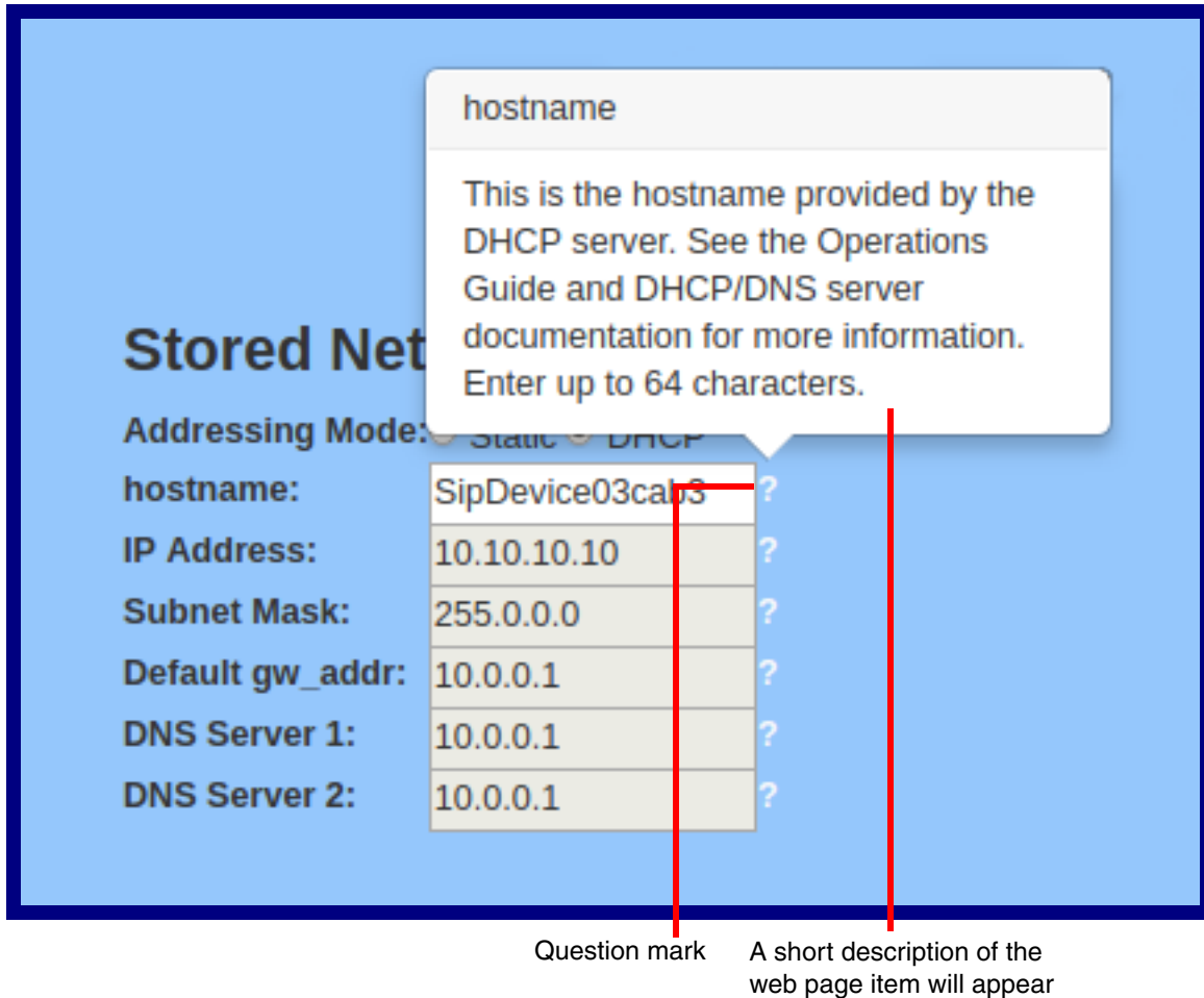
Figure 2-33. Short Description Provided by the Help Feature
