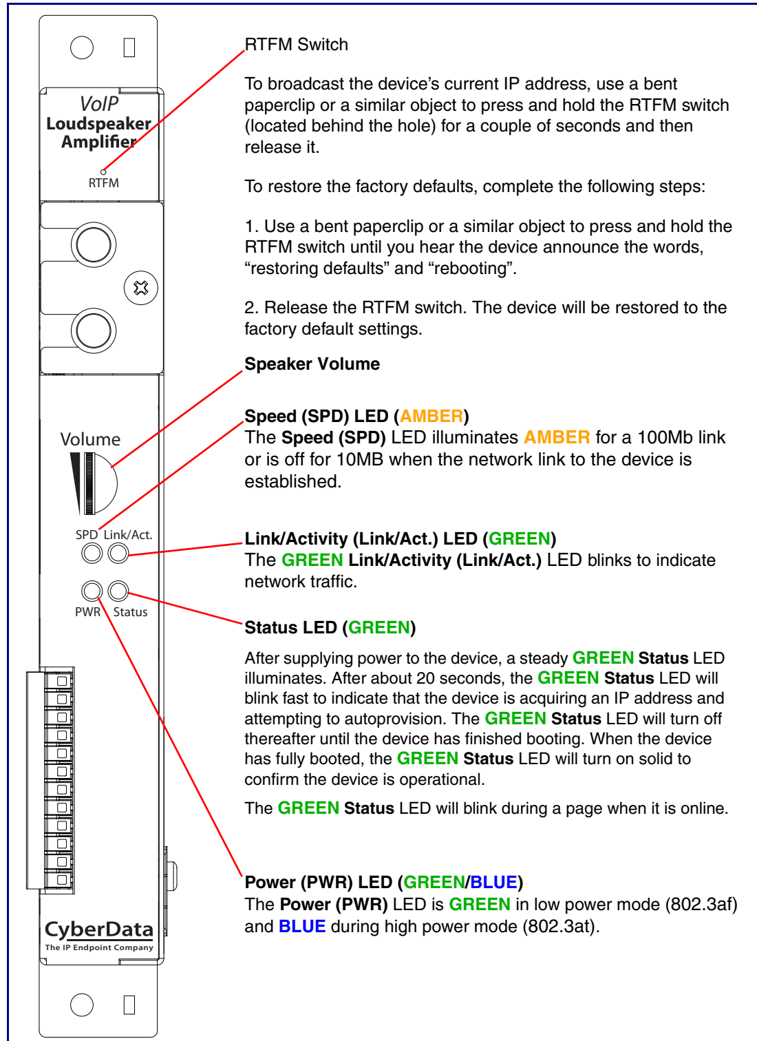
Figure 2-1. SIP Loudspeaker Amplifier (PoE) Components
