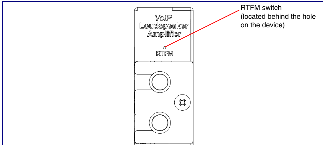
Figure 2-21. RTFM Switch
