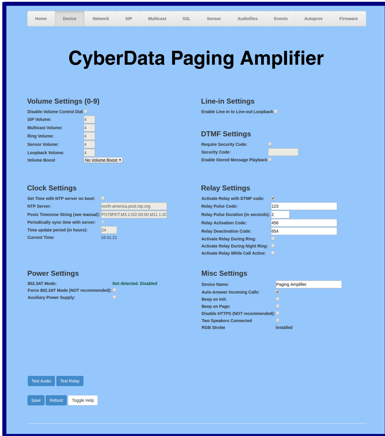
Figure 2-28. Device Page
