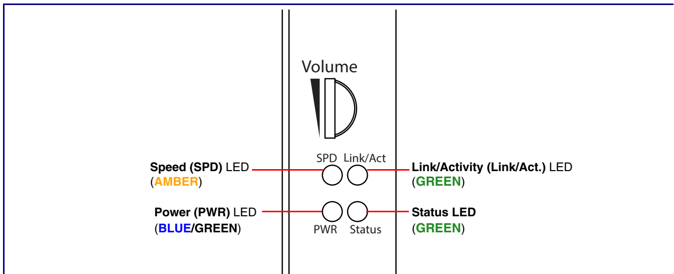
Figure 2-20. SIP Loudspeaker Amplifier (PoE) LEDs
