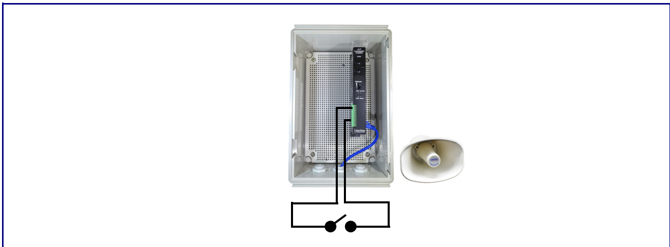
Figure 2-12. Sensor Connection
