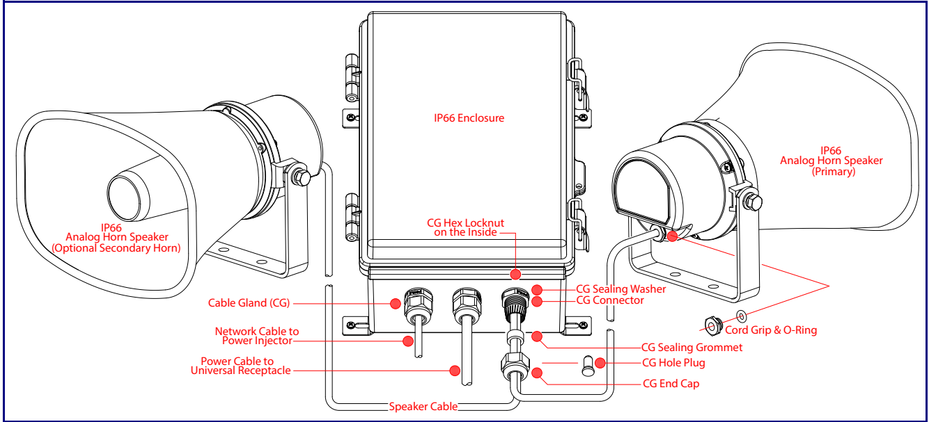
Figure 2-19. IP66 Weatherproofing
