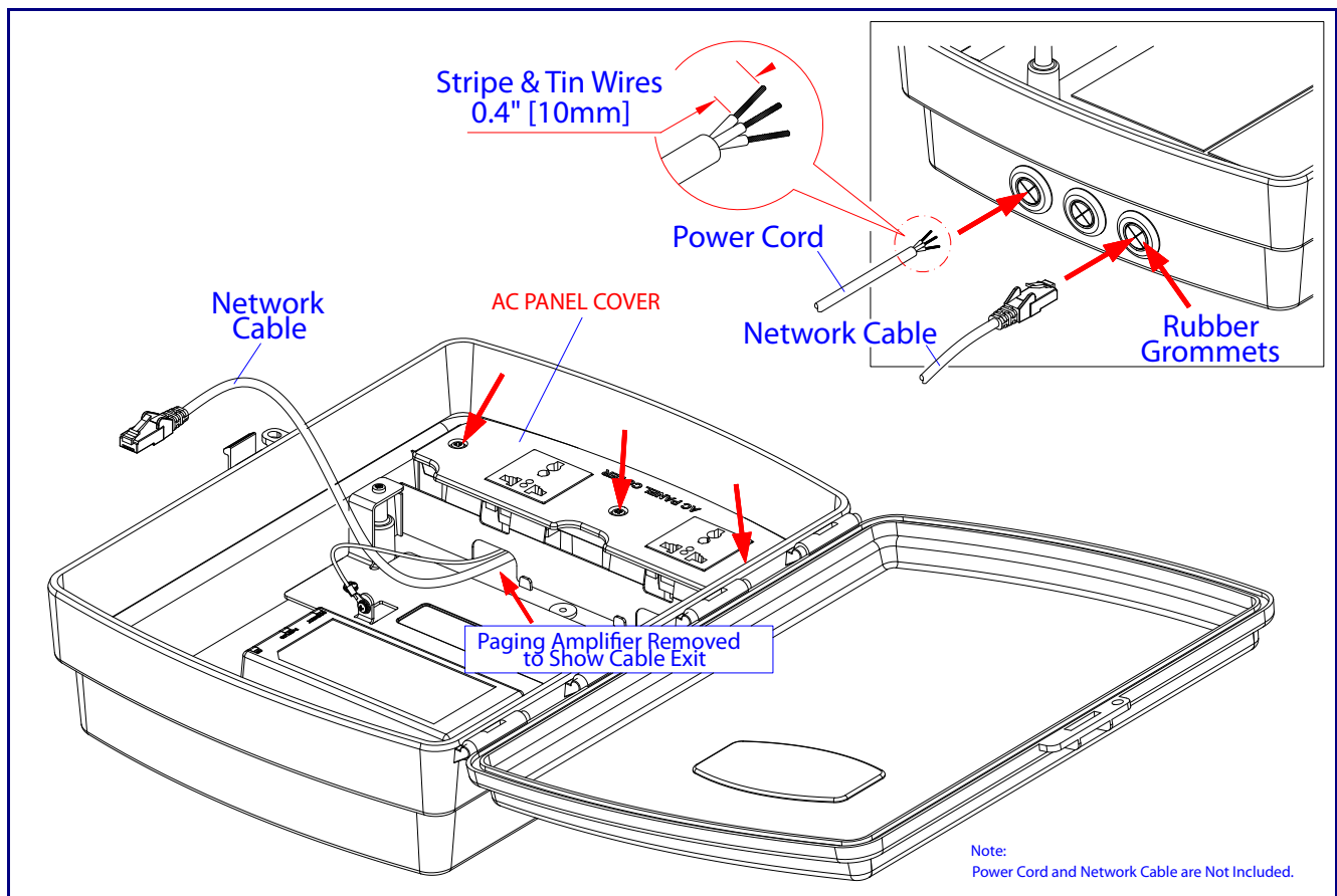
Figure 2-12. Connecting the Strobe
