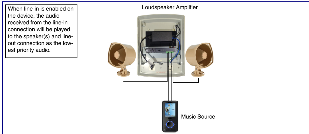
Figure 2-8. Line-In Connection
