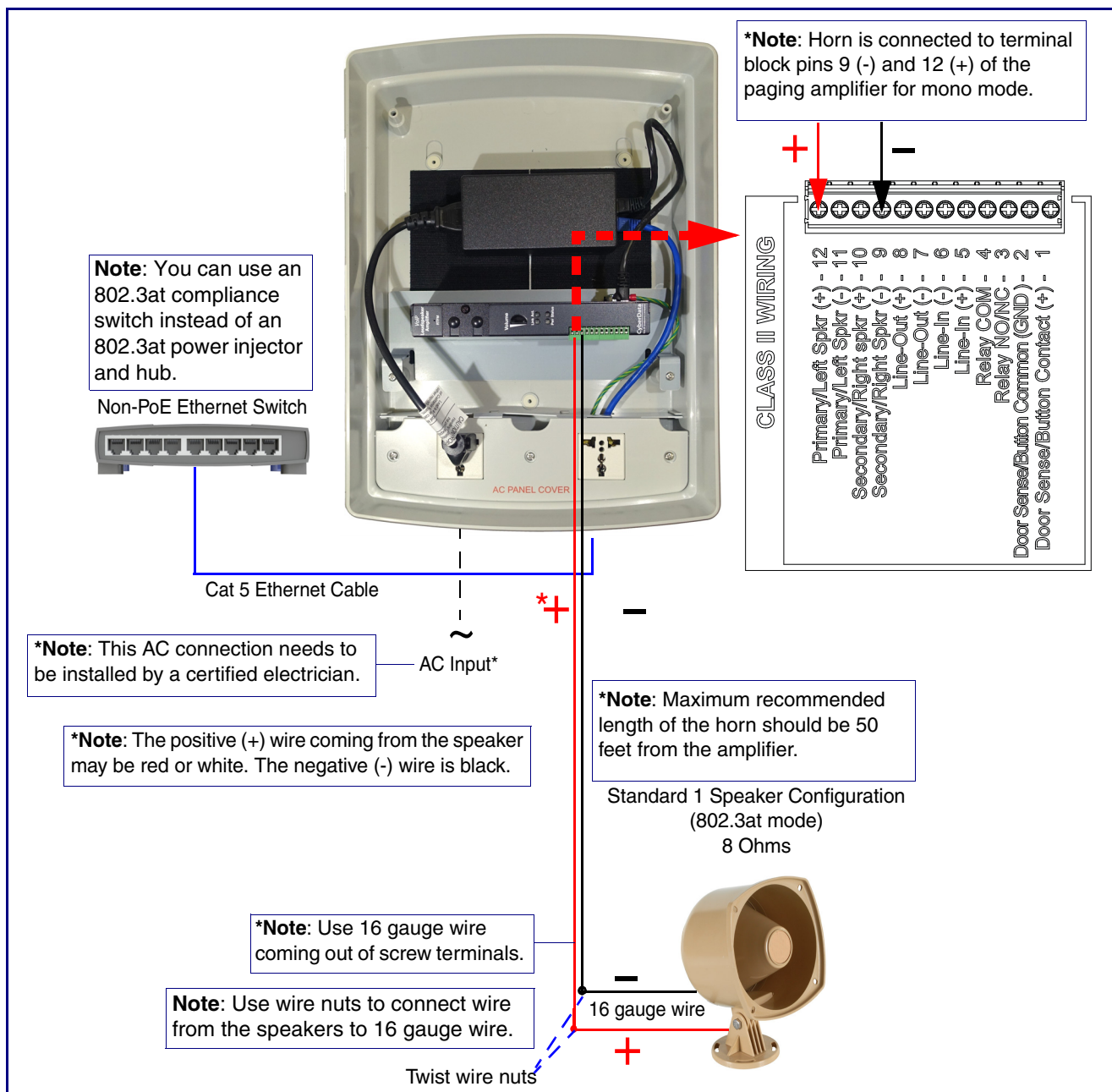
Figure 2-5. Using the Amplified Outputs—High Power Mode with One Speaker
