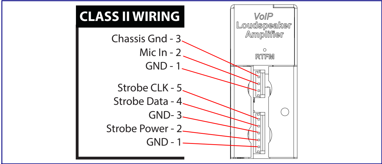
Figure 2-11. Connections Behind the Port Cover
