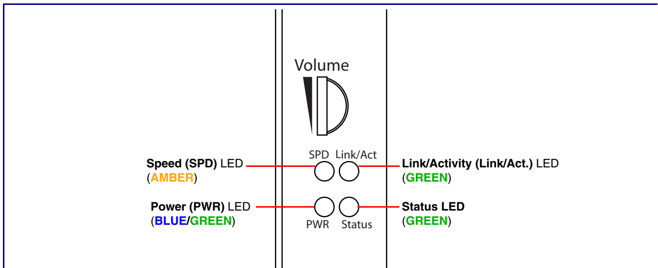
Figure 2-16. Singlewire InformaCast Loudspeaker Amplifier LEDs
