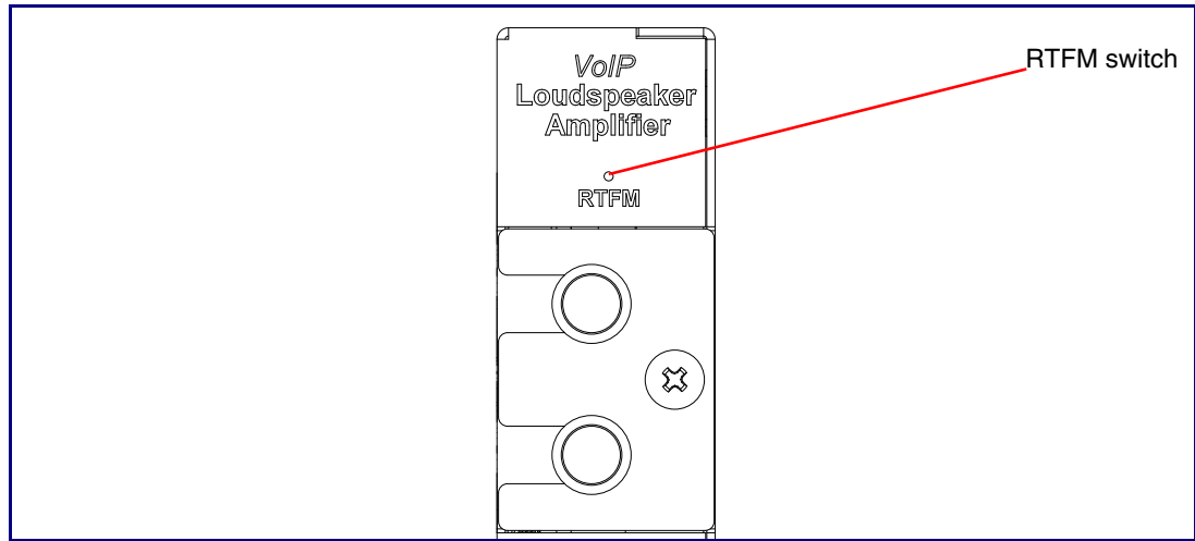
Figure 2-17. RTFM Switch
