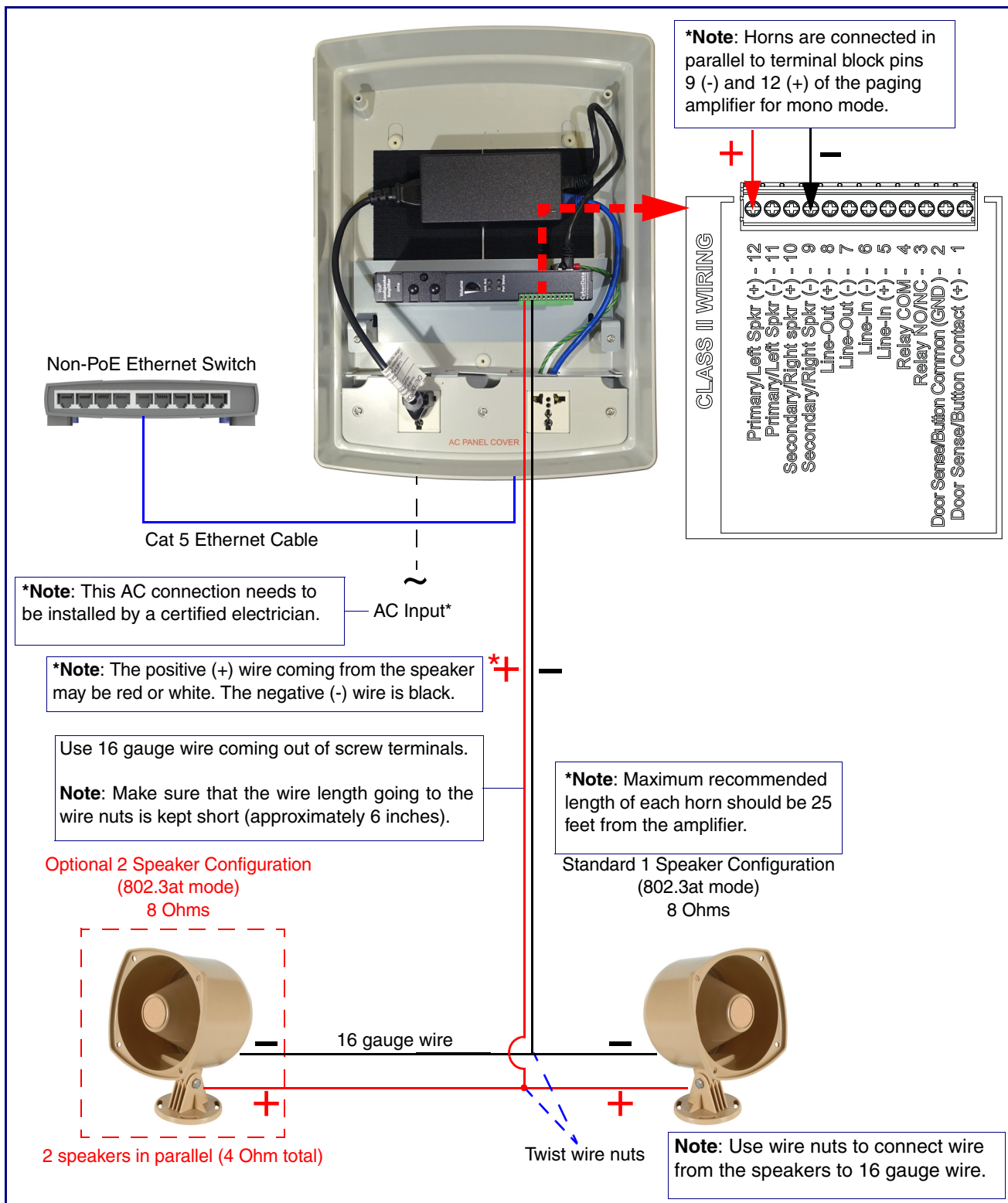
Figure 2-6. Using the Amplified Outputs—High Power Mode with Two Speakers
