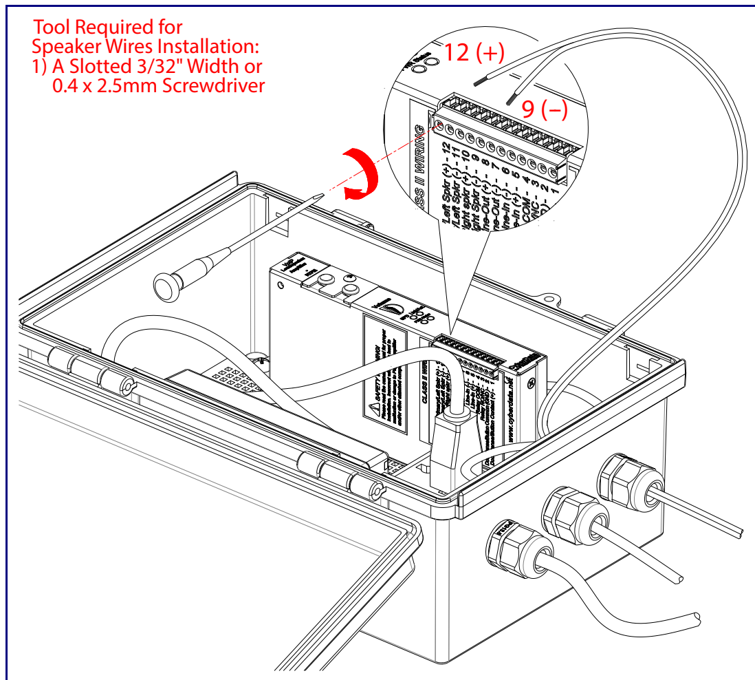
Figure 2-12. Connecting the Speaker Wires
