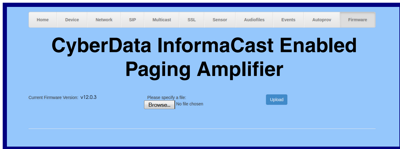
Figure 2-55. Firmware Page
