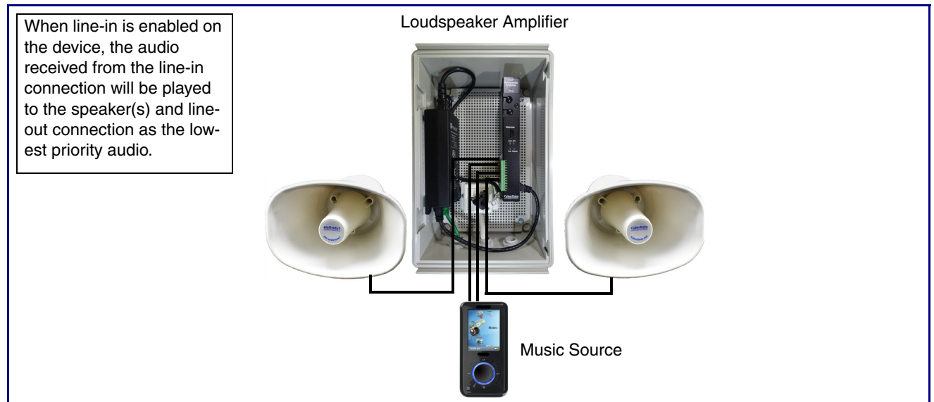
Figure 2-18. Line-In Connection
