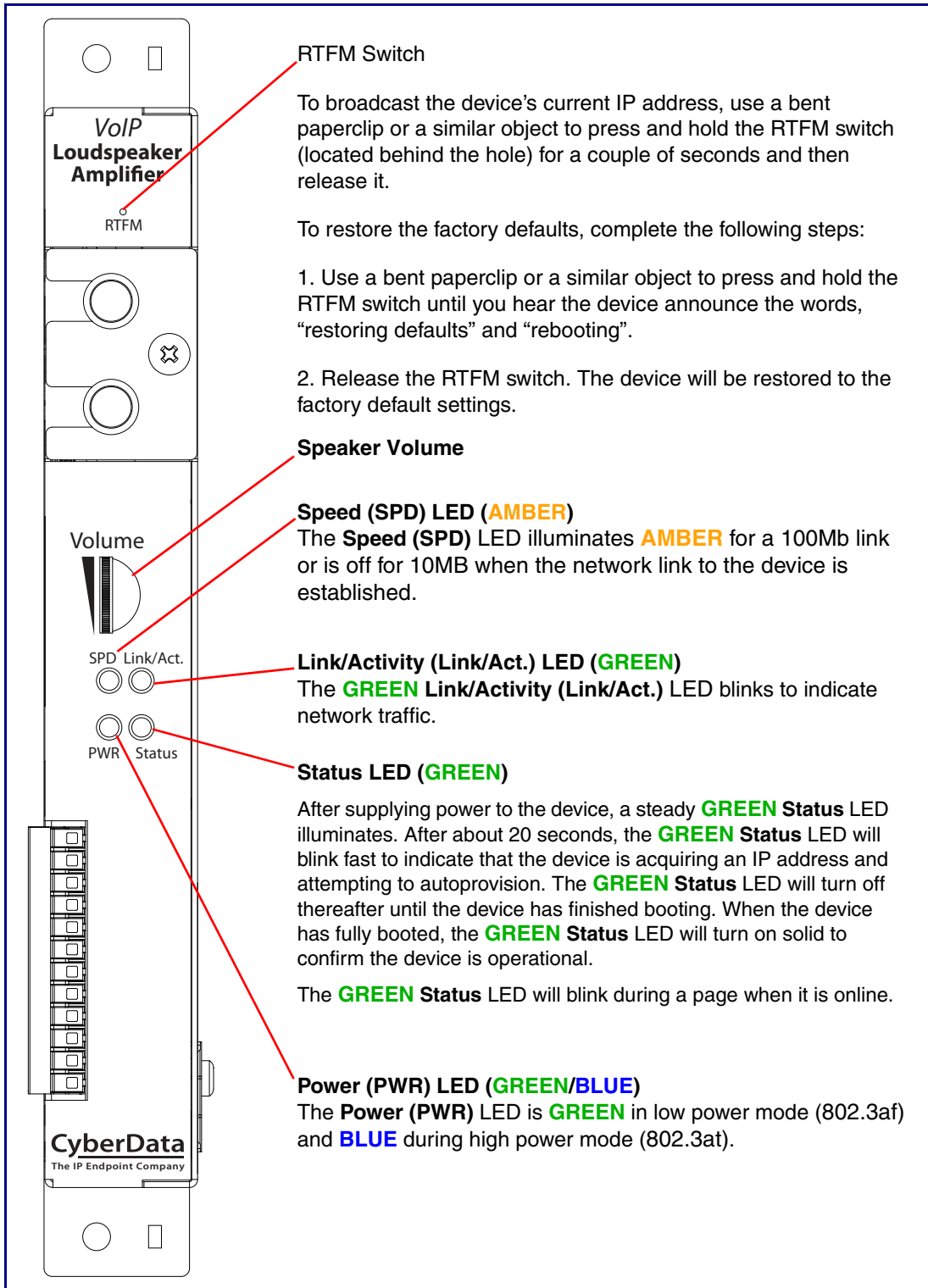
Figure 2-5. InformaCast Enabled Loudspeaker Amplifier (AC-Powered) Components
