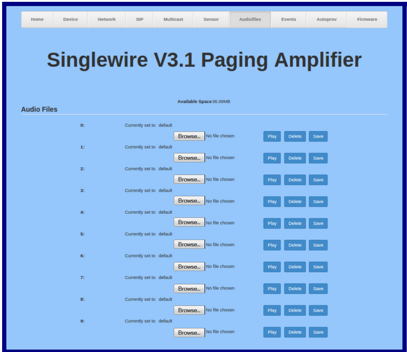
Figure 2-34. Audiofiles Page
