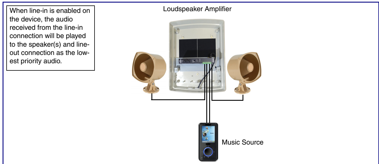
Figure 2-10. Line-In Connection
