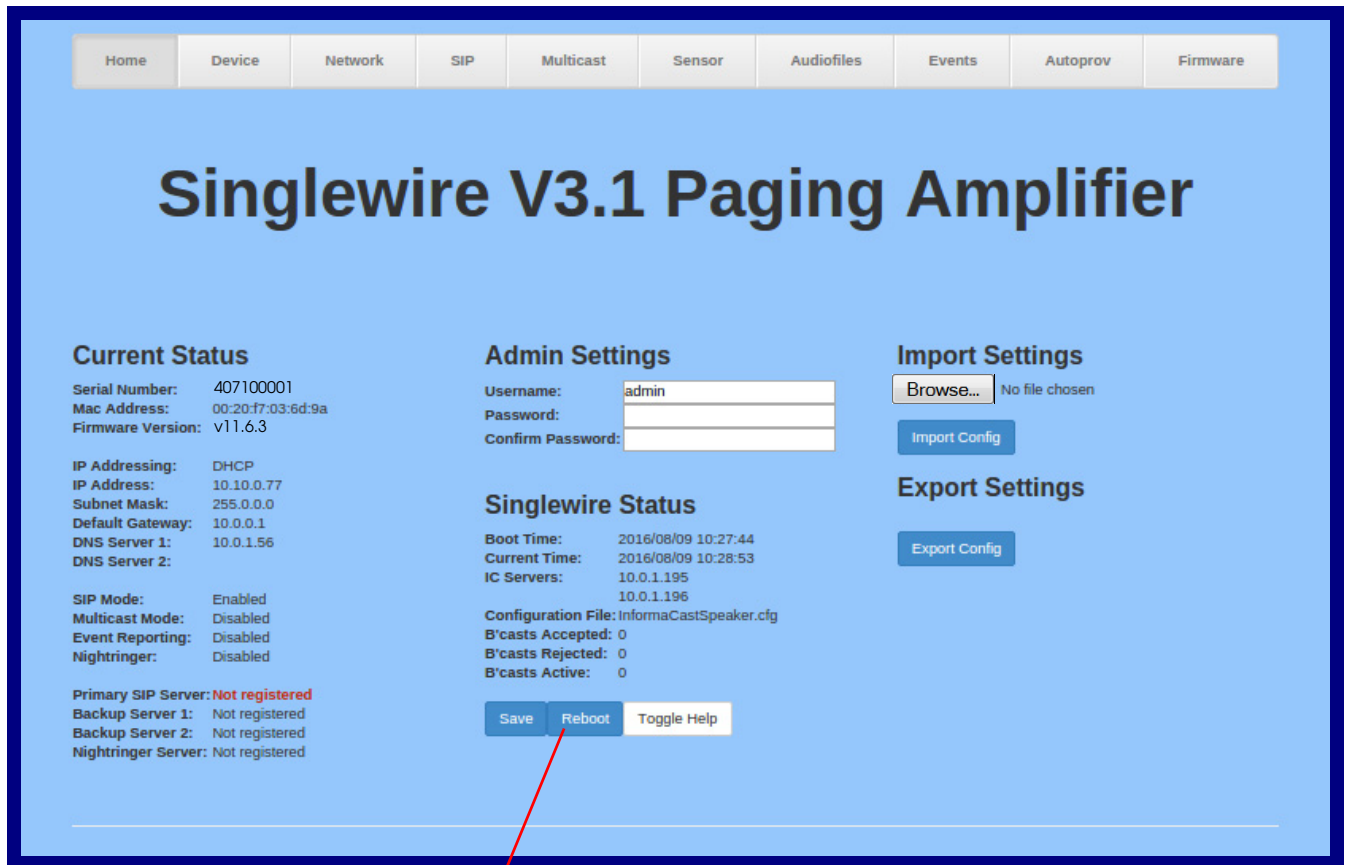
Figure 2-43. Home Page
