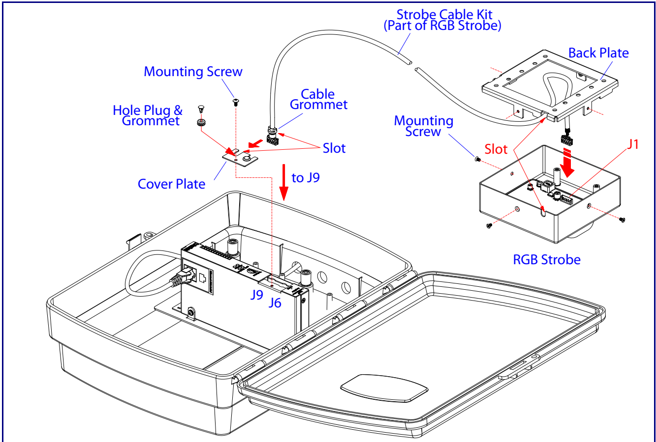
Figure 2-15. Connecting the Strobe
