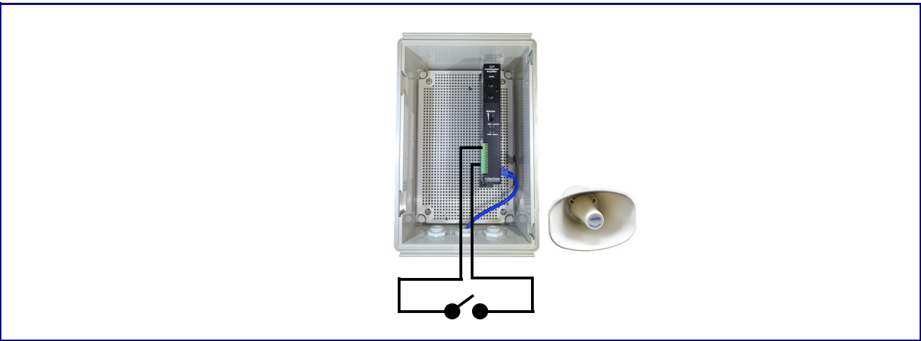
Figure 2-12. Sensor Connection
