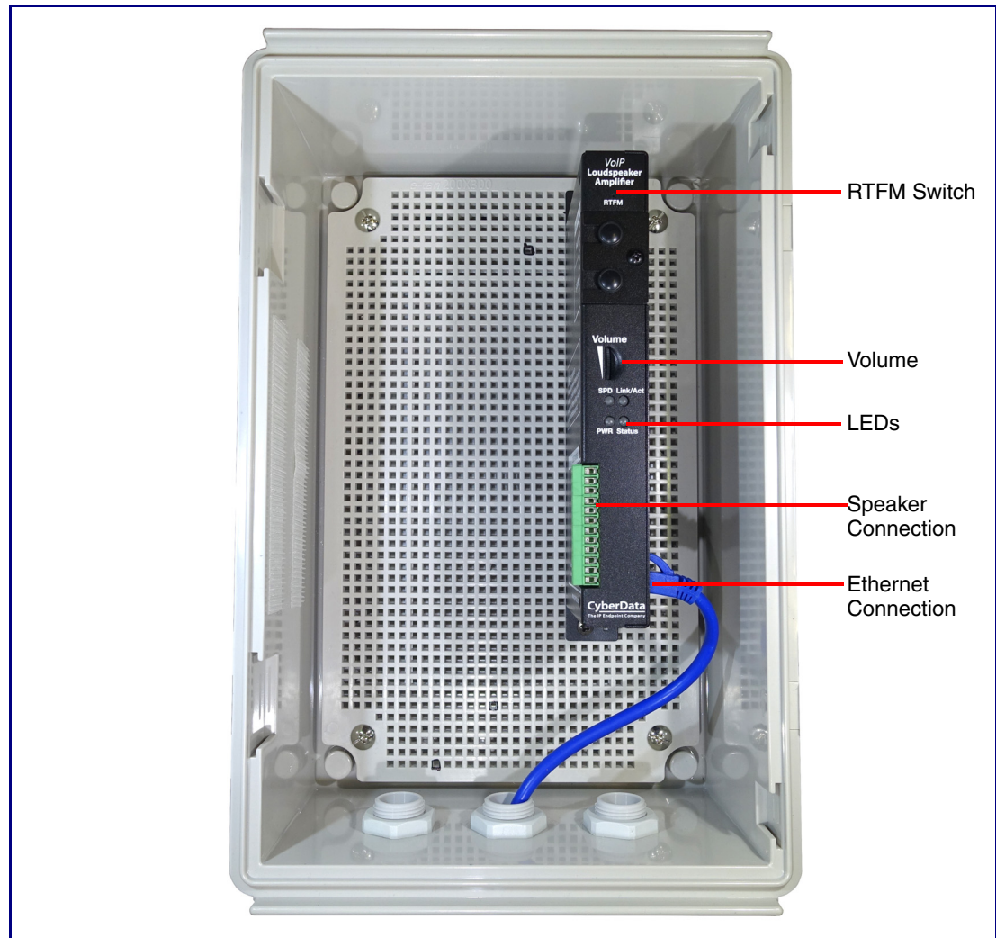
Figure 2-2. Loudspeaker Amplifier Components—PoE
