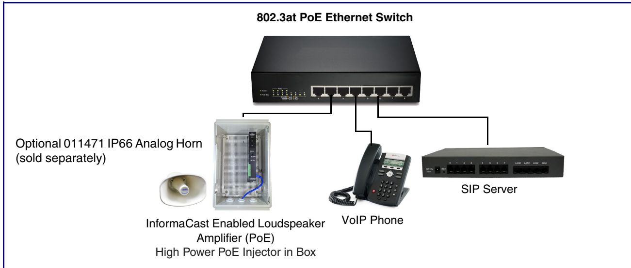
Figure 1-2. Typical Installation
