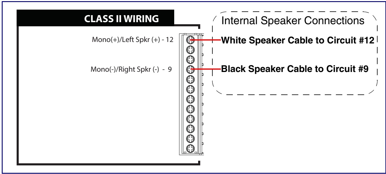
Figure 2-1. Singlewire InformaCast IP66 Outdoor Horn Connections
