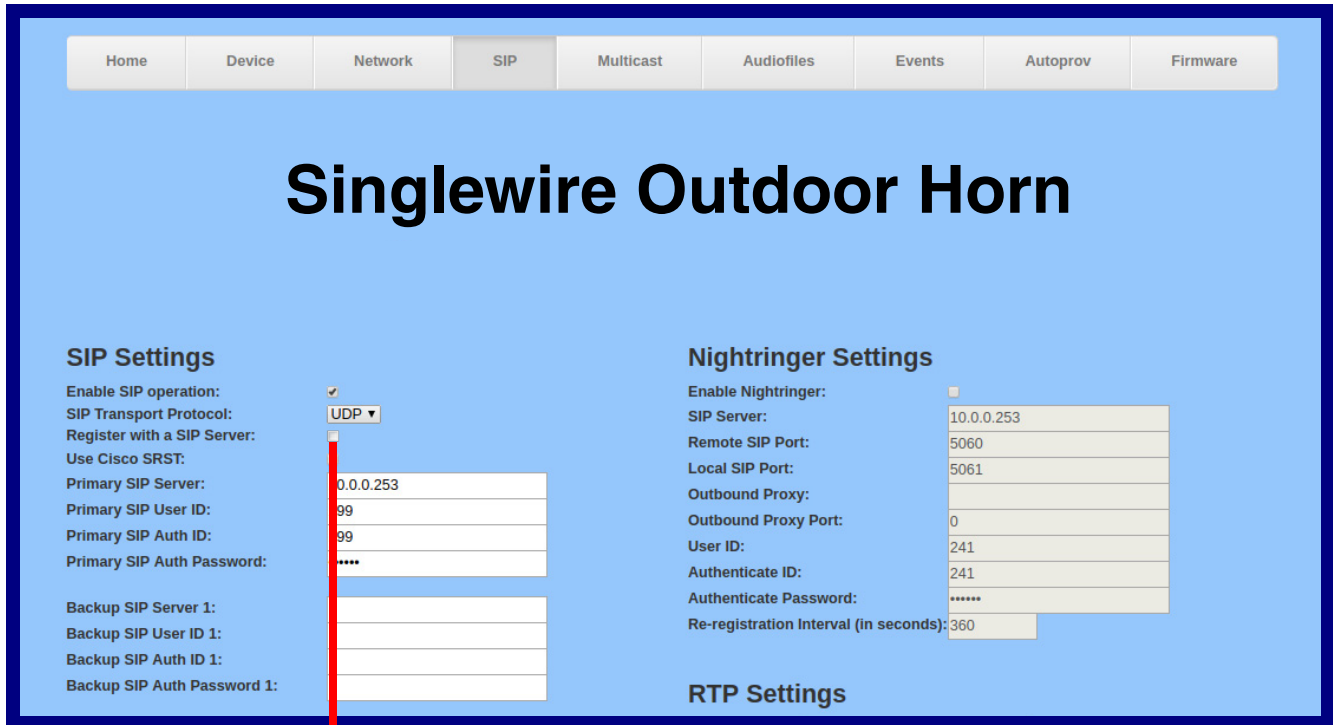
Figure 2-14. SIP Page Set to Point-to-Point Mode
