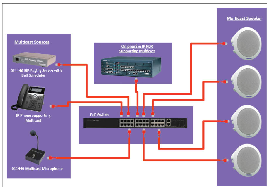
Typical IP Speaker Configuration
