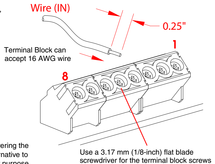
Figure 2-1. Connections and Alternate Power Input
