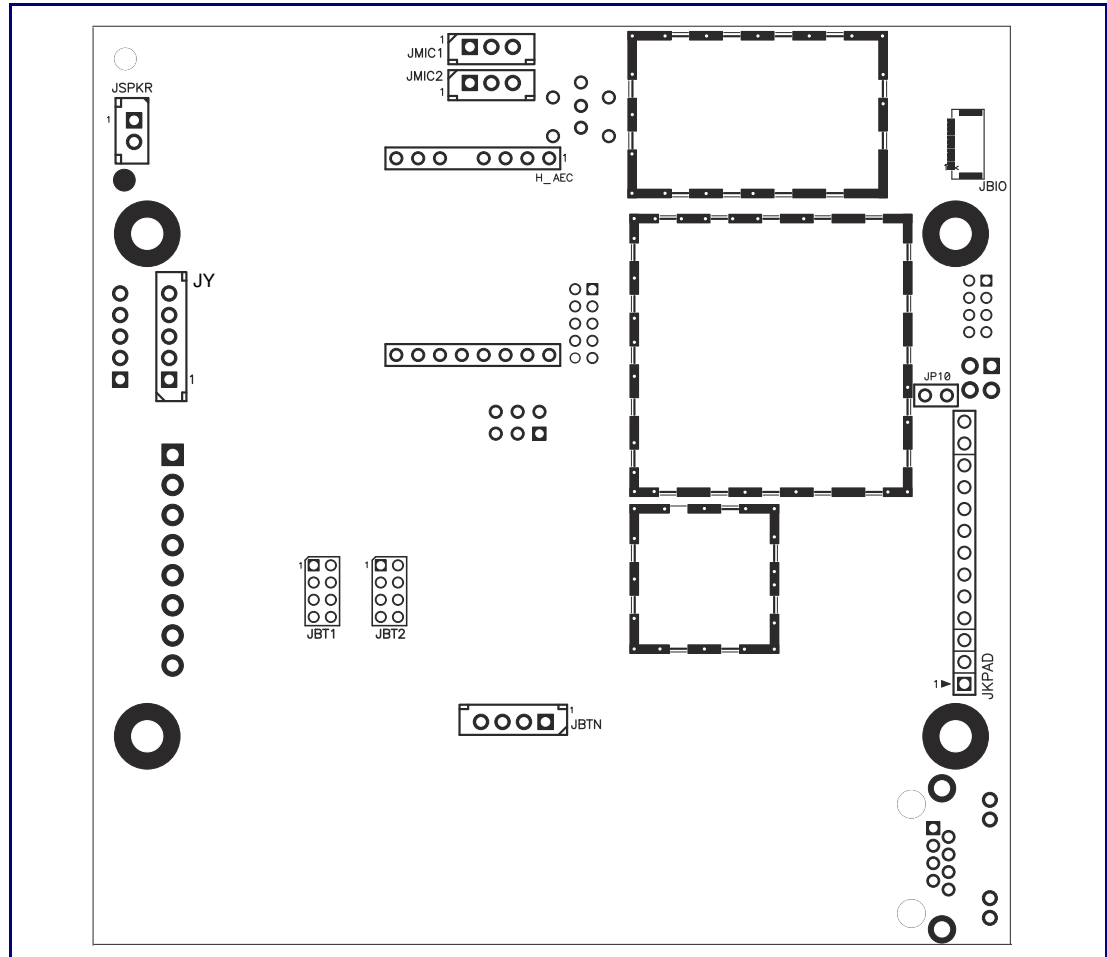
Figure 2-6. Connector Locations
