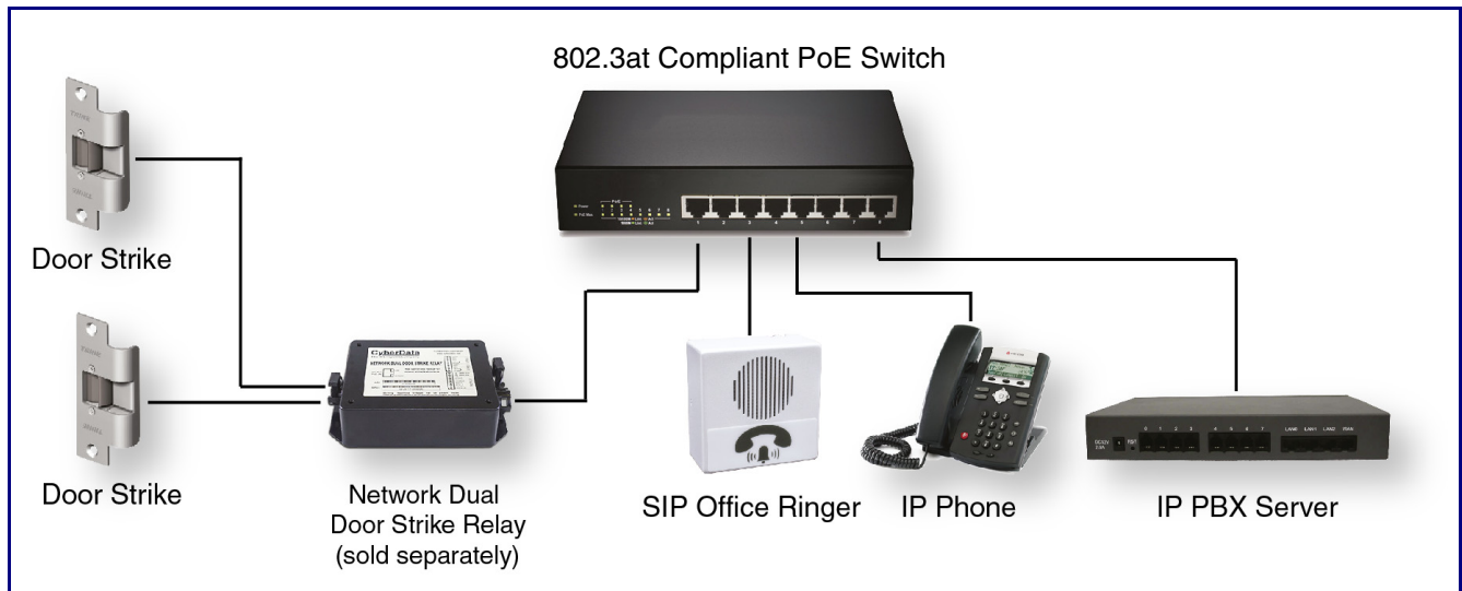
Figure 1-3. Typical Installation Example
