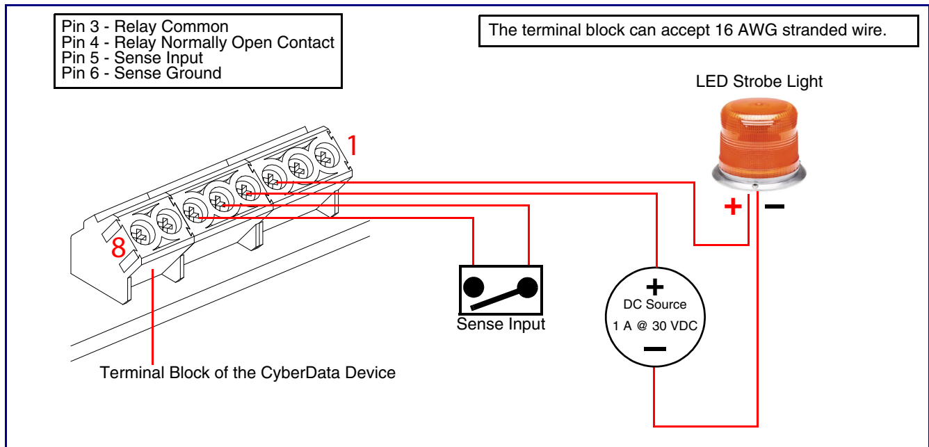
Figure 2-6. Devices Less than 1A at 30 VDC
