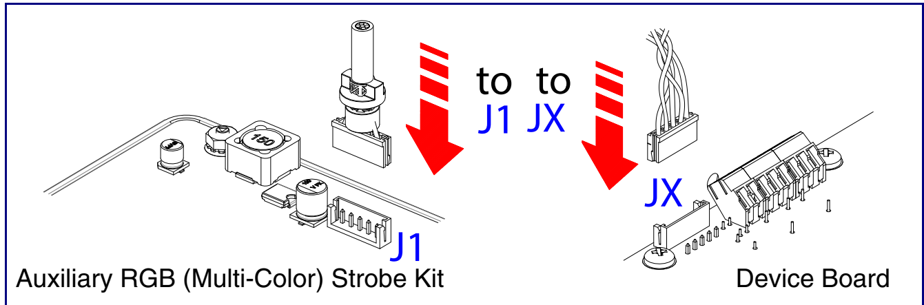
Figure 2-11. Connecting the Auxiliary RGB (Multi-Color) Strobe Kit to the Device
