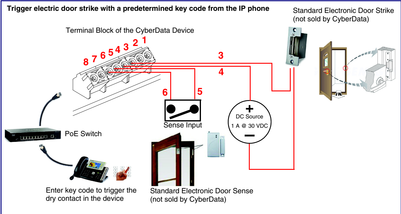
Figure 2-7. Example Installation - Door Strike
