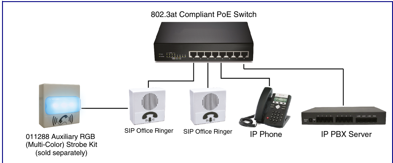
Figure 1-3. Typical Installation Example
