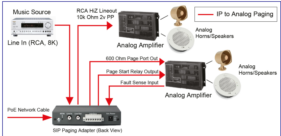
Figure 2-3. Typical Installation
