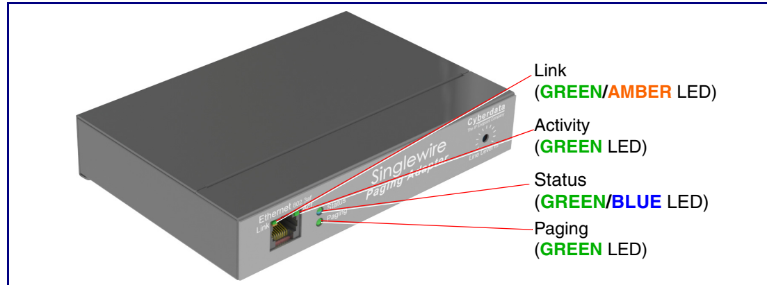
Figure 2-8. SIP Paging Adapter LEDs
