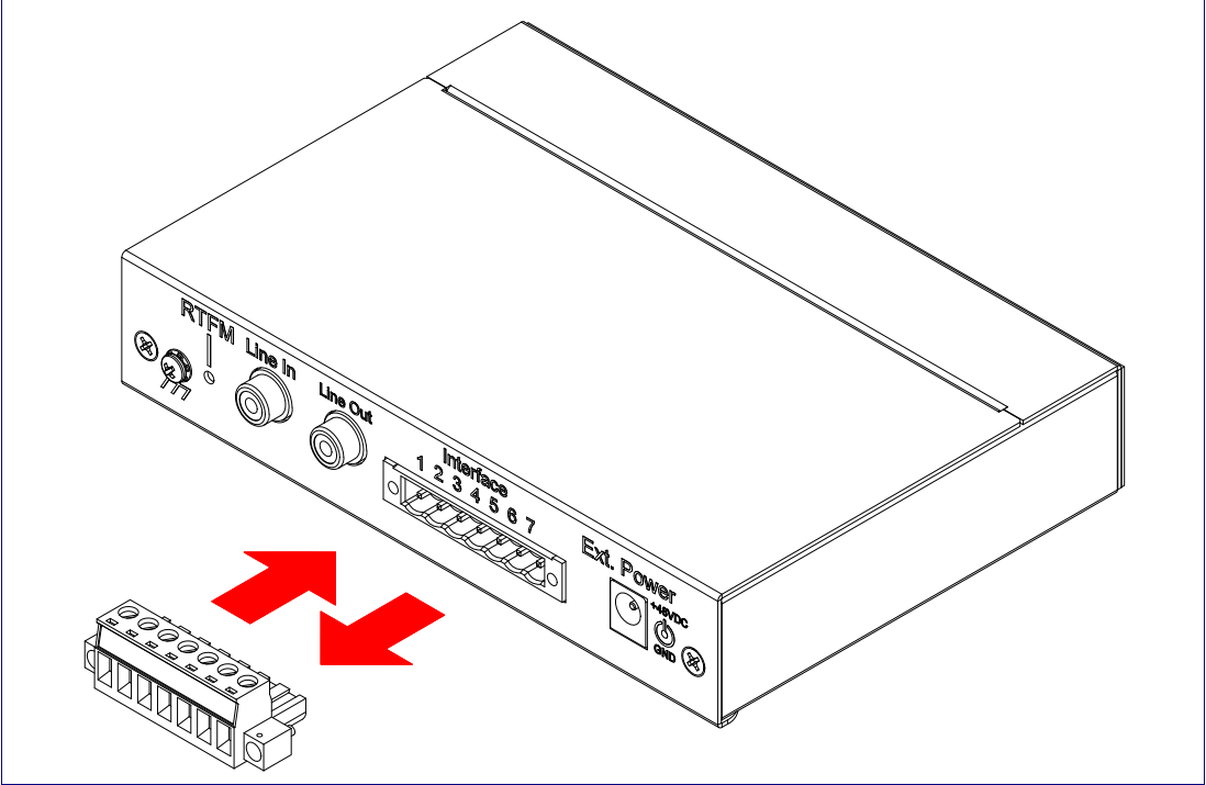
Figure 2-5. Removable Interface Connector
