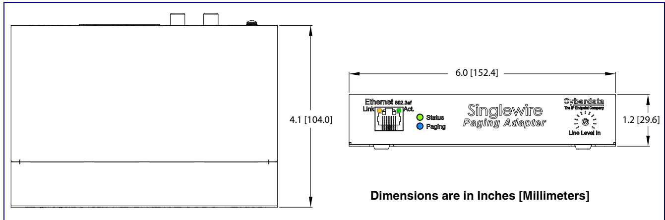
Figure 1-2. Dimensions
