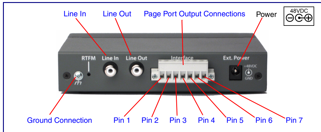
Figure 2-4. Connection Options
