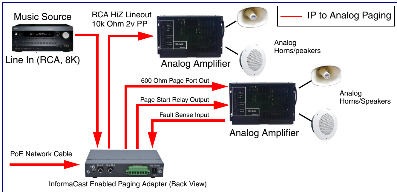
Figure 2-1. Typical Installation
