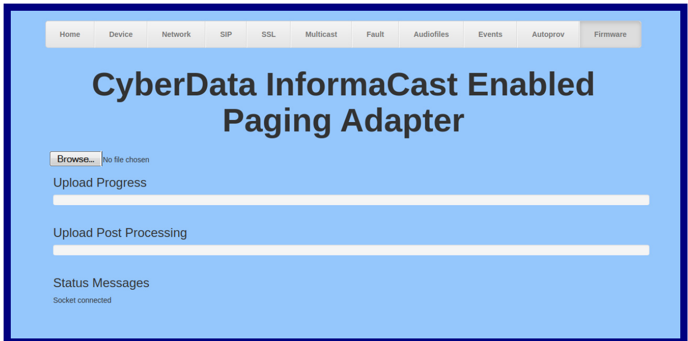
Figure 2-32. Firmware Page
