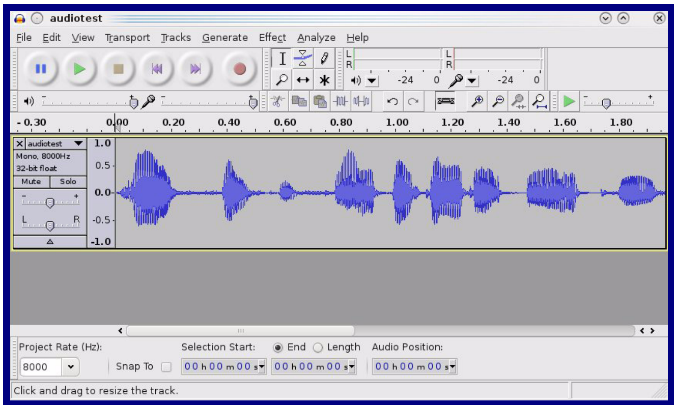
Figure 2-26. Audacity 1
