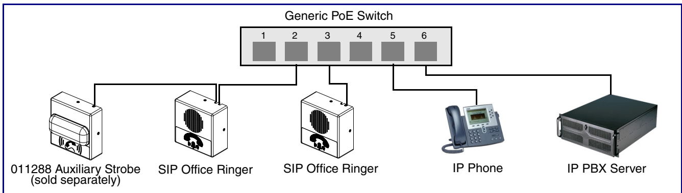
Figure 1-2. Typical Installation
