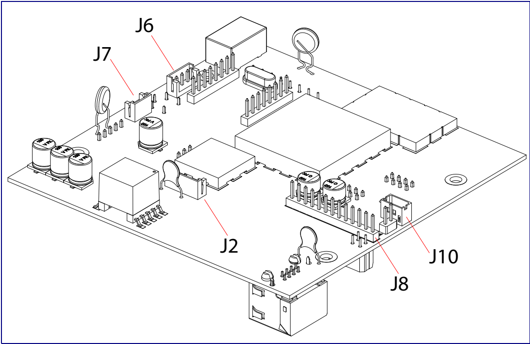
Figure 2-9. Connector Locations
