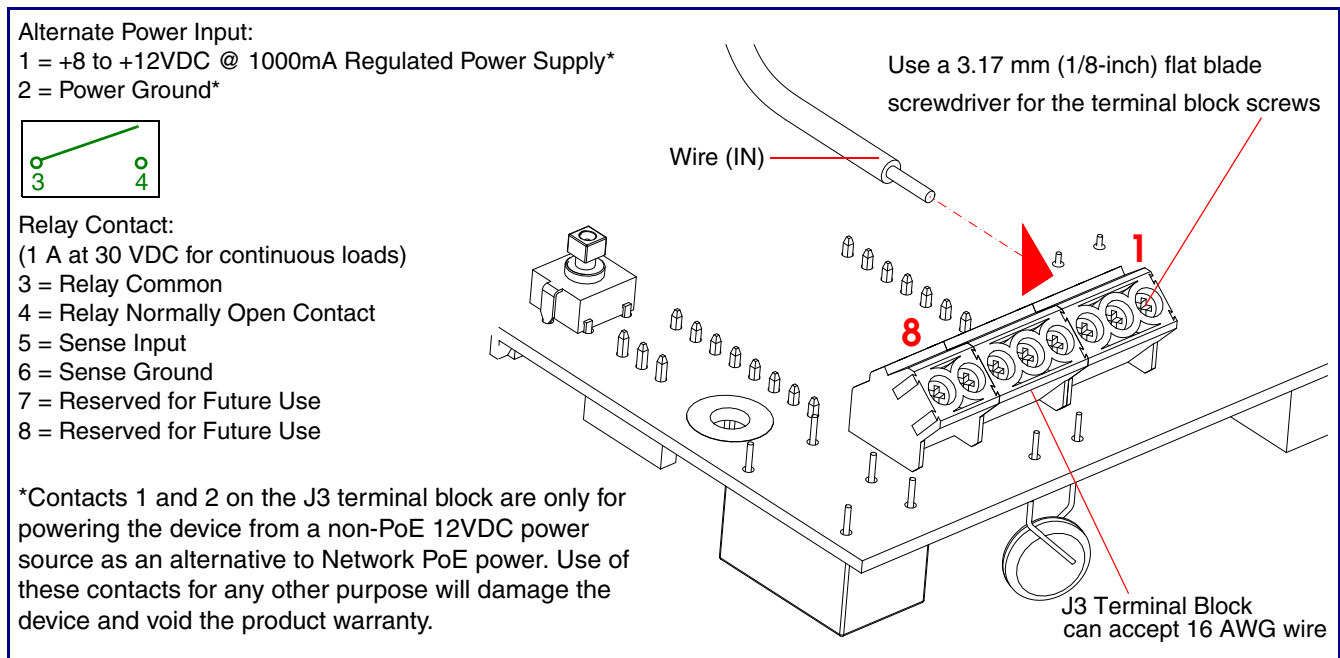
Figure 2-5. Connections
