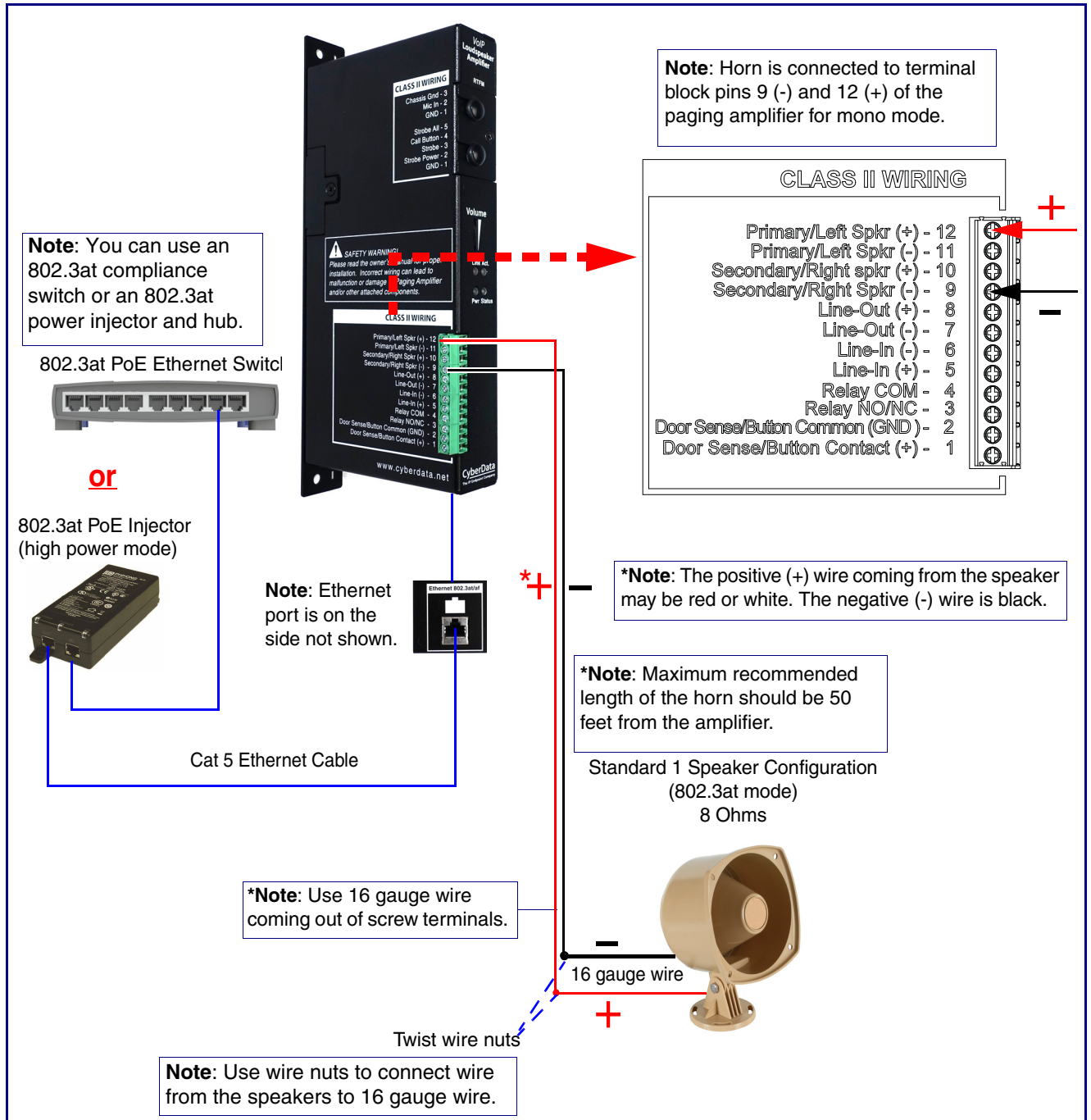
Figure 2-6. Using the Amplified Outputs—High Power Mode with One Speaker
