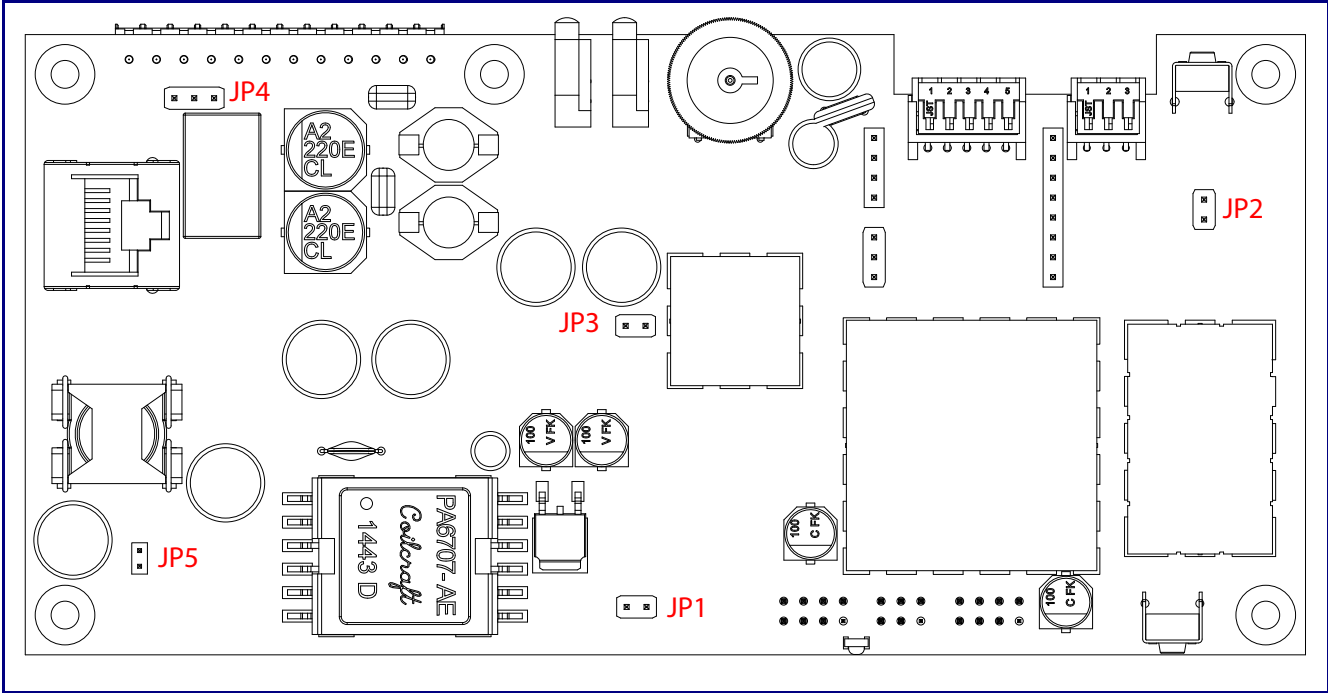
Figure 2-14. Jumper Locations
