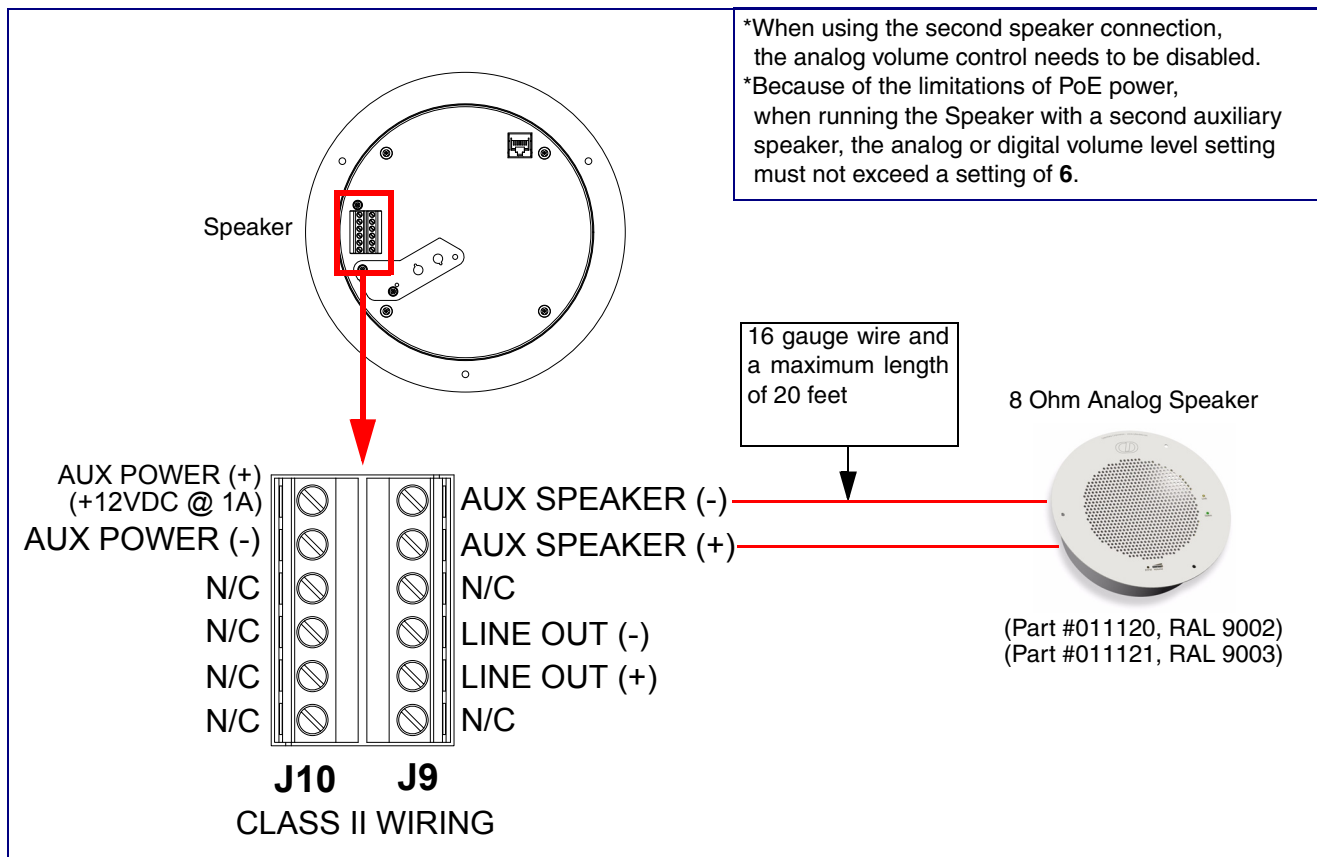
Figure 2-6. Singlewire InformaCast Speaker with Extra Speaker Connection
