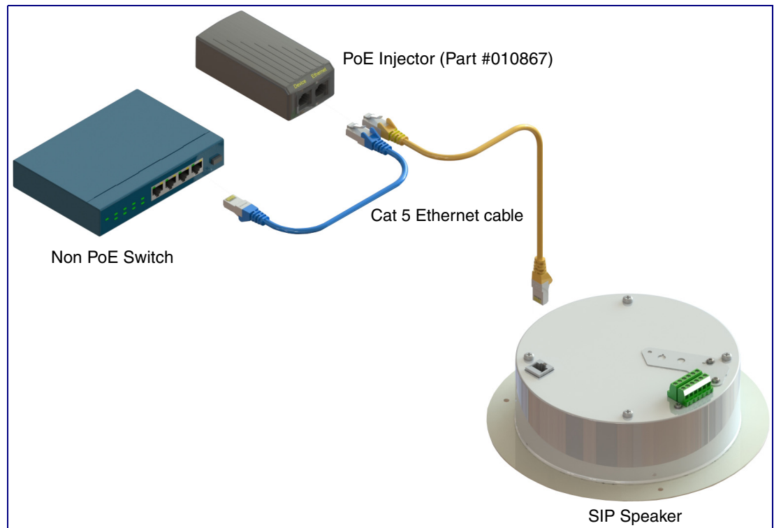
Figure 2-4. Singlewire InformaCast Speaker Speaker (with PoE Injector) to a Non PoE Switch
