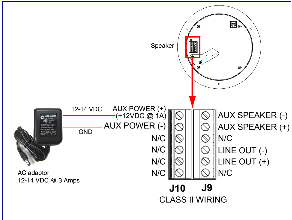
Figure 2-5. Running the Singlewire InformaCast Speaker with Auxiliary Power
