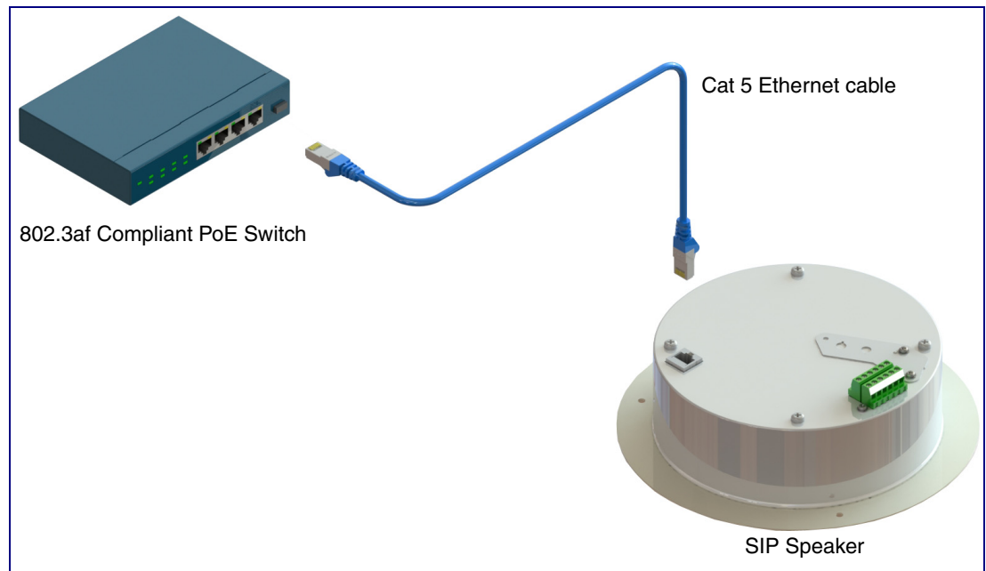
Figure 2-3. Singlewire InformaCast Speaker to a 802.3af Compliant PoE Switch
