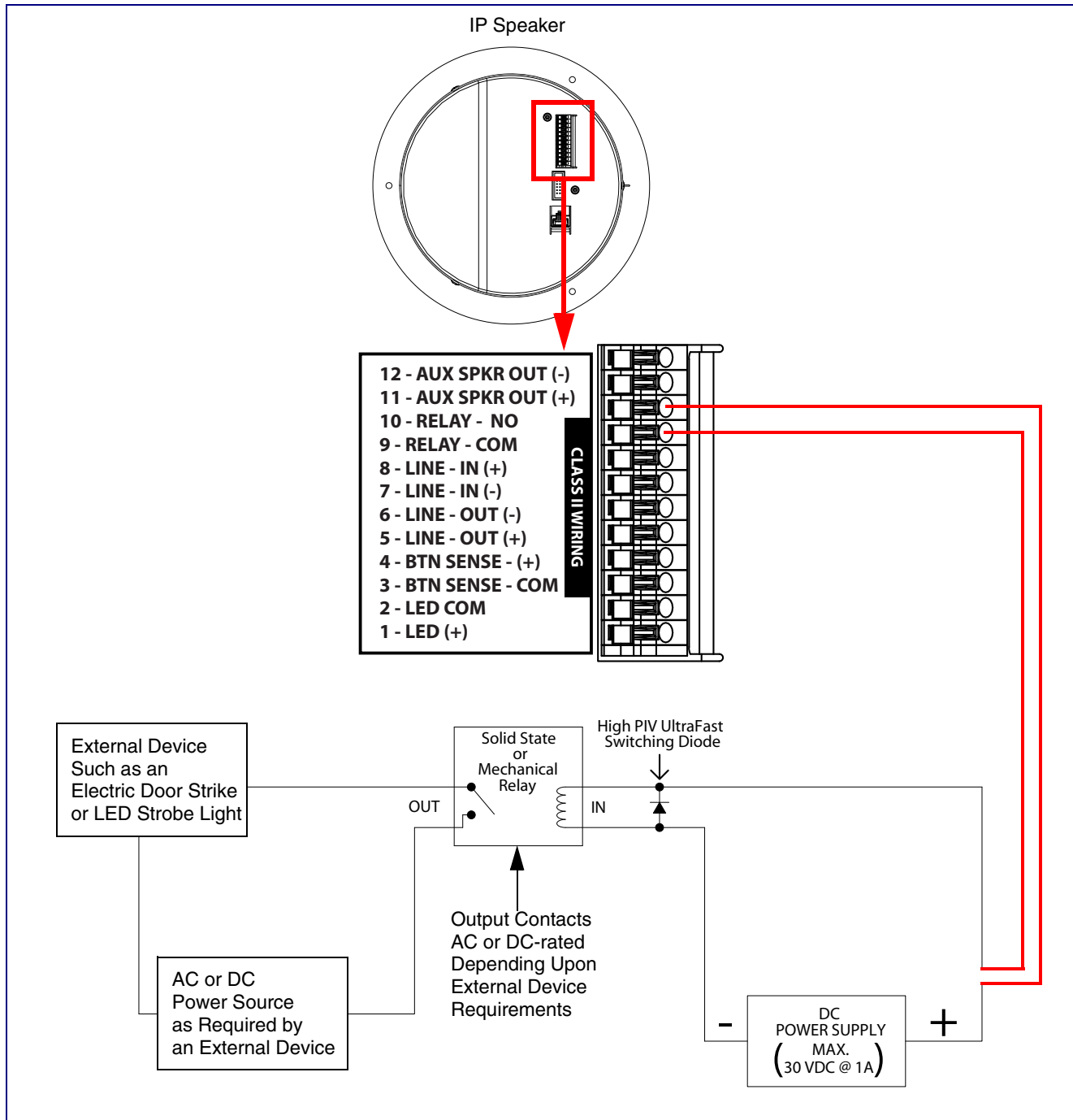
Figure 2-4. InformaCast Enabled Speaker with Talk-Back with Alert Strobe
