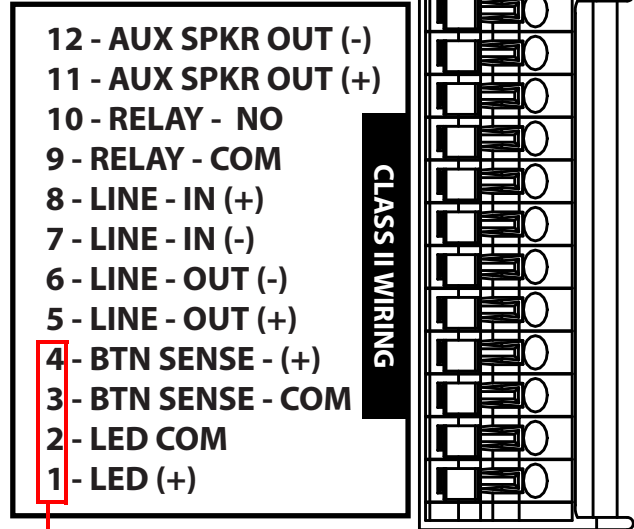
Figure 1-3. Optional Connections
