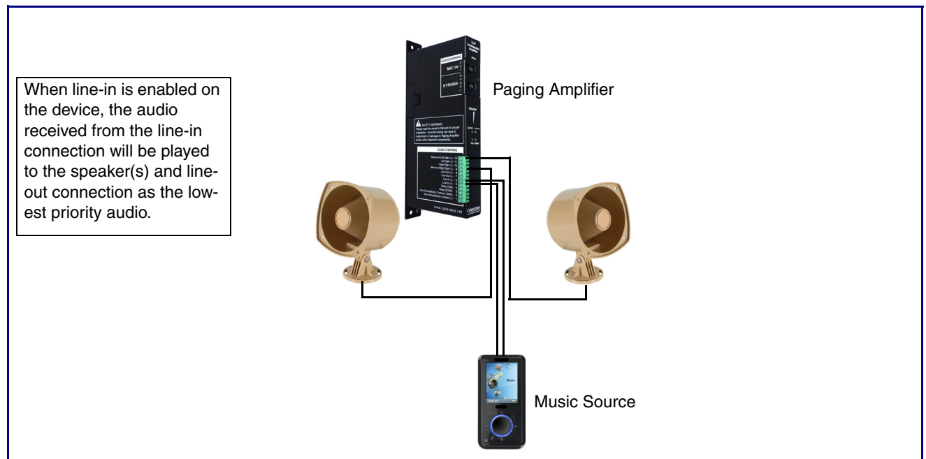
Figure 2-9. Line-In Connection
