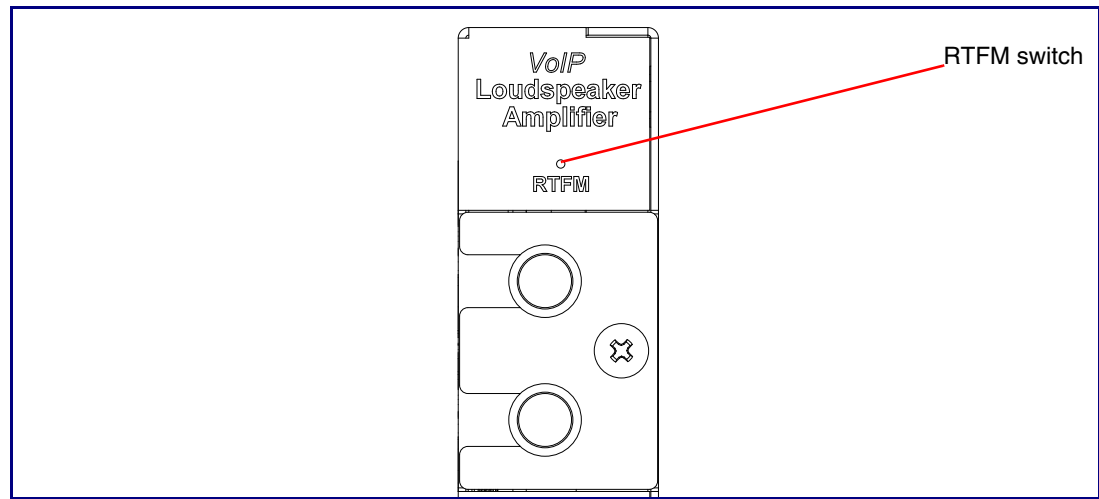
Figure 2-17. RTFM Switch
