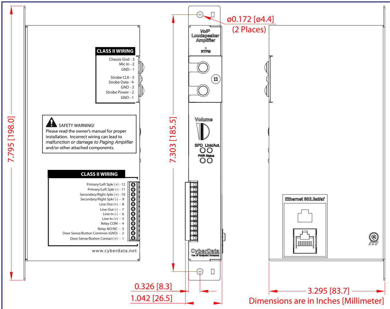
Figure A-1. Dimensions
