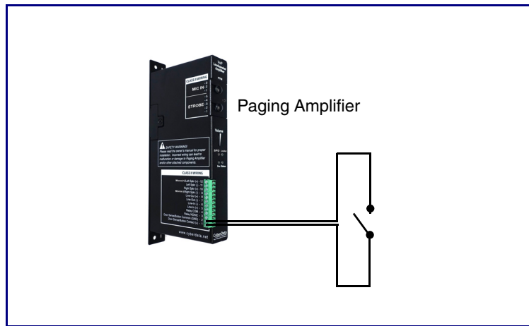
Figure 2-11. Sensor Connection
