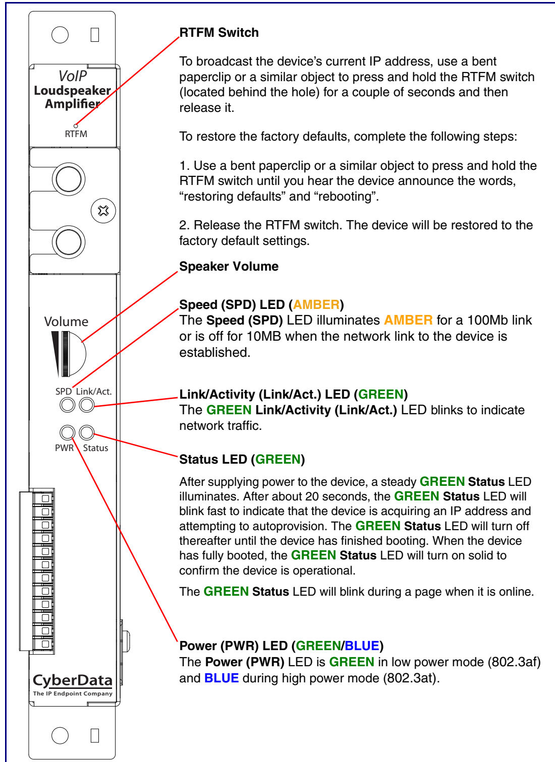
Figure 2-5. Singlewire InformaCast Paging Amplifier Components
