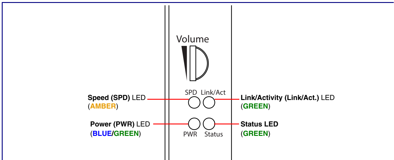
Figure 2-17. InformaCast Enabled Paging Amplifier LEDs
