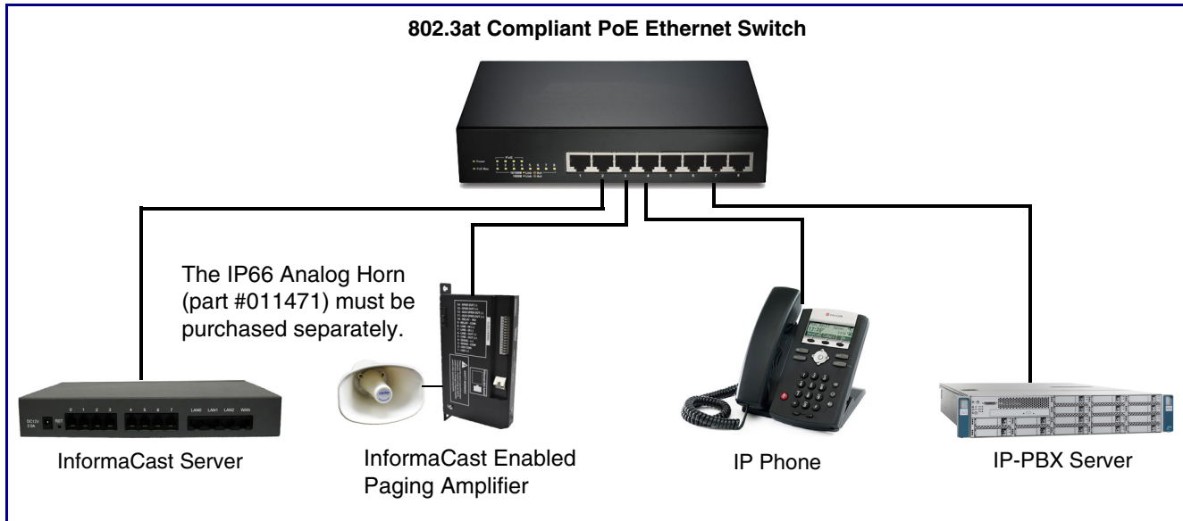
Figure 1-2. Typical Installation
