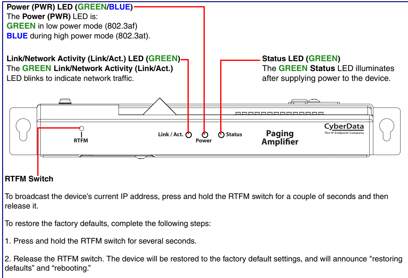
Figure 2-5. InformaCast Enabled Paging Amplifier Components
