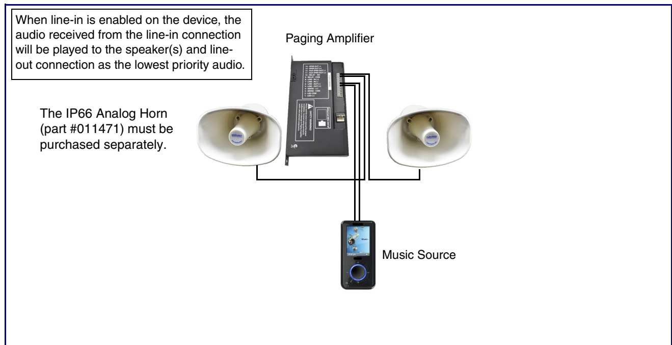
Figure 2-10. Line-In Connection
