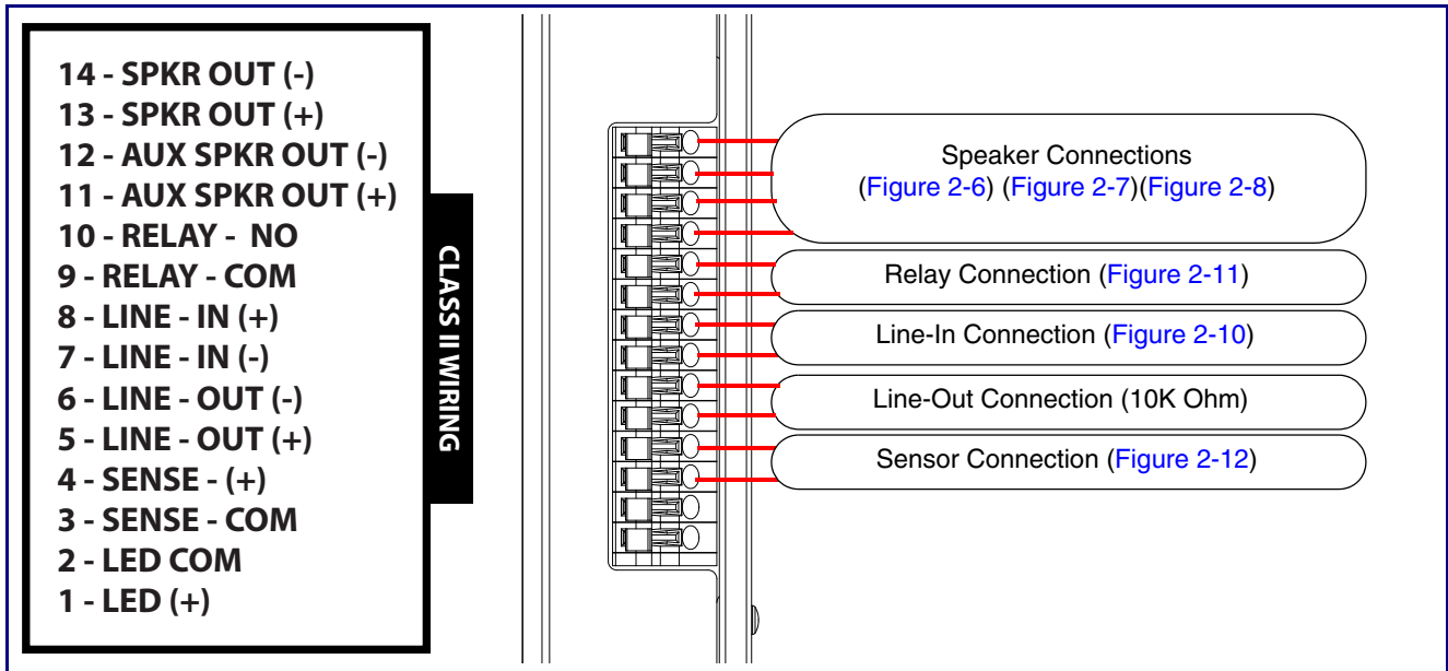
Figure 2-9. InformaCast Enabled Paging Amplifier Connections
