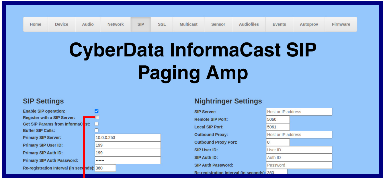
Figure 2-29. SIP Page Set to Point-to-Point Mode
