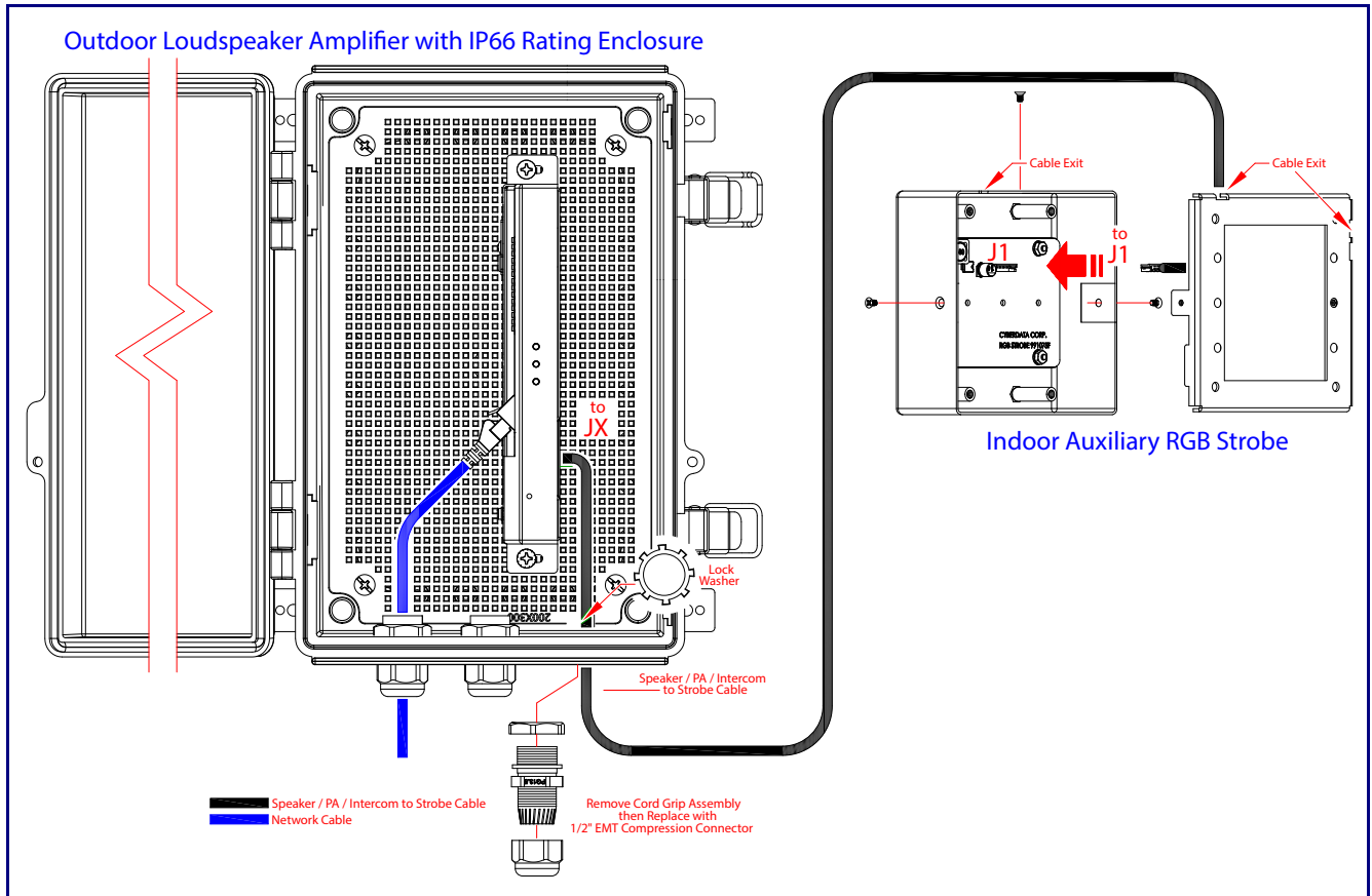
Figure 2-15. Connecting the 011288 Auxiliary RGB (Multi-Color) Strobe Kit
