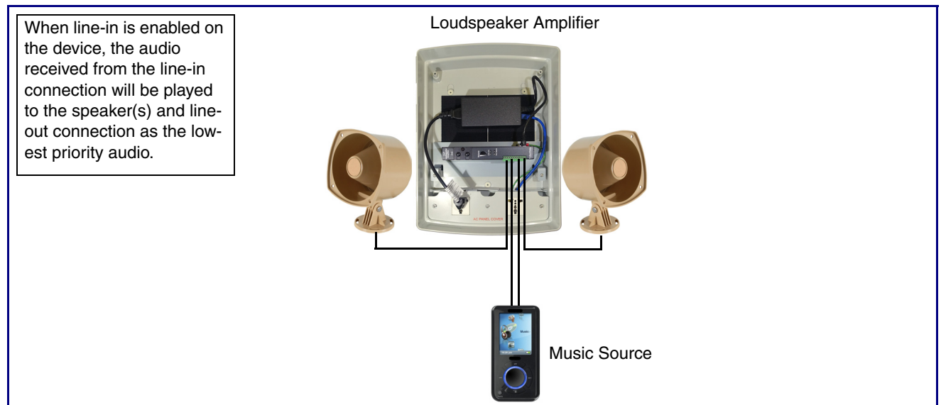
Figure 2-6. Line-In Connection
