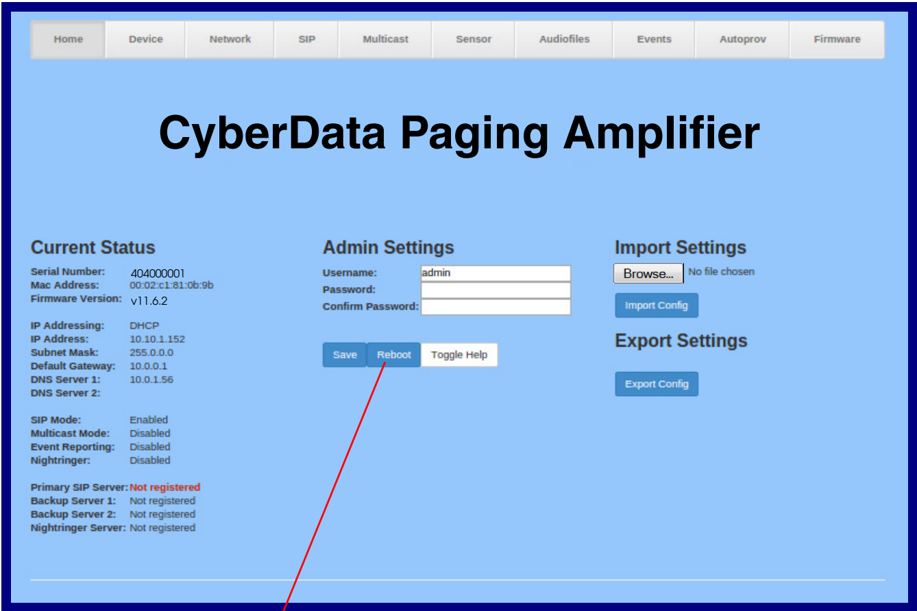
Figure 2-39. Home Page
