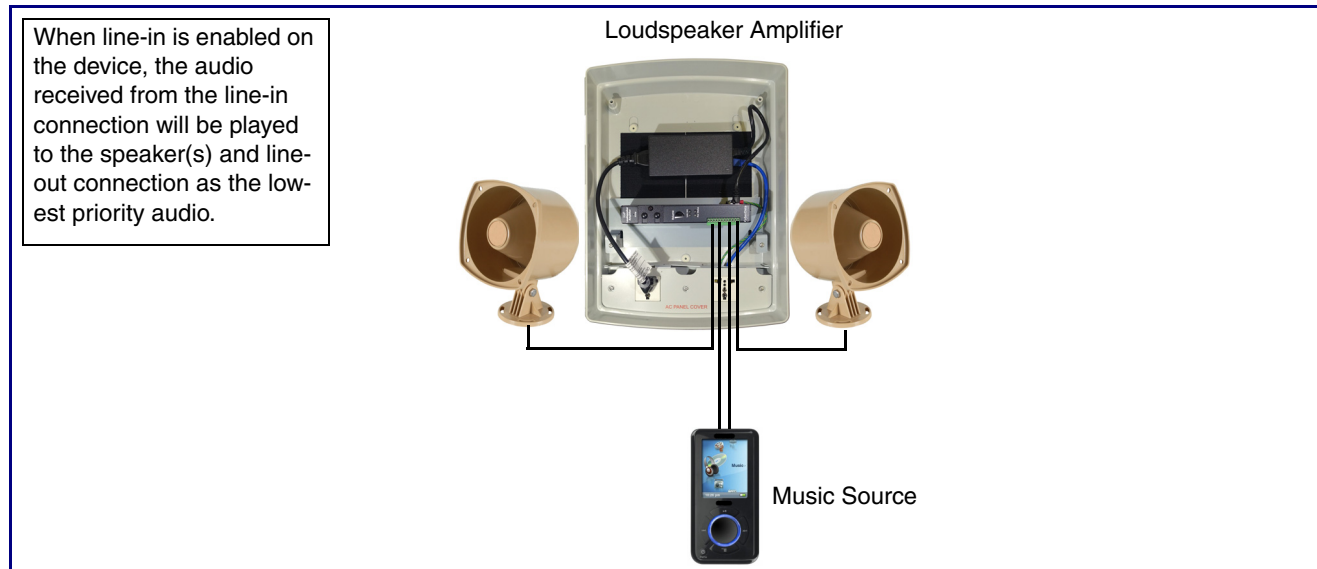
Figure 2-6. Line-In Connection
