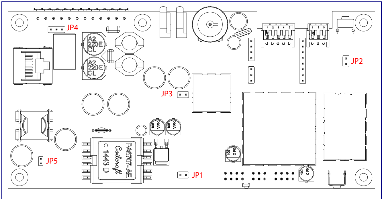
Figure 2-12. Jumper Locations
