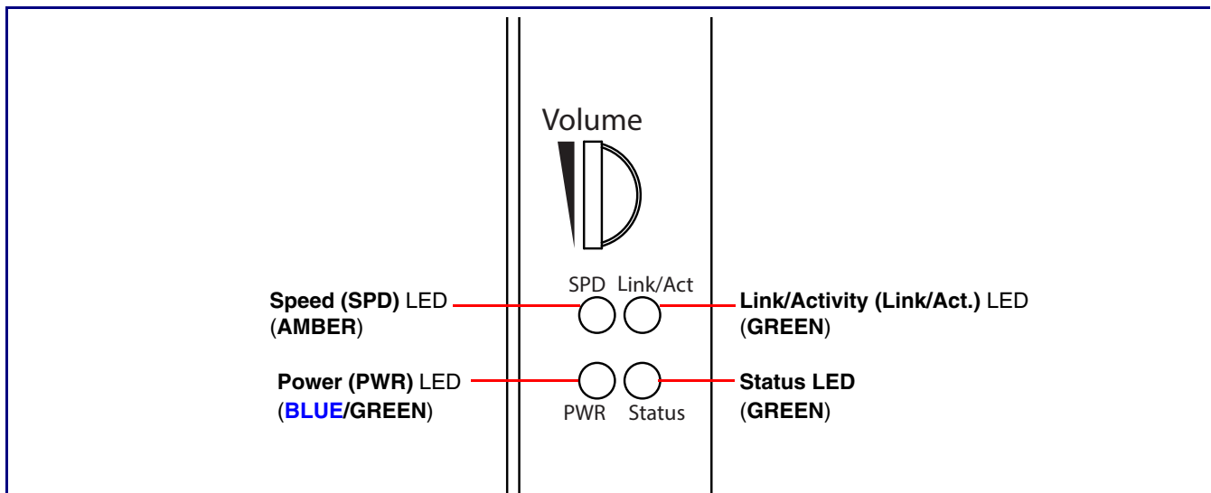
Figure 2-14. SIP Loudspeaker Amplifier (AC-Powered) LEDs
