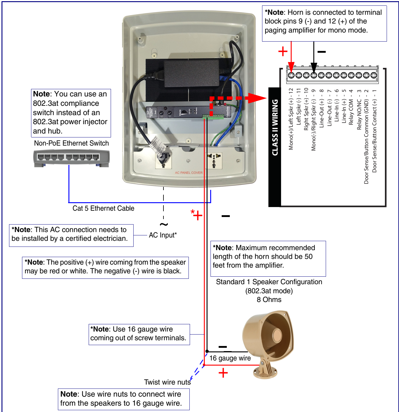
Figure 2-3. Using the Amplified Outputs—High Power Mode with One Speaker
