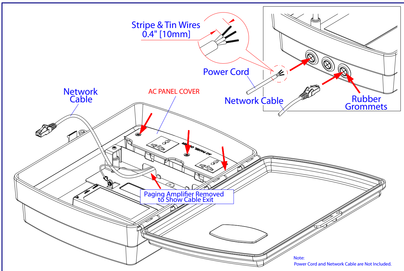
Figure 2-10. Power Cord and Network Cable Through Rubber Grommet and Prepare Power Cord Wires for Receptacle on AC Panel Cover
