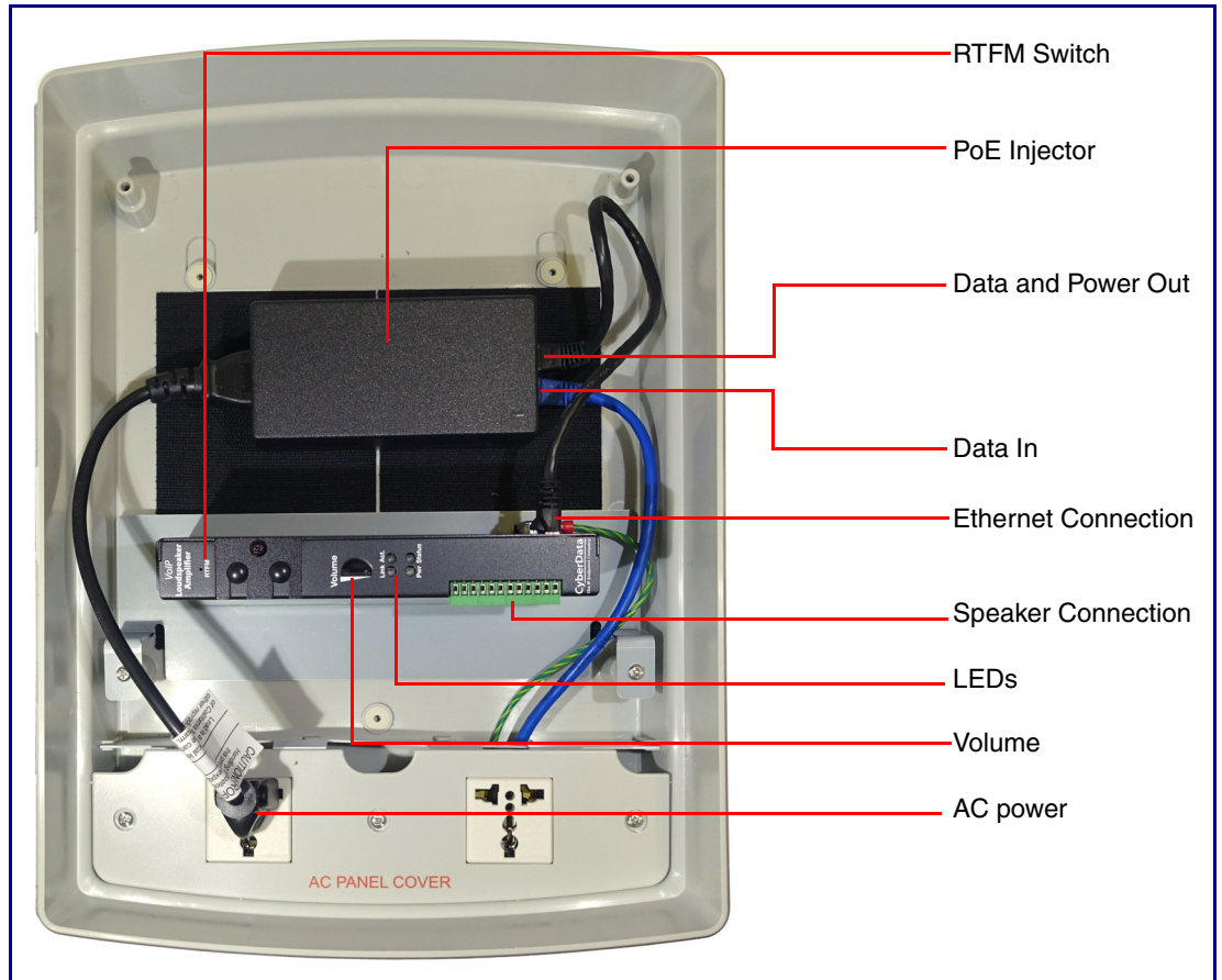
Figure 2-2. Loudspeaker Amplifier Components—AC powered
