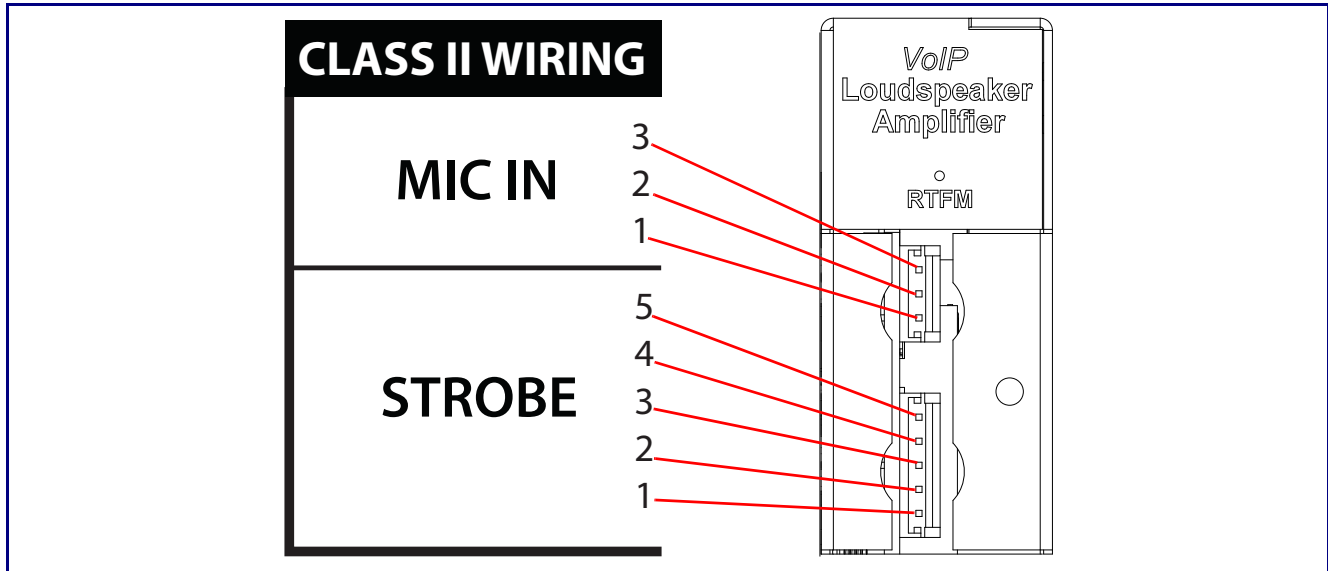
Figure 2-9. Connections Behind the Port Cover
