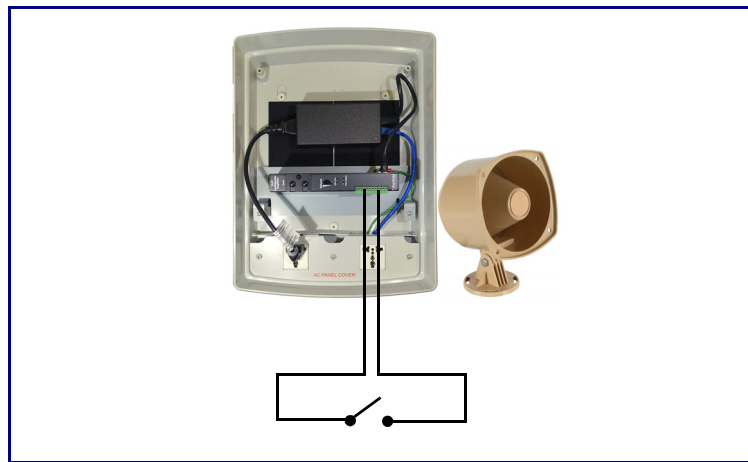
Figure 2-8. Sensor Connection
