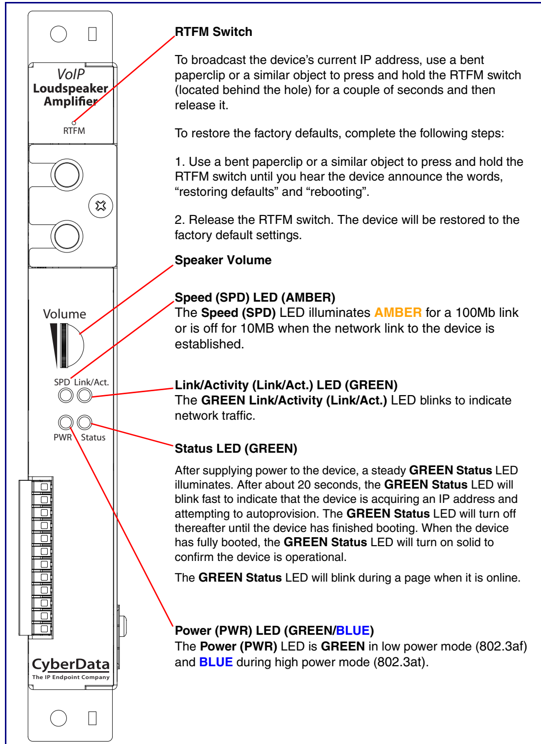
Figure 2-1. SIP Loudspeaker Amplifier (AC-Powered) Components
