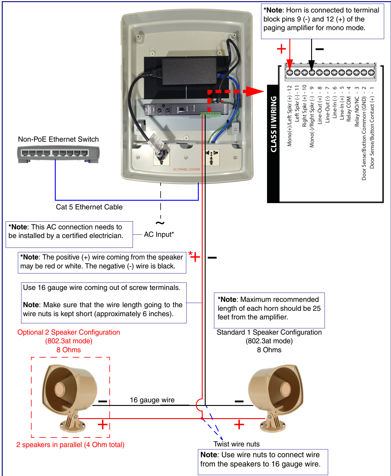
Figure 2-4. Using the Amplified Outputs—High Power Mode with Two Speakers
