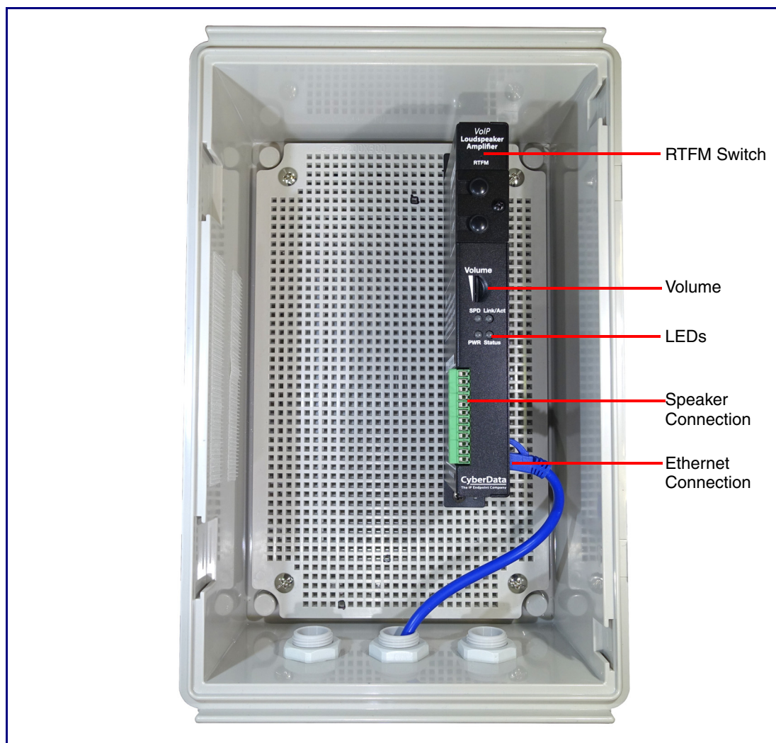
Figure 2-2. Loudspeaker Amplifier Components—PoE
