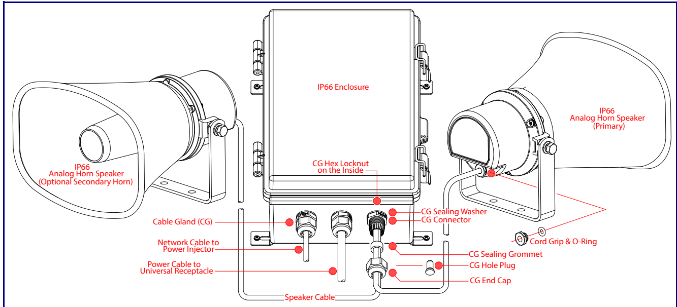
Figure 2-19. IP66 Weatherproofing
