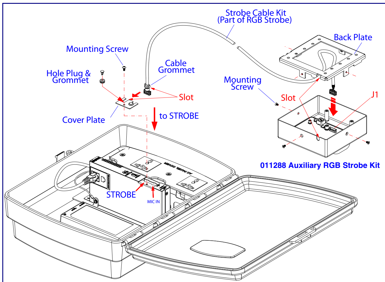
Figure 2-13. Connecting the Strobe
