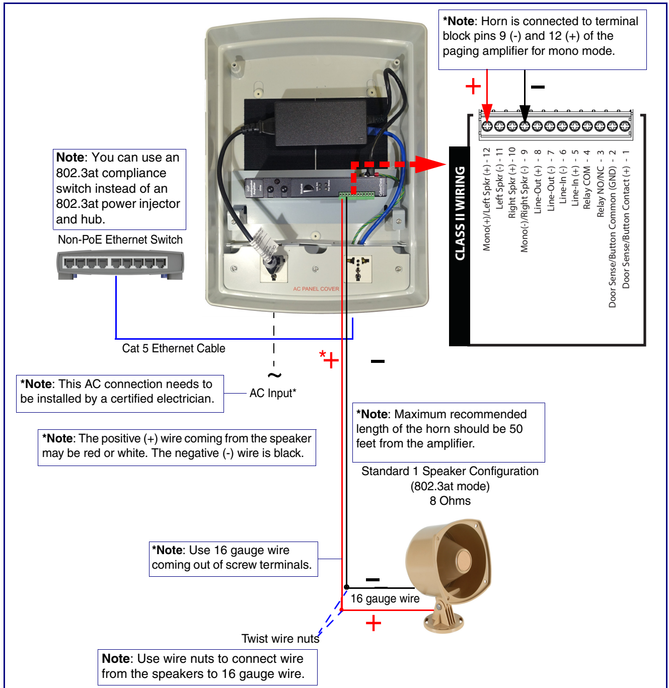
Figure 2-5. Using the Amplified Outputs—High Power Mode with One Speaker
