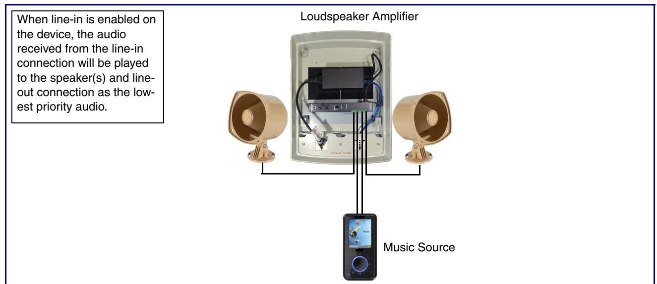
Figure 2-8. Line-In Connection
