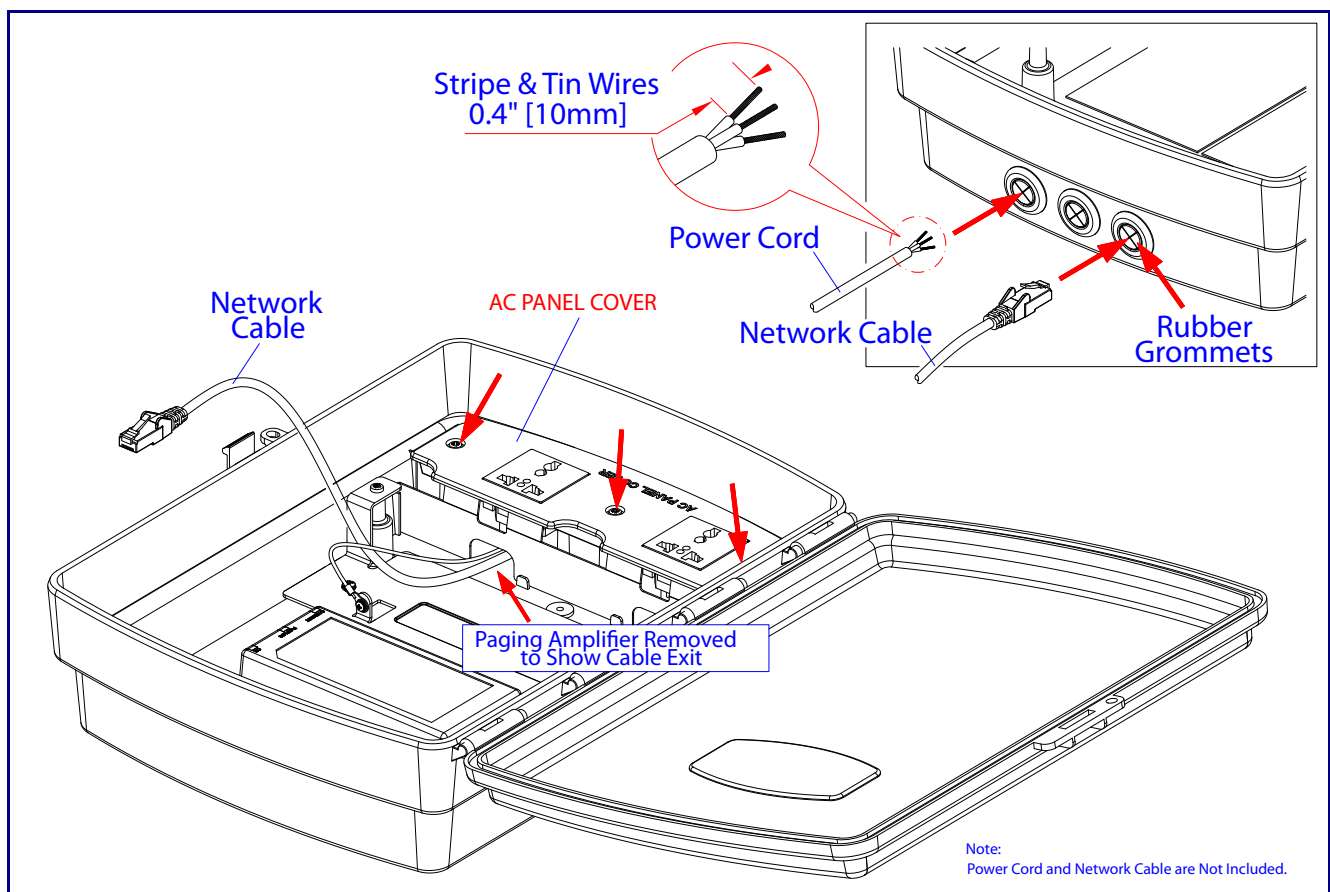
Figure 2-12. Power Cord and Network Cable Through Rubber Grommet and Prepare Power Cord Wires for Receptacle on AC Panel Cover
