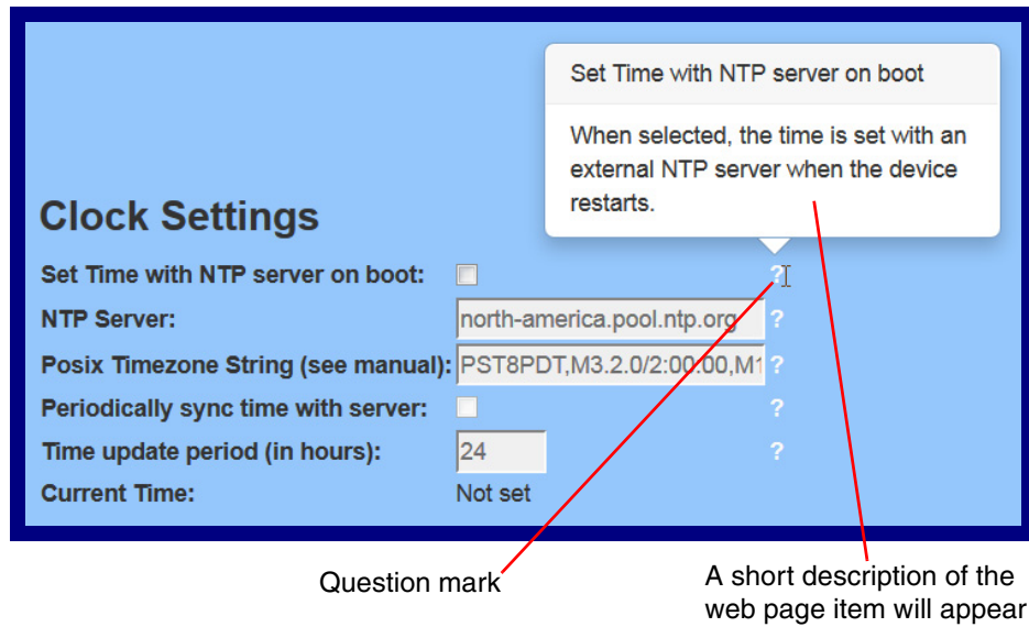
Figure 2-22. Short Description Provided by the Help Feature
