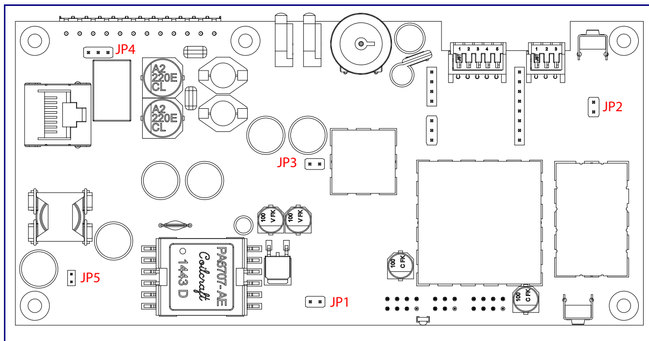
Figure 2-14. Jumper Locations
