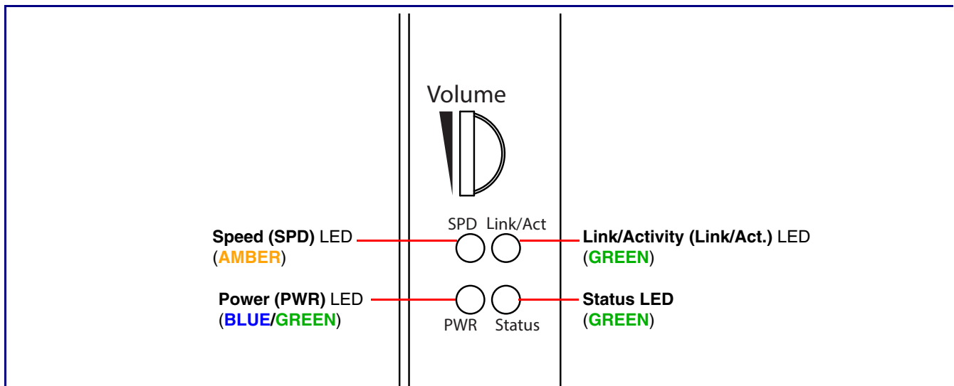
Figure 2-16. Singlewire InformaCast Loudspeaker Amplifier LEDs
