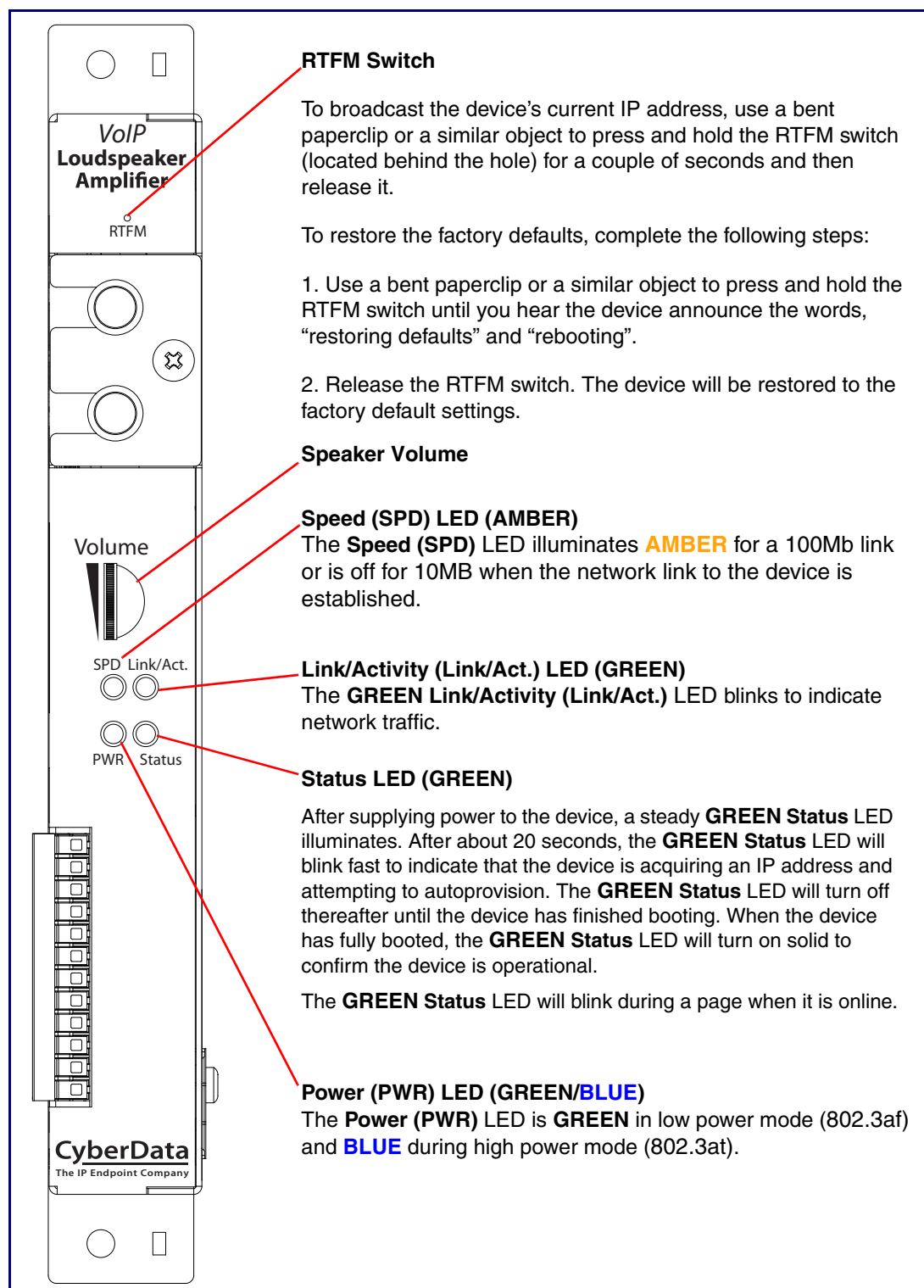
Figure 2-4. Singlewire InformaCast Loudspeaker Amplifier (PoE) Components
