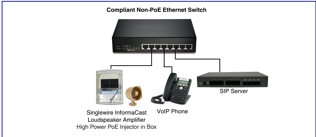
Figure 1-2. Typical Installation
