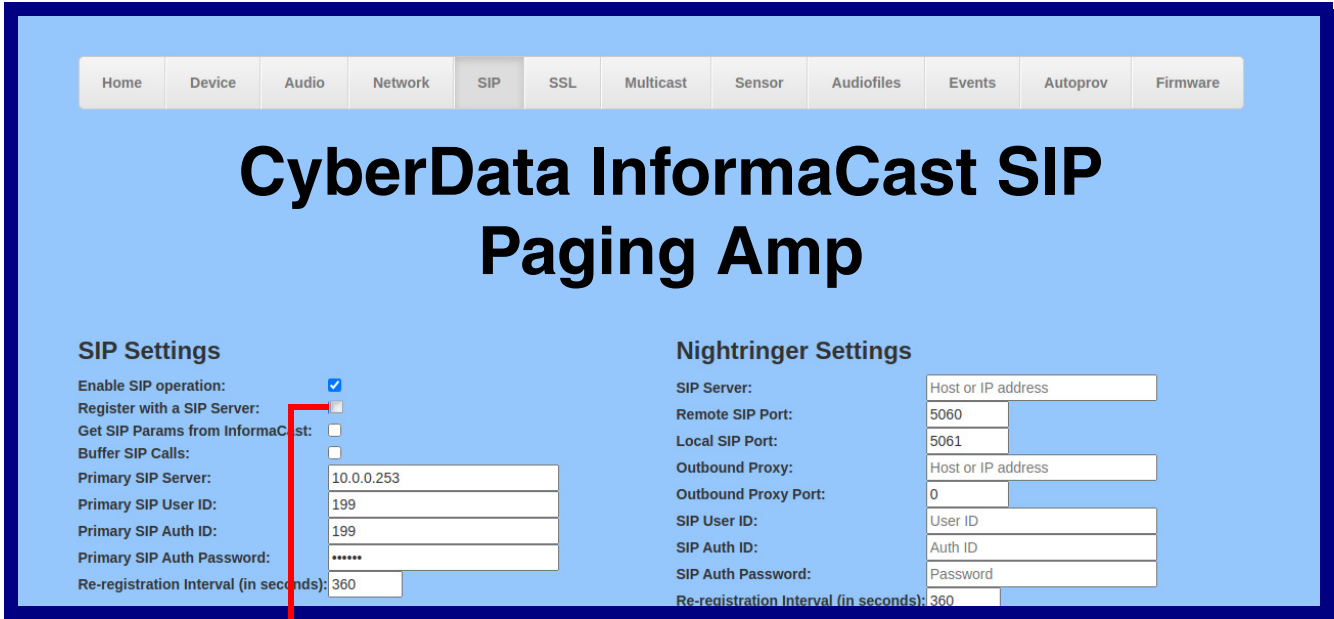
Figure 2-31. SIP Page Set to Point-to-Point Mode
