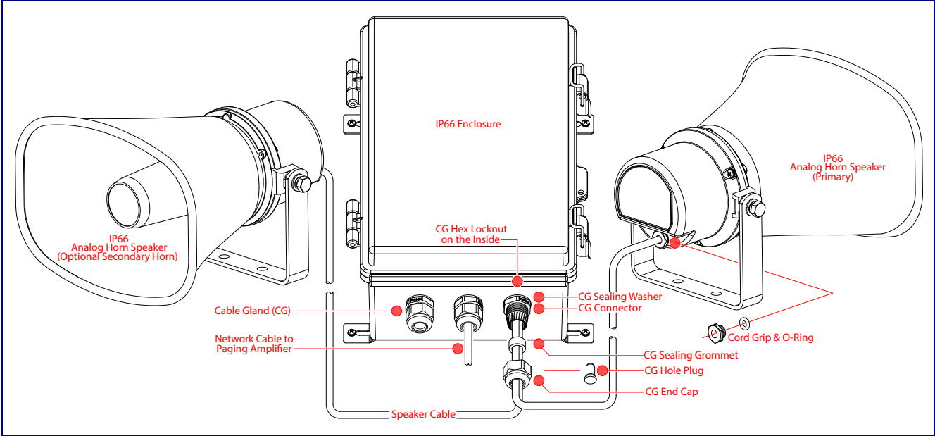
Figure 2-18. IP66 Weatherproofing
