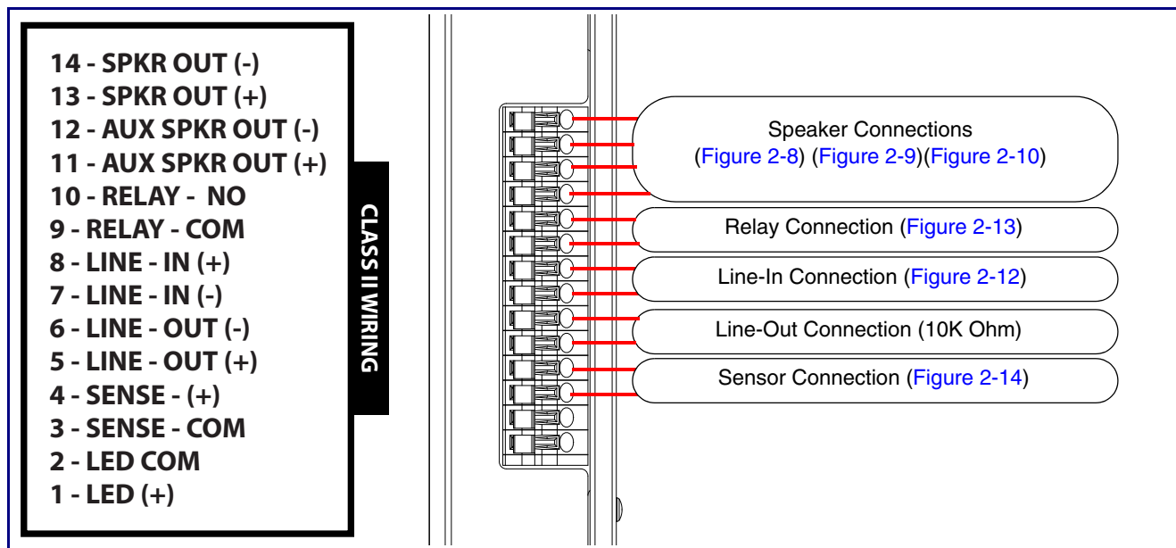
Figure 2-11. InformaCast Enabled Loudspeaker Amplifier (PoE) Connections
