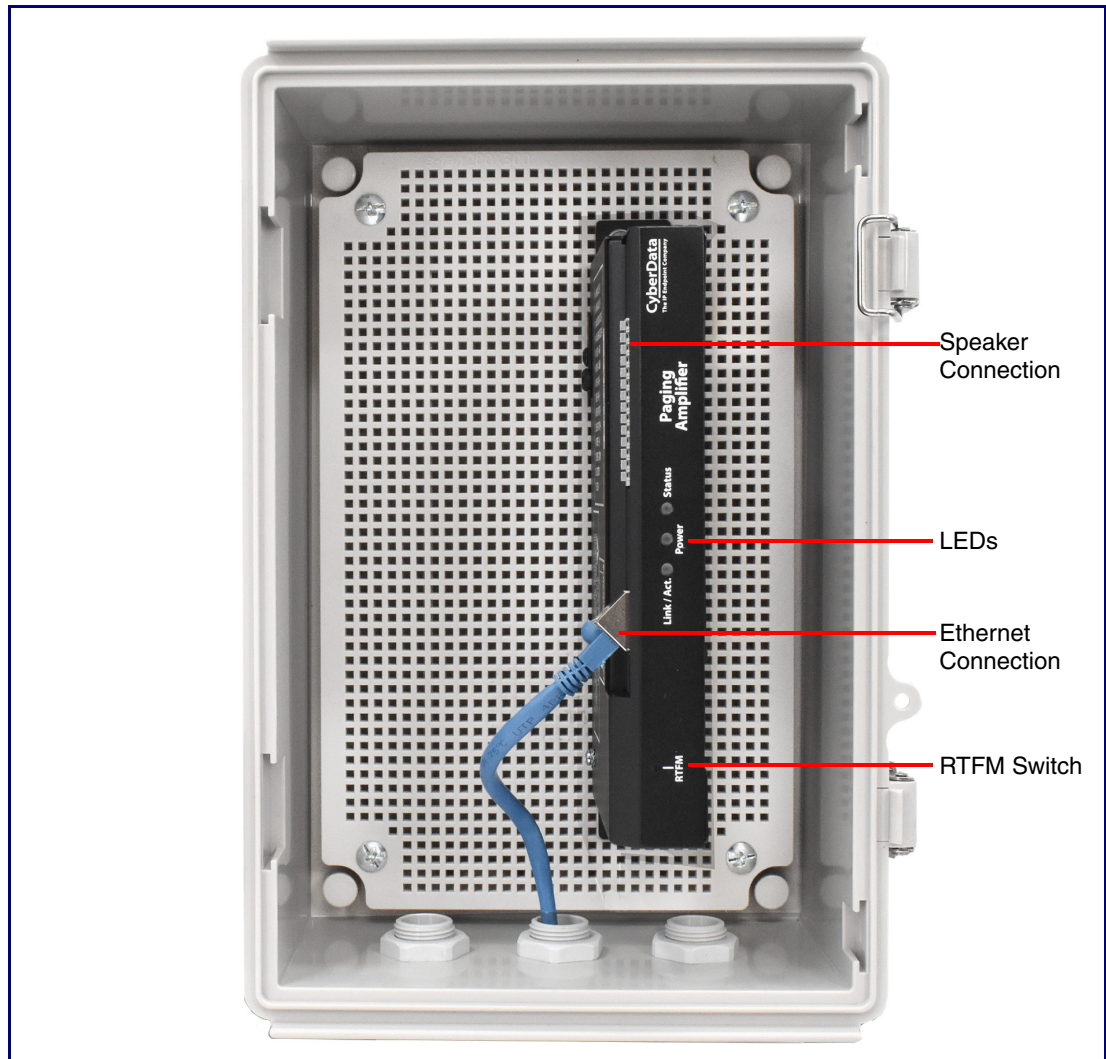
Figure 2-6. Loudspeaker Amplifier Components—PoE
