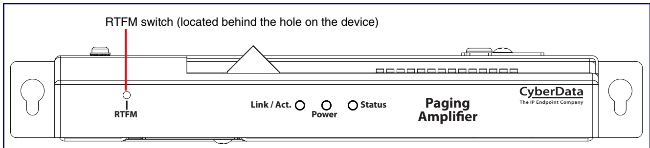
Figure 2-21. RTFM Switch
