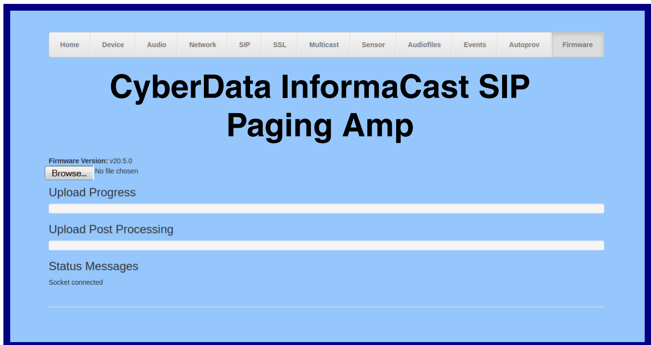
Figure 2-46. Firmware Page
