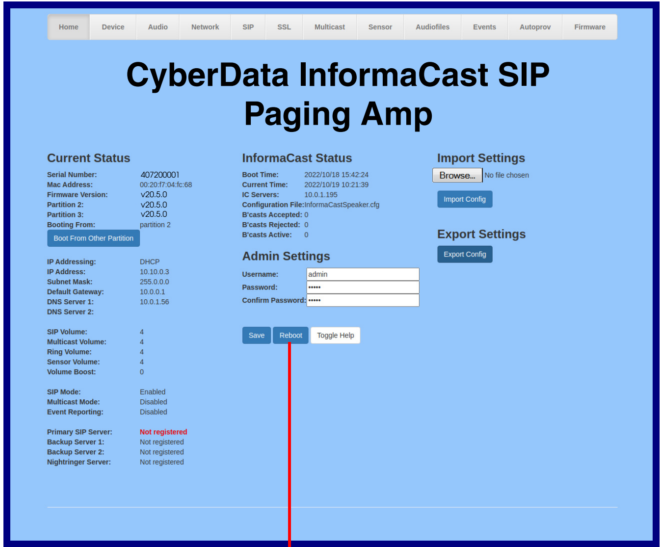
Figure 2-48. Home Page
