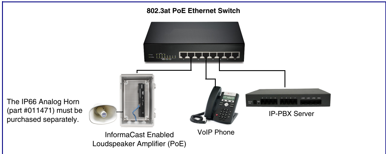
Figure 1-2. Typical Installation
