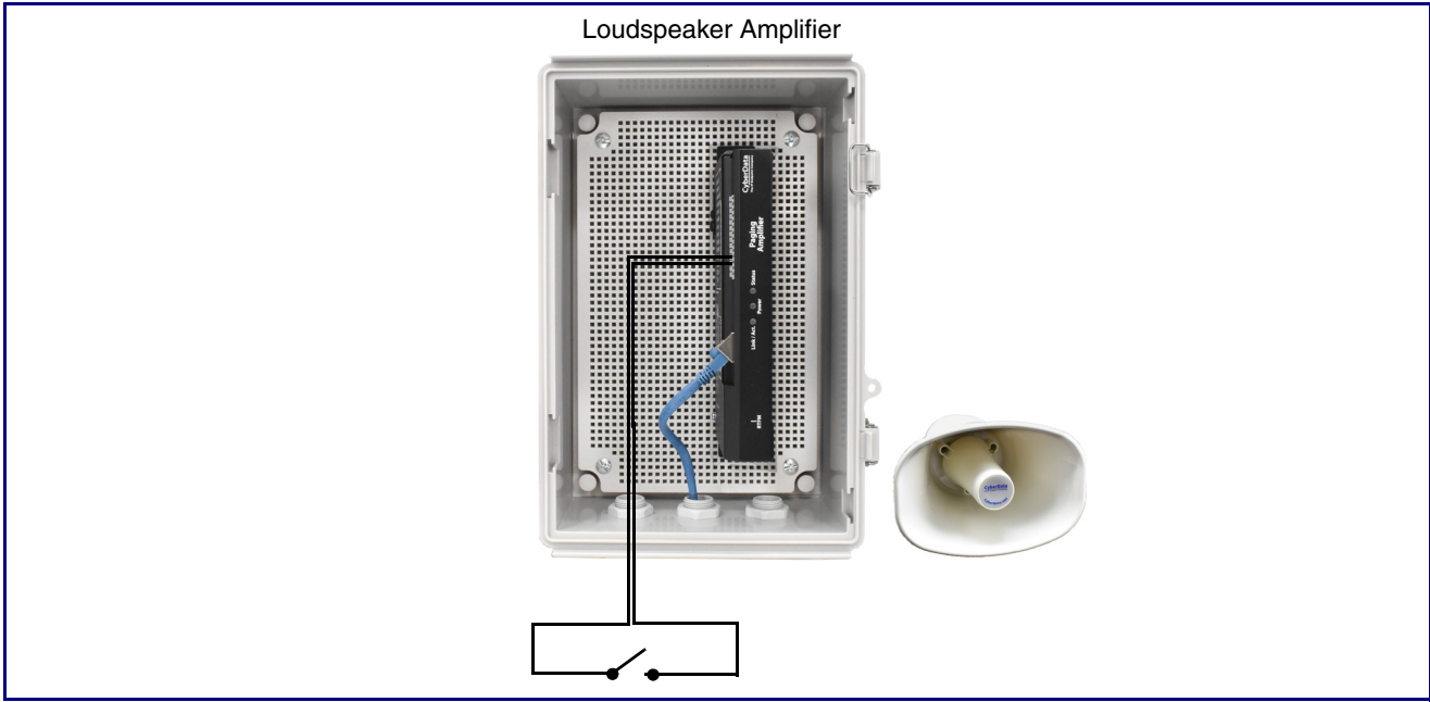
Figure 2-14. Sensor Connection
