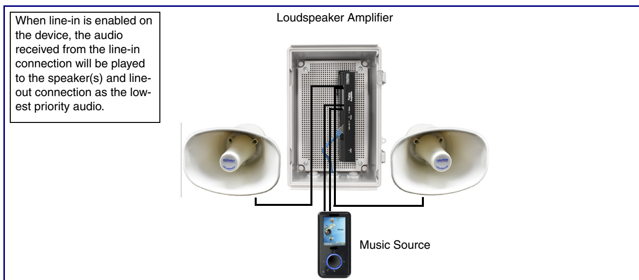
Figure 2-12. Line-In Connection
