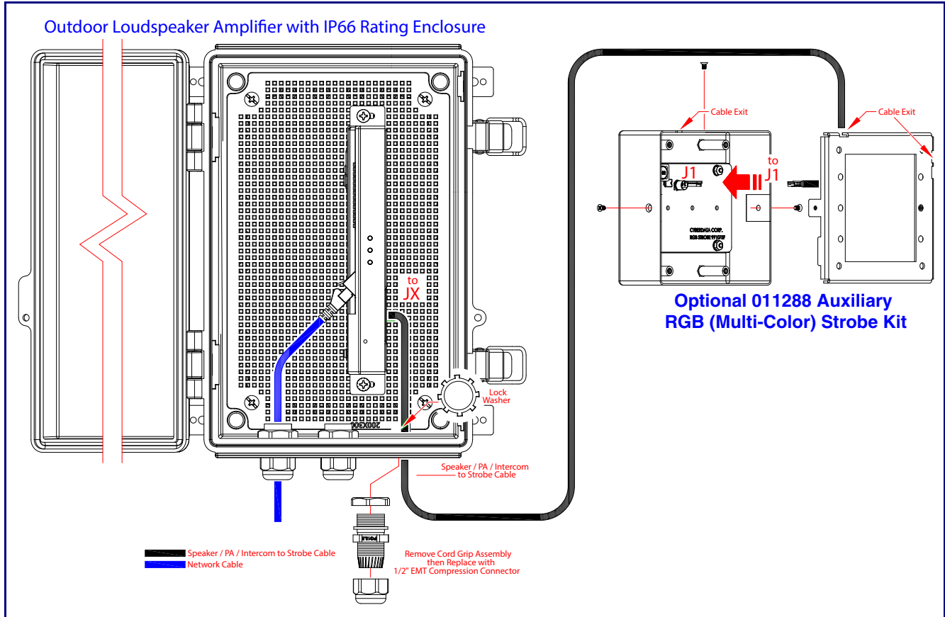
Figure 2-16. Connecting the 011288 Auxiliary RGB (Multi-Color) Strobe Kit
