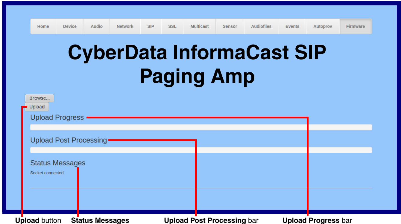
Figure 2-47. Upload Button
