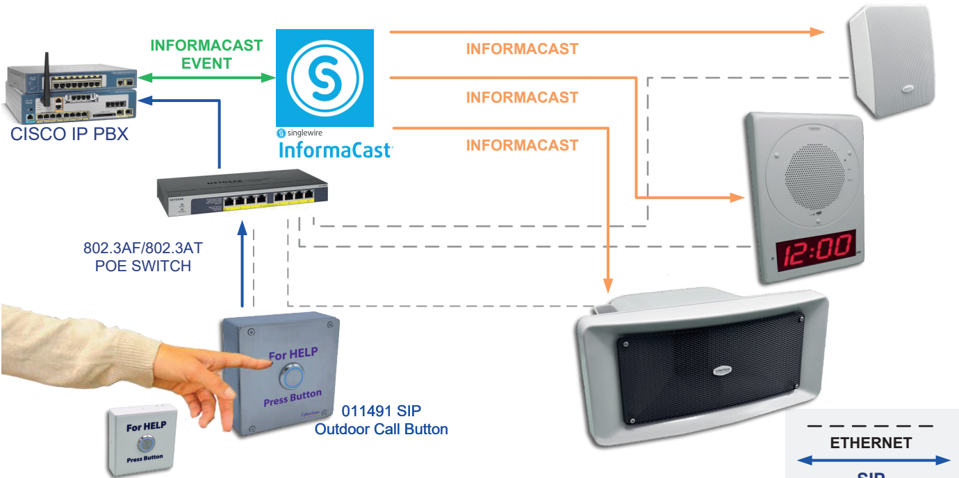
011049 SIP Call Button
