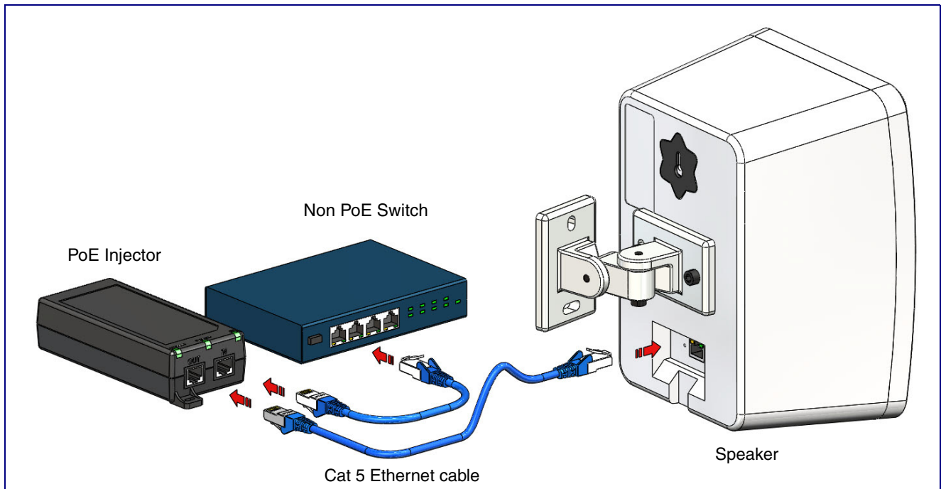
Figure 2-2. VoIP SIP/Multicast Wall Mount Speaker (with PoE Injector) to a Non PoE Switch
