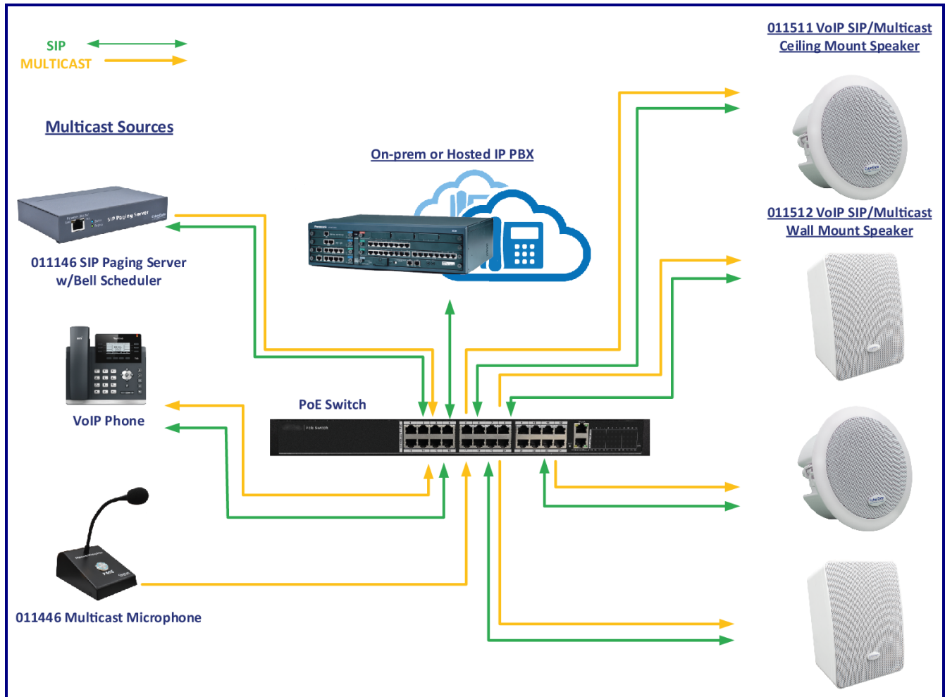
Figure 1-2. Typical IP Speaker Configuration
