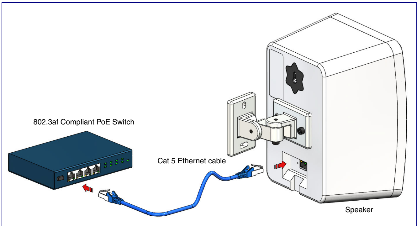
Figure 2-1. VoIP SIP/Multicast Wall Mount Speaker to a 802.3af Compliant PoE Switch
